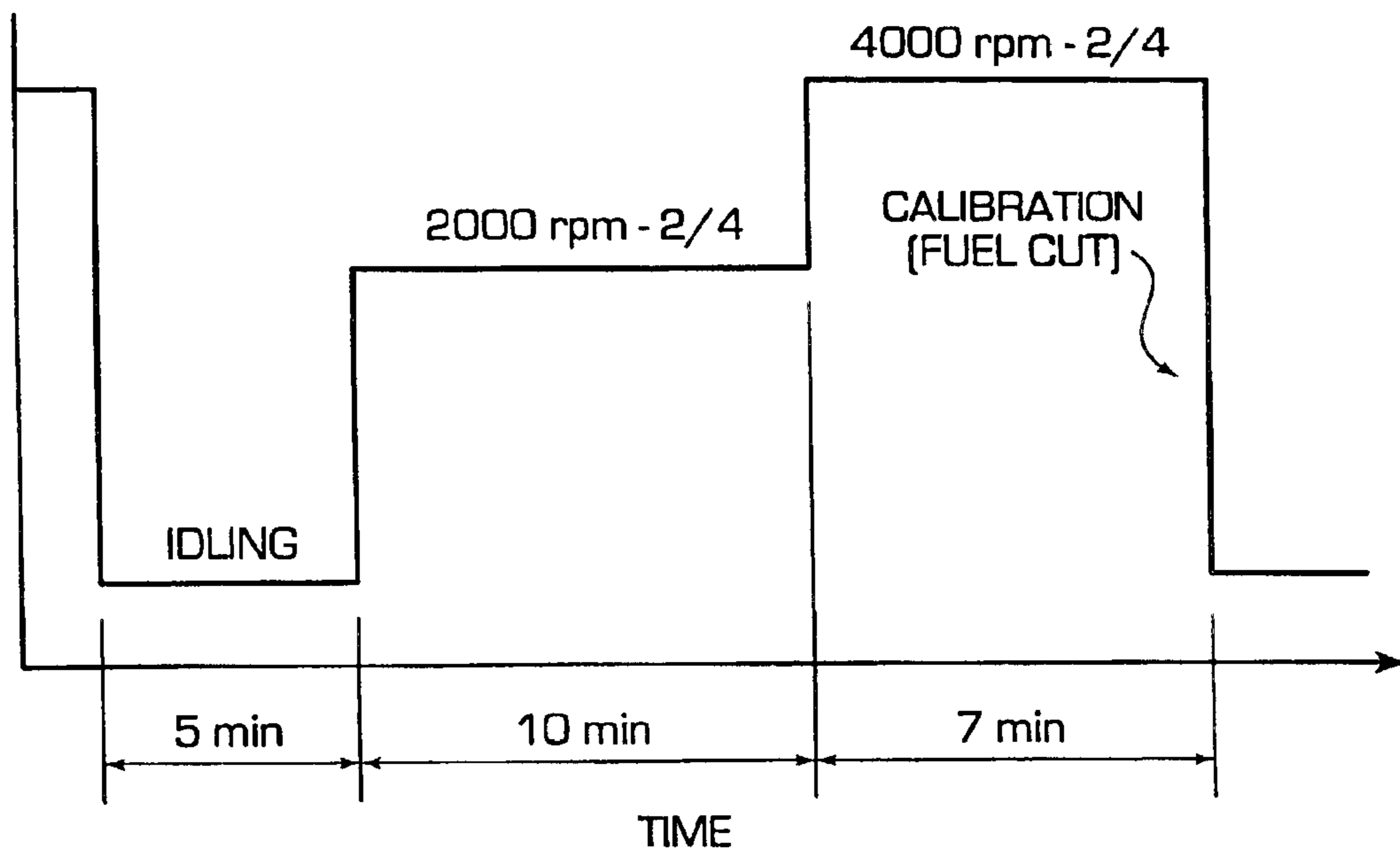
FIG. 18 DURABILITY TEST MODE
