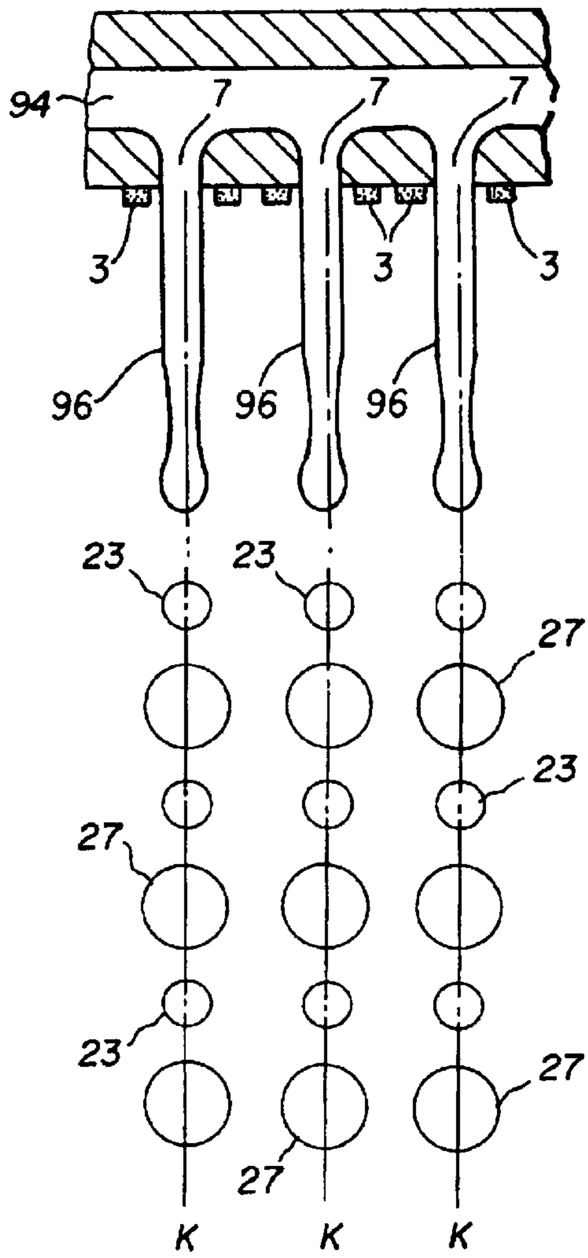
FIG. 4 (PRIOR ART)
