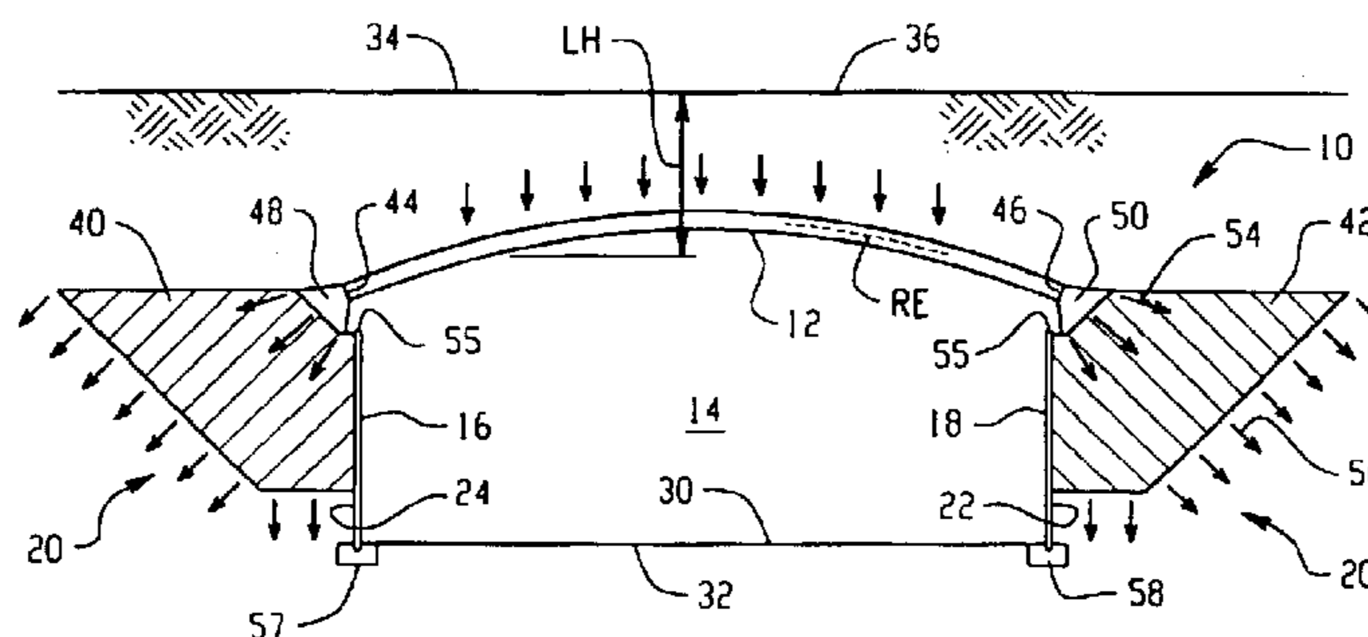
DIRECT TRANSFER OF THE ARCH THRUST THROUGH THE SOLIDIFIED BACKFILL MATERIAL (FOUNDATION BLOCKS) INTO THE SUBSOIL. THE FOUNDATION BLOCKS REDUCE THE LOADS IN THE SUBSOIL SUCH THAT THE OUTWARD DISPLACEMENTS OF THE ARCH SPRINGS REMAIN VERY LIMITED.
