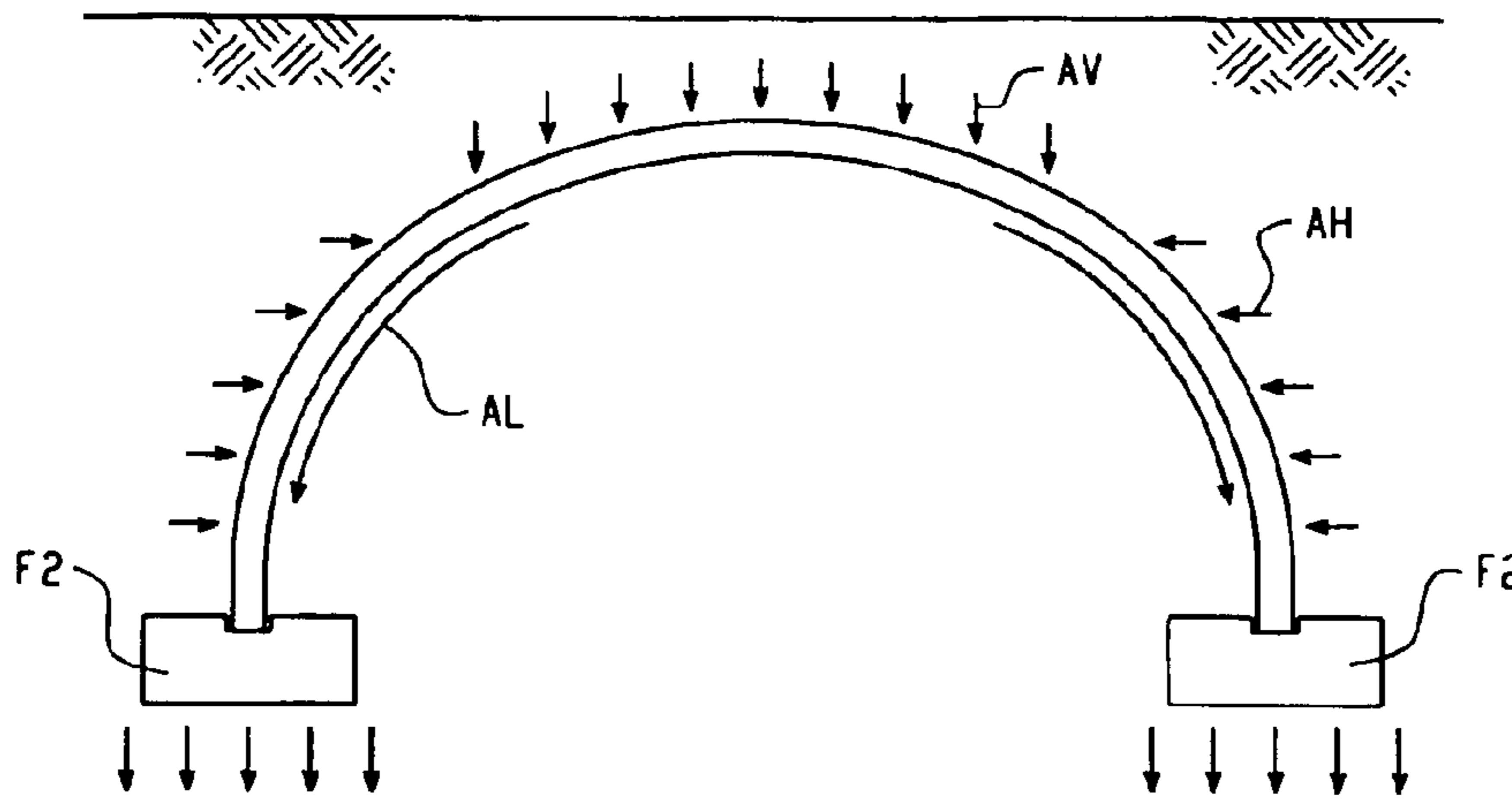
TRANSFER OF LOADS THROUGH THE SIDES TO FOOTINGS AT THE BASE OF THE BACKFILLED/OVERFILLED STRUCTURE
