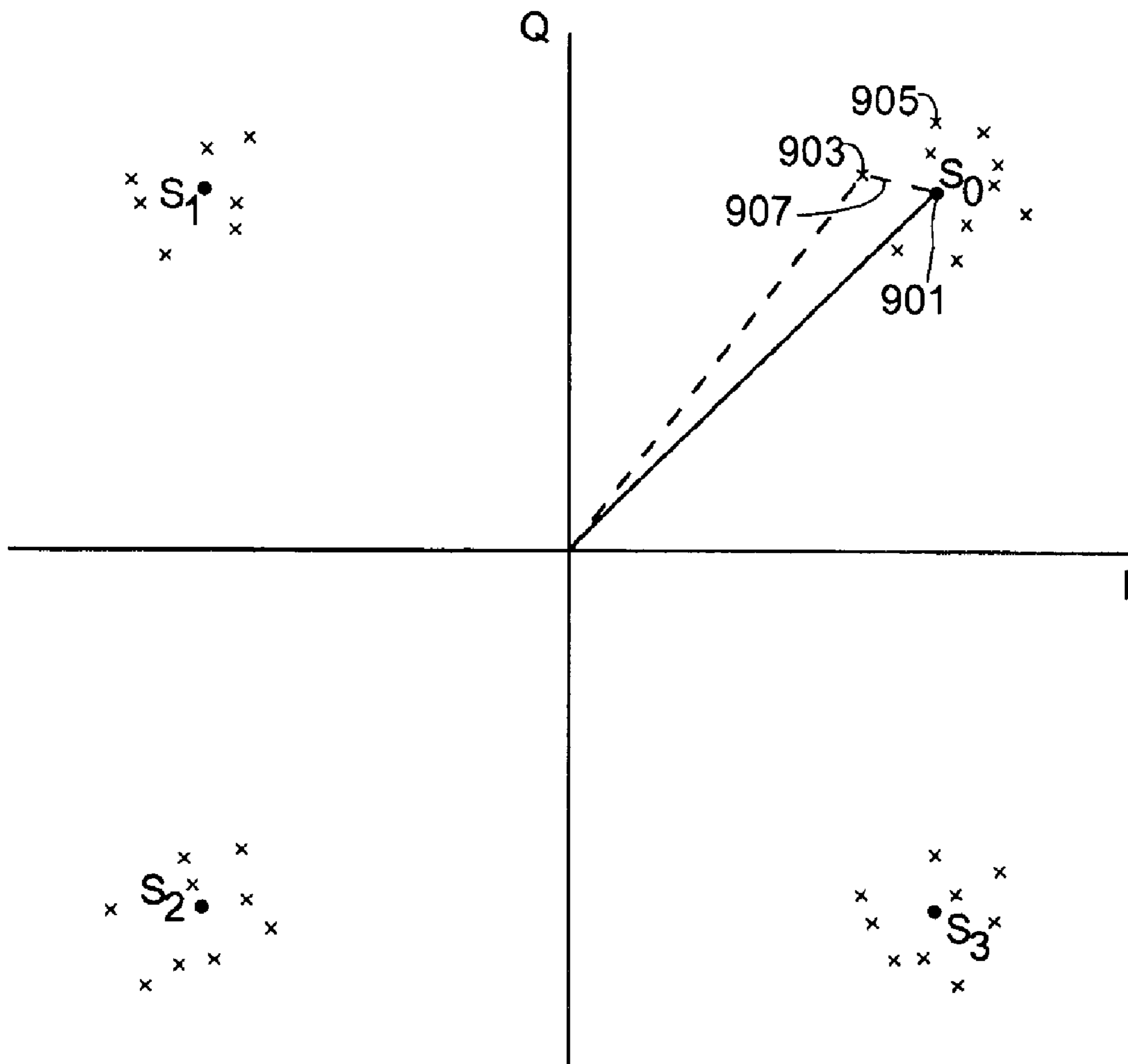
FIG. 9 (Prior Art)
