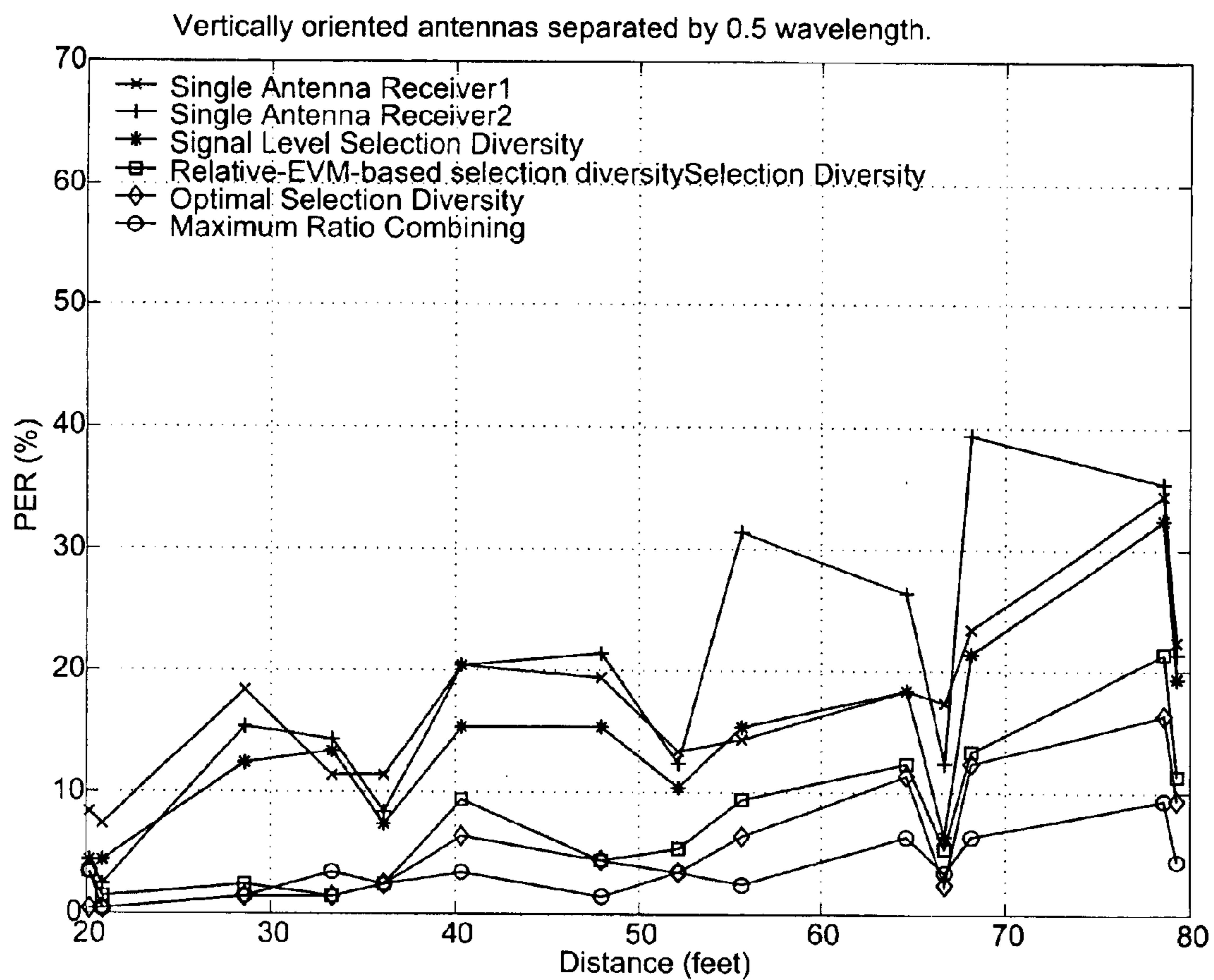
FIG. 12 (Prior Art)
