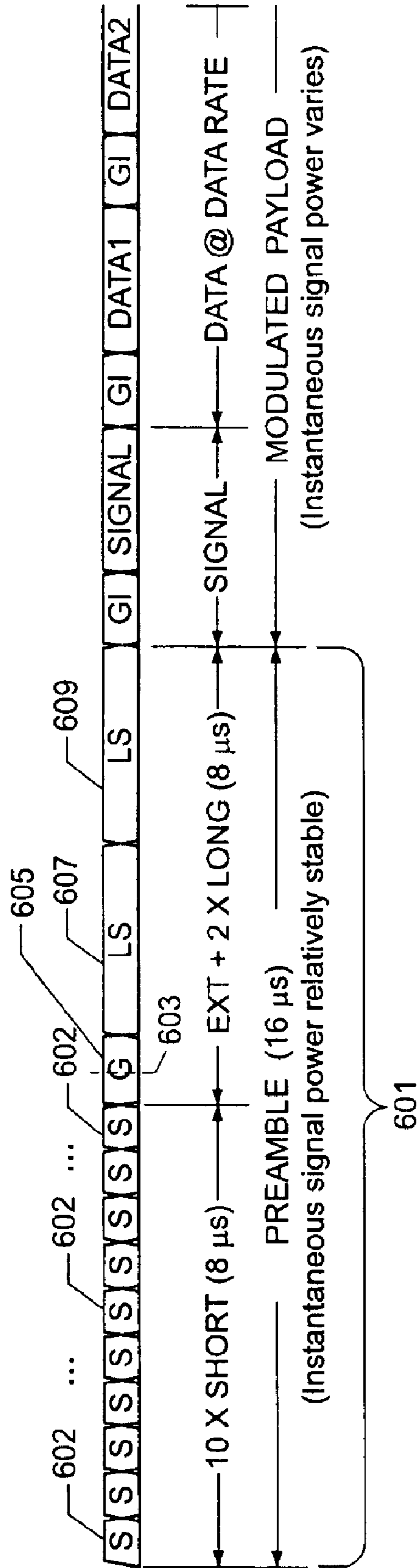
FIG. 6 (PRIOR ART)
