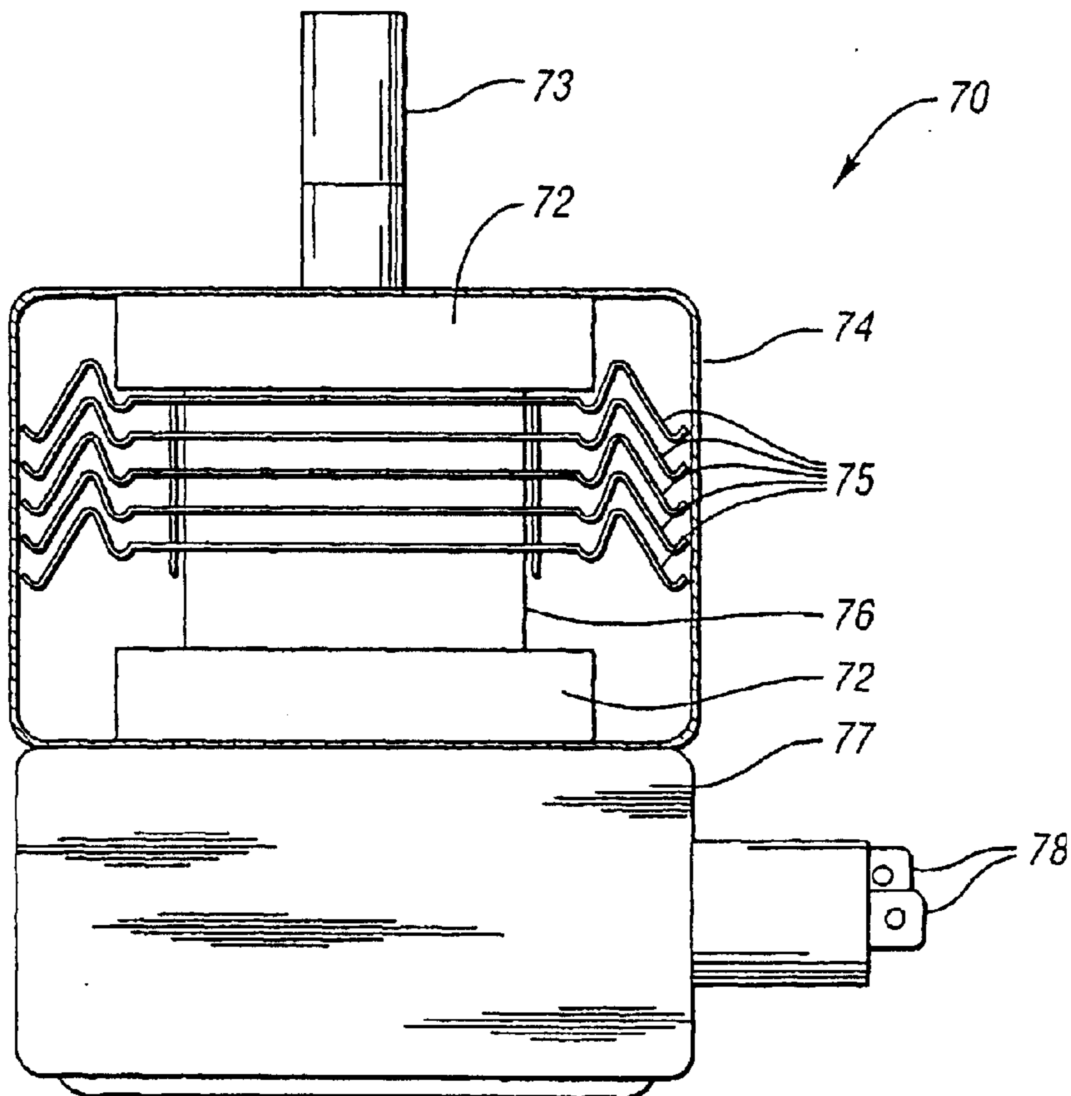
Fig. 7 (PRIOR ART)
