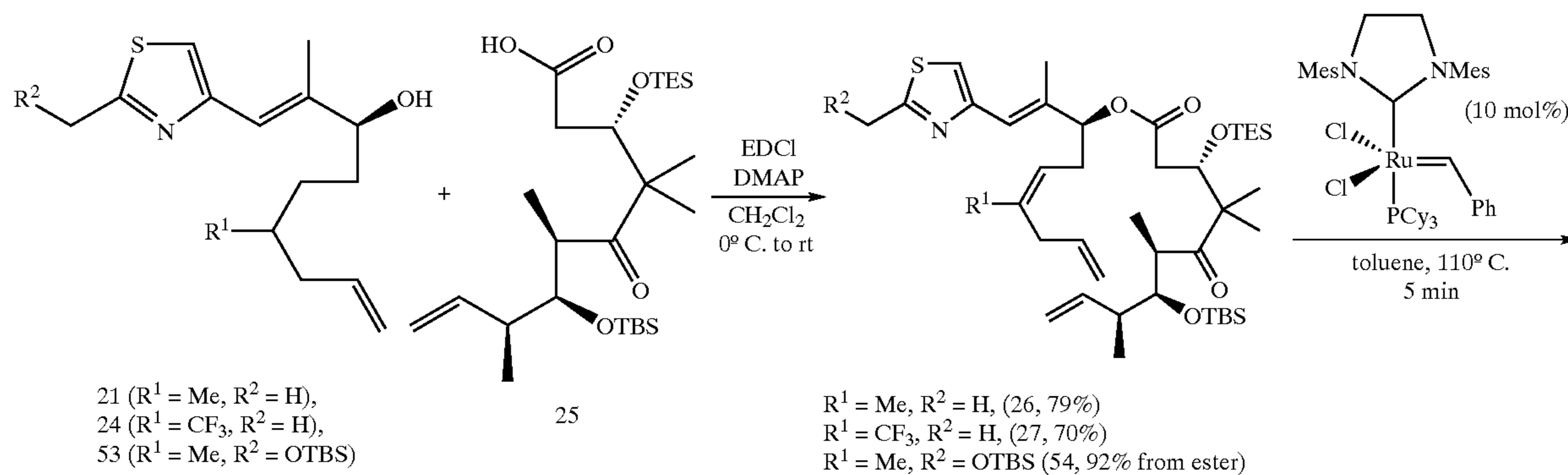
Scheme 7.
