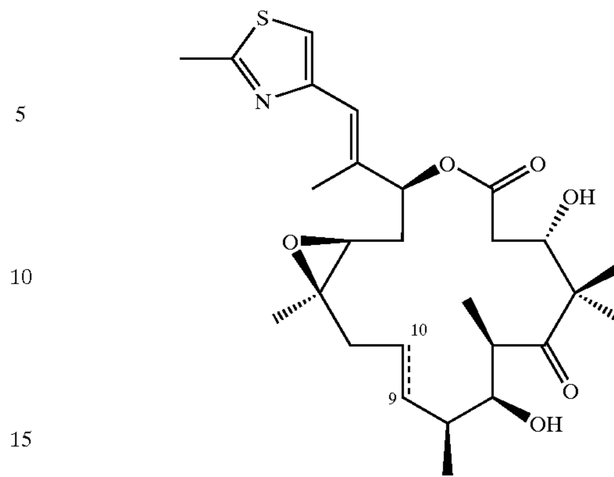
EpoB (51) (E)-9,10-dehydroEpoB (49)
