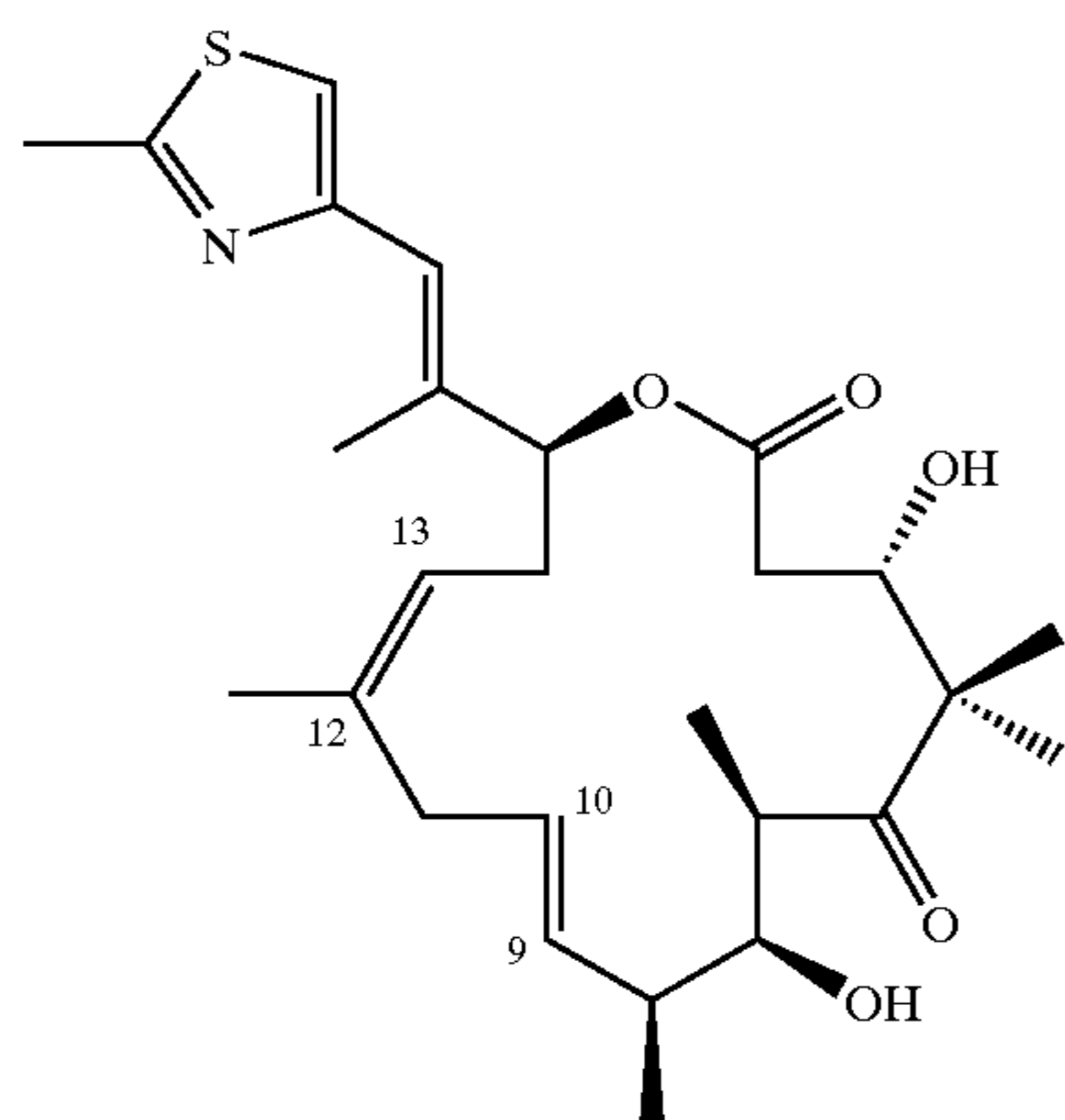
(E)-9,10-dehydro-dEpoB (28)
