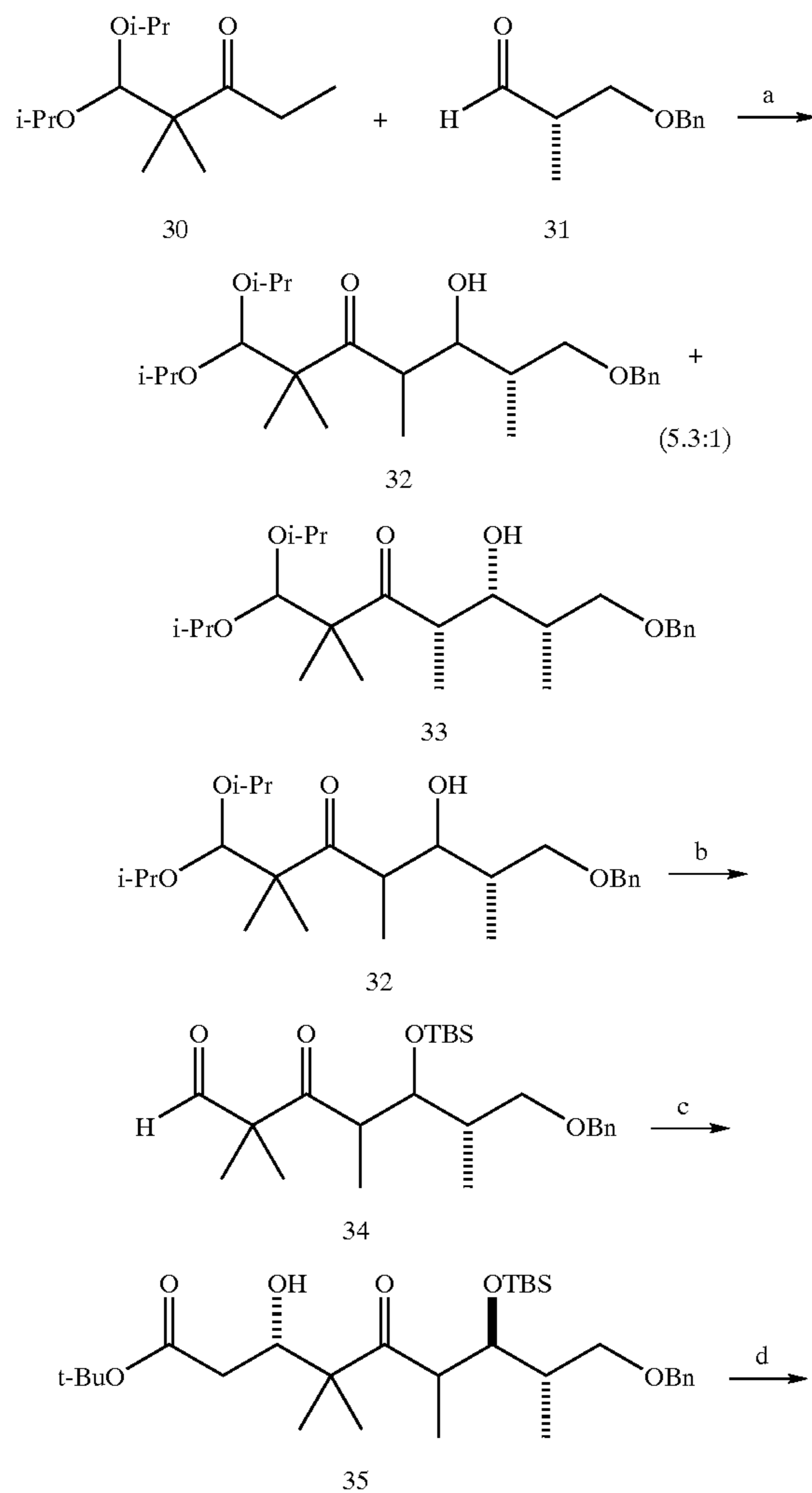
Scheme 6.
