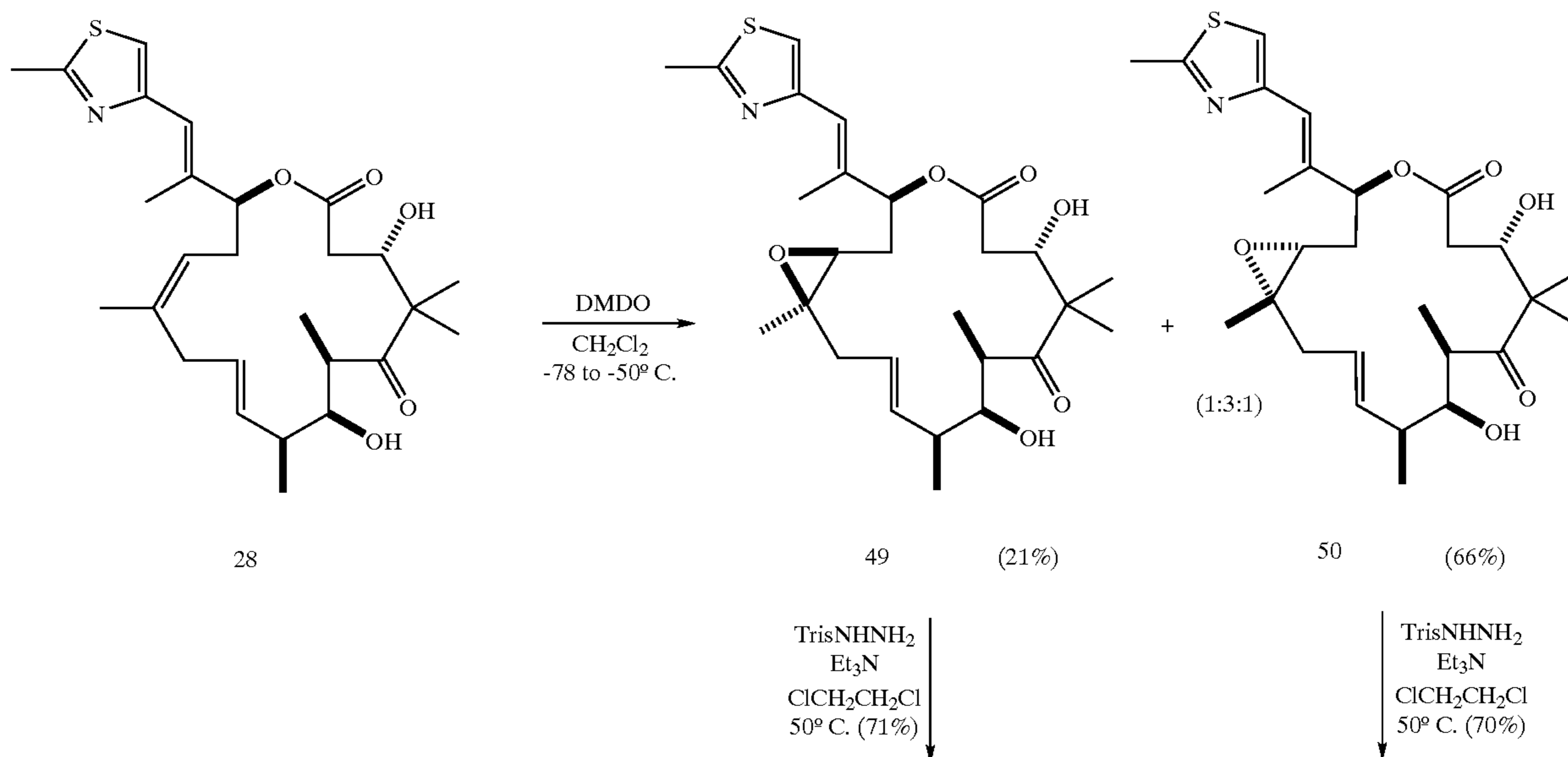
Scheme 9
