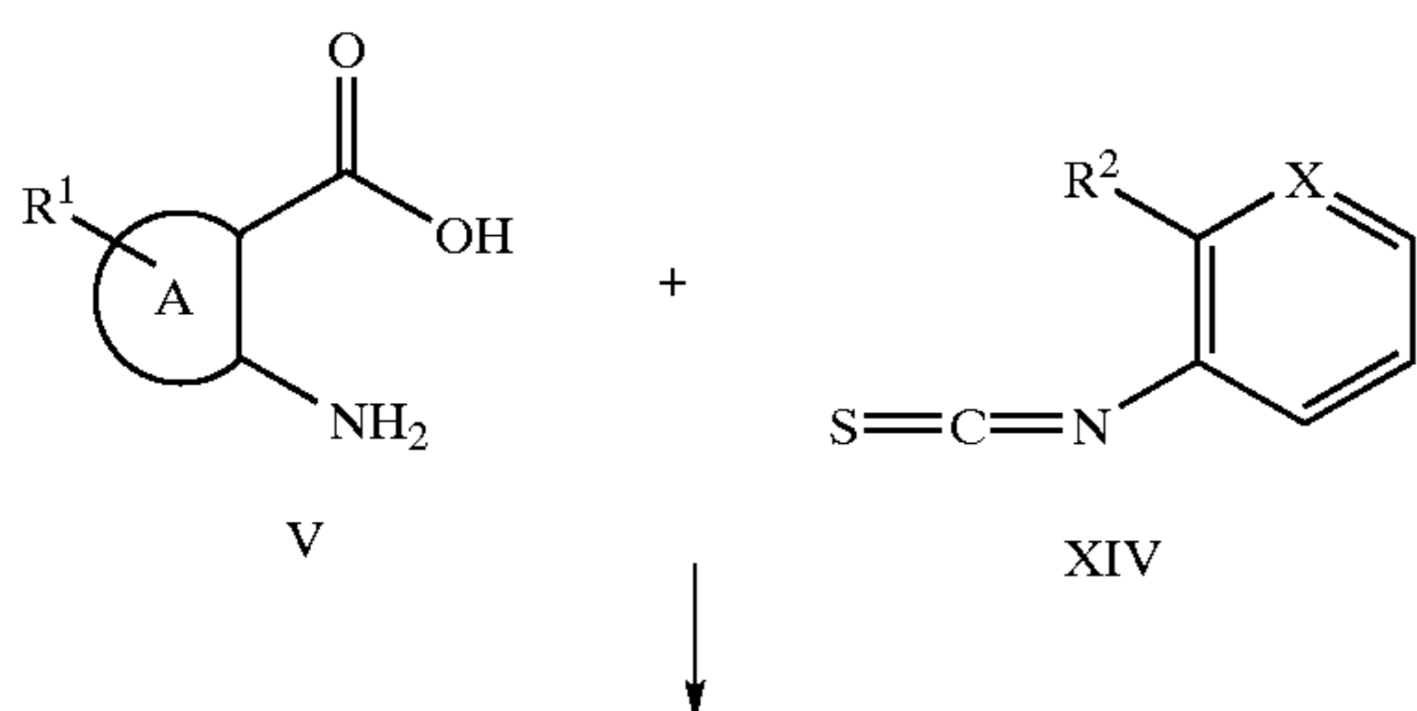
Scheme 5
