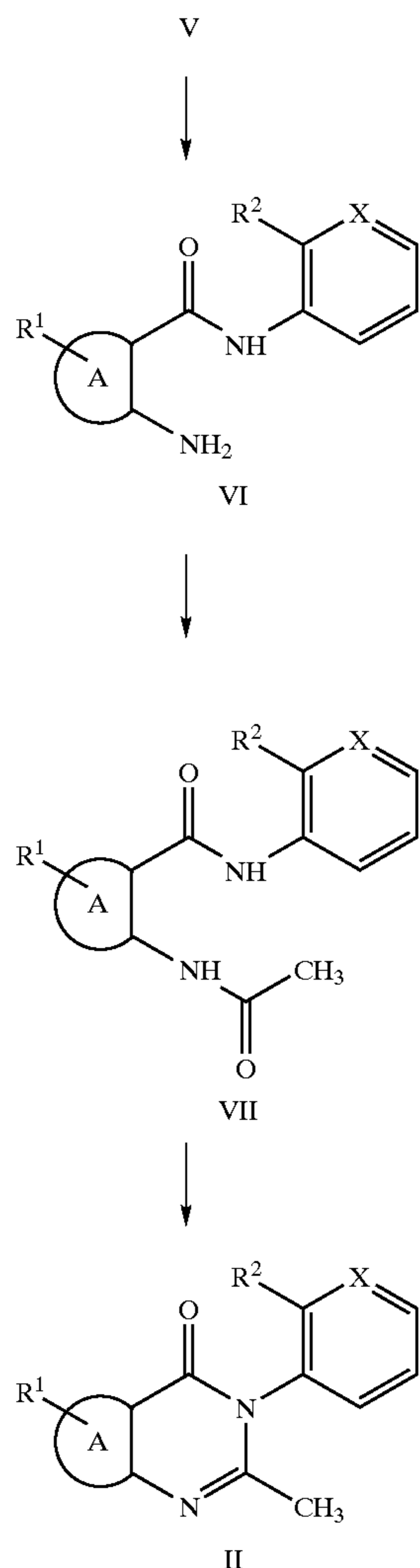
Scheme 4
