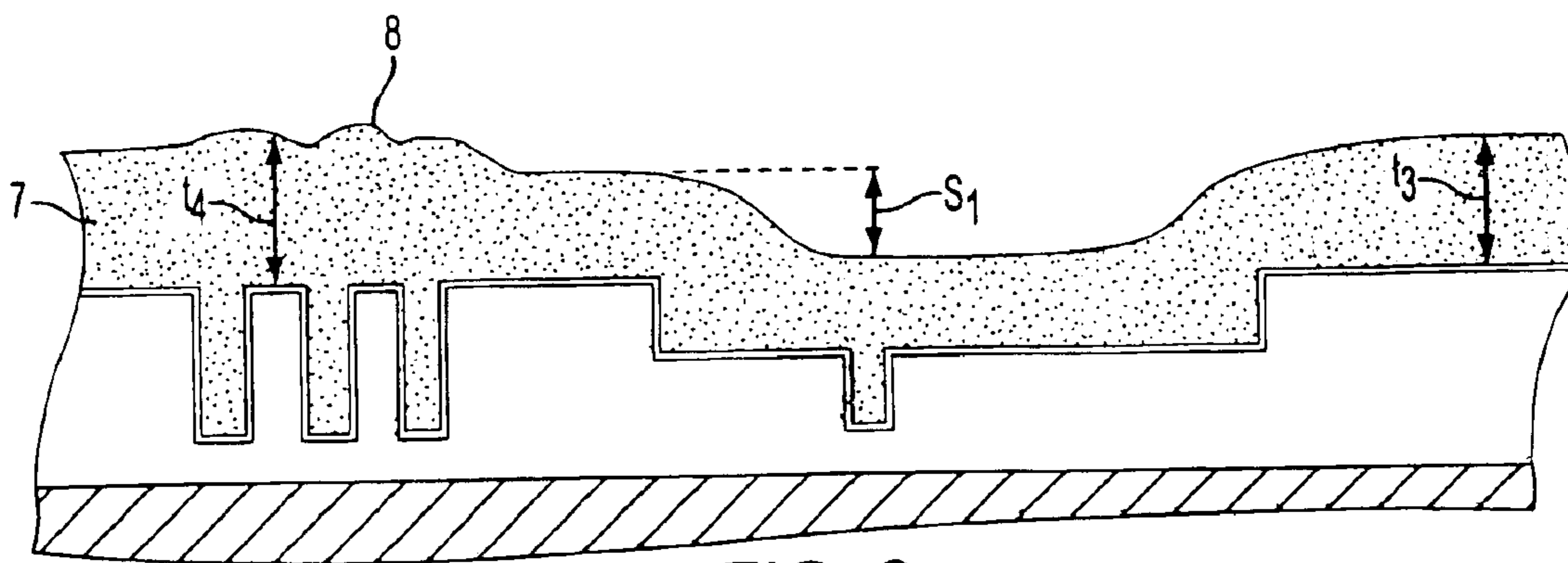
FIG. 2c (PRIOR ART)
