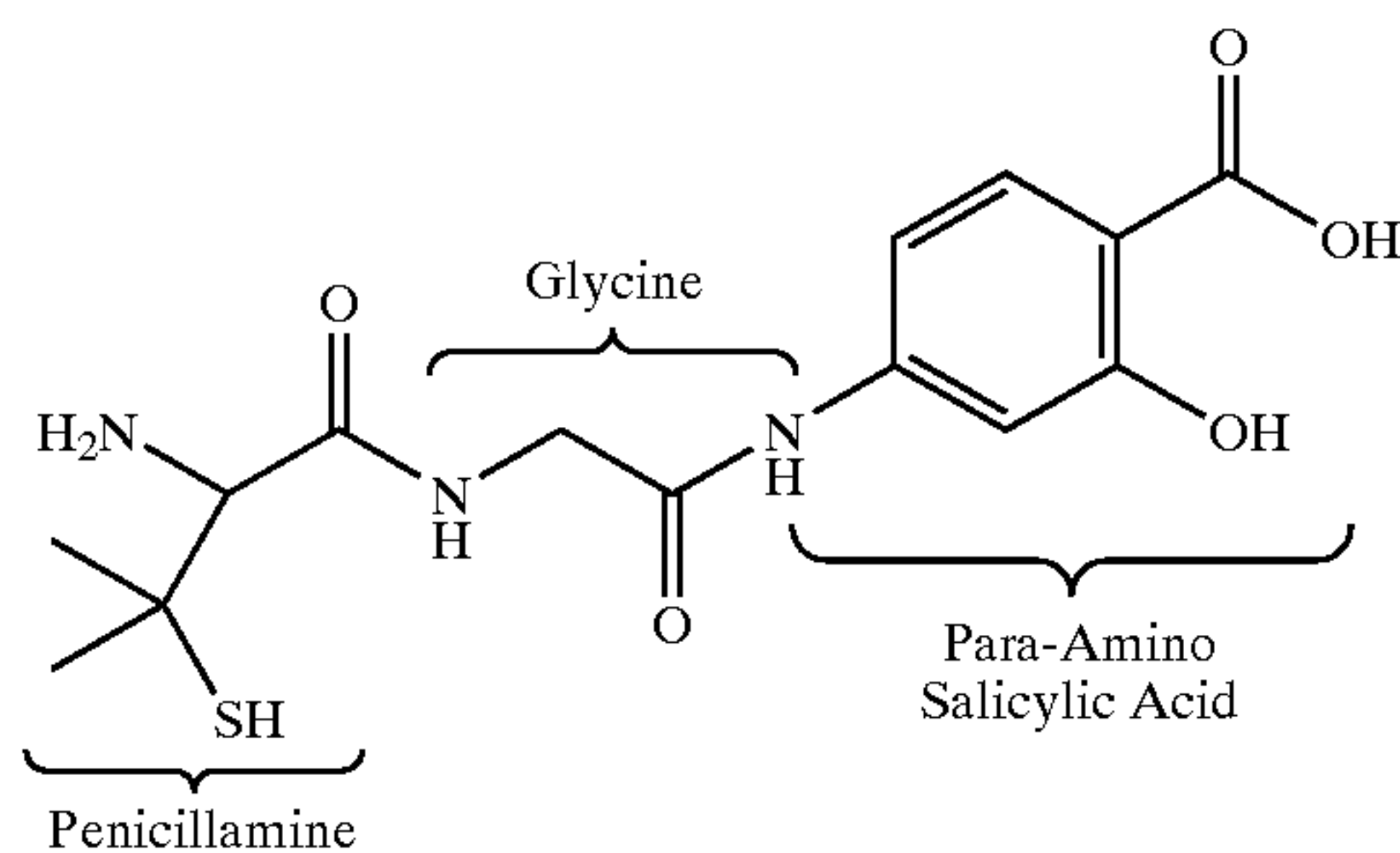
Structure of Heterodimeric Compound 1
