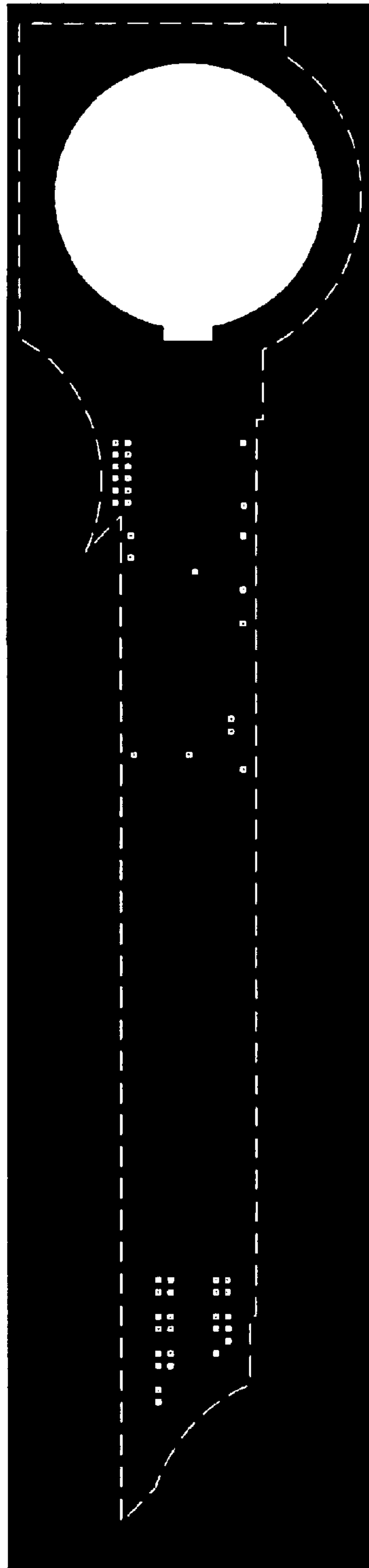
Via 1 mask
