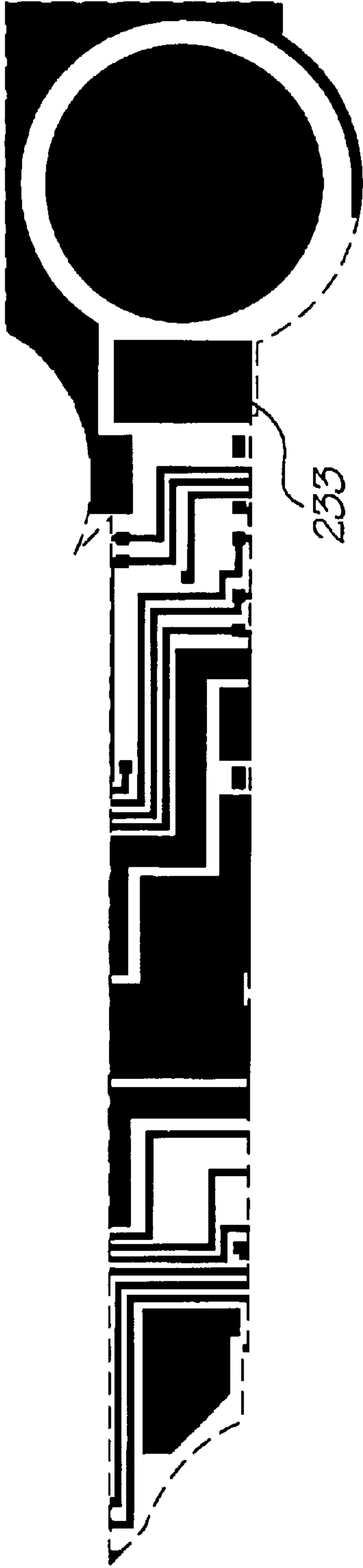
Metal 2 mask
