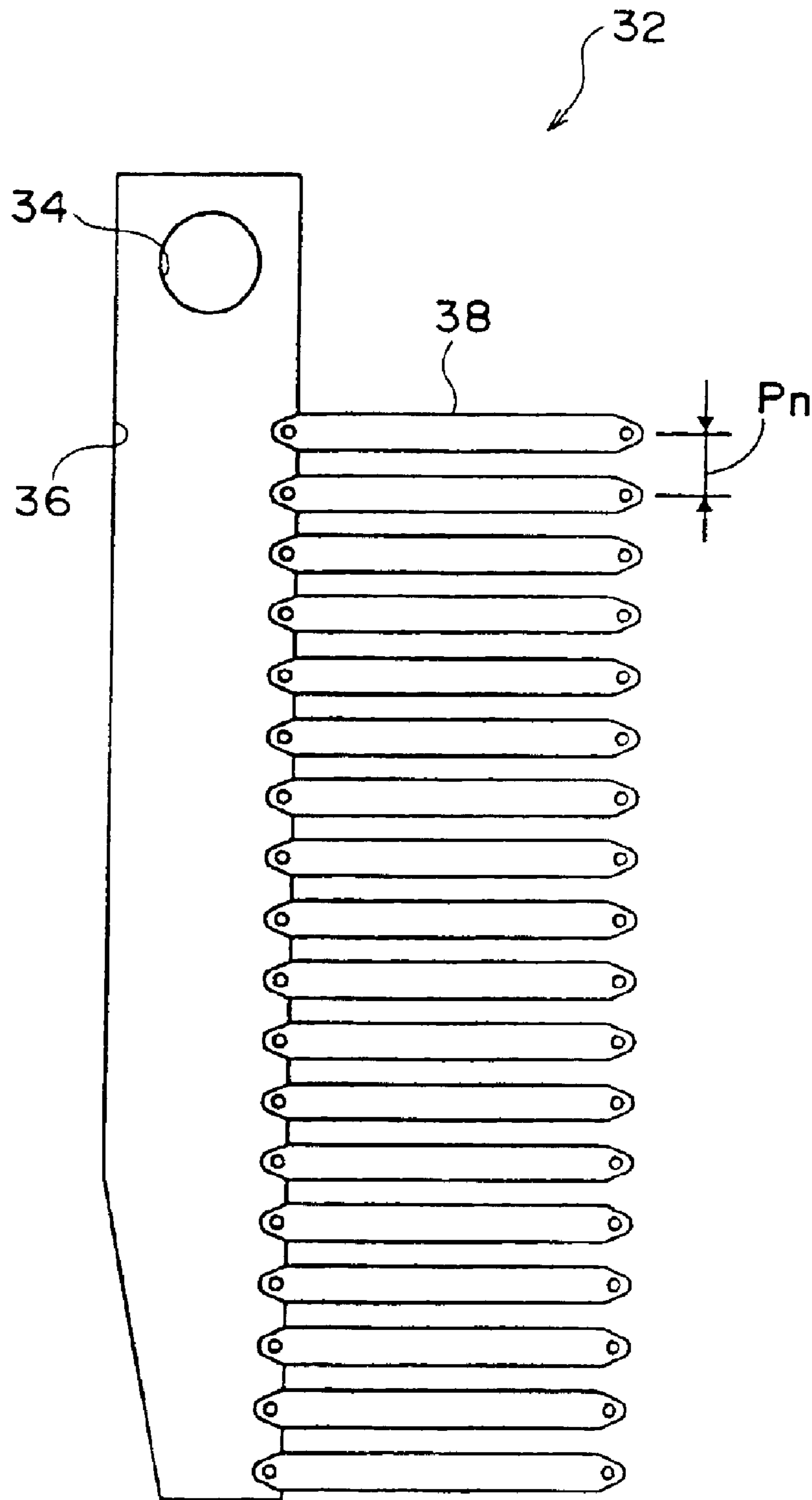
FIG. 14 PRIOR ART
