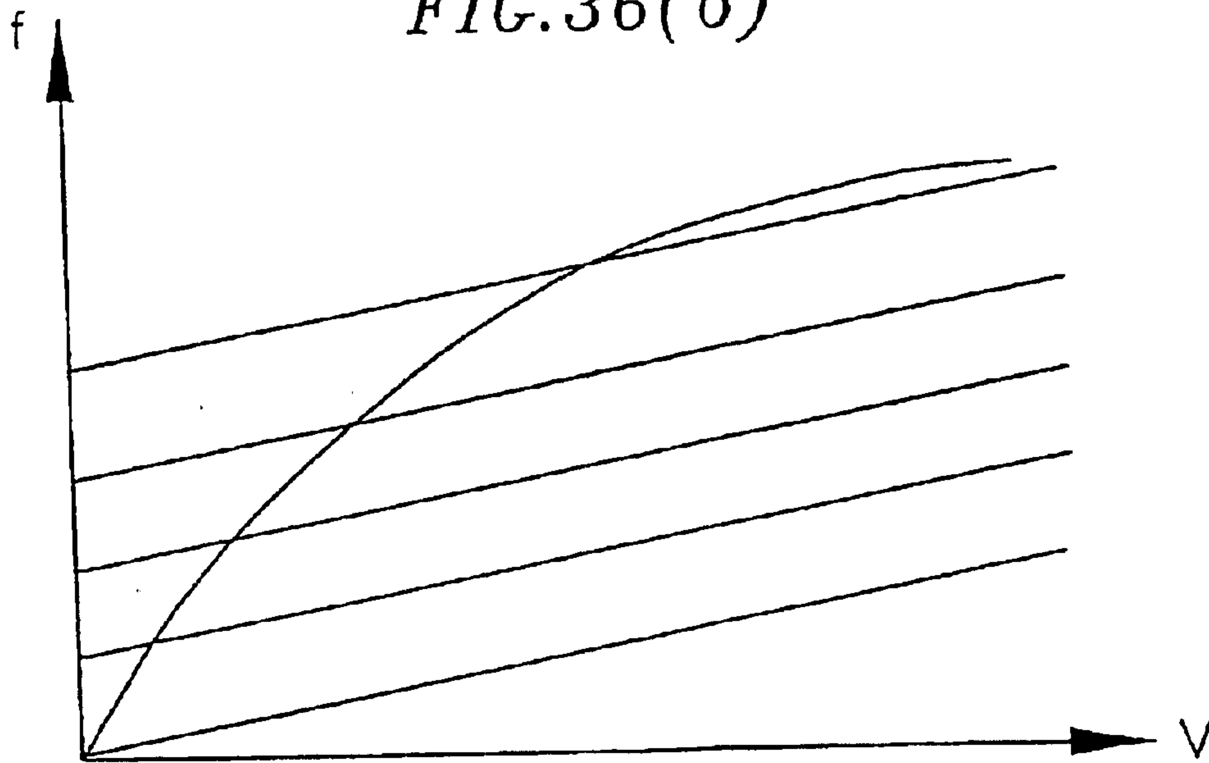
SEGMENTED VCO TUNING CURVE
