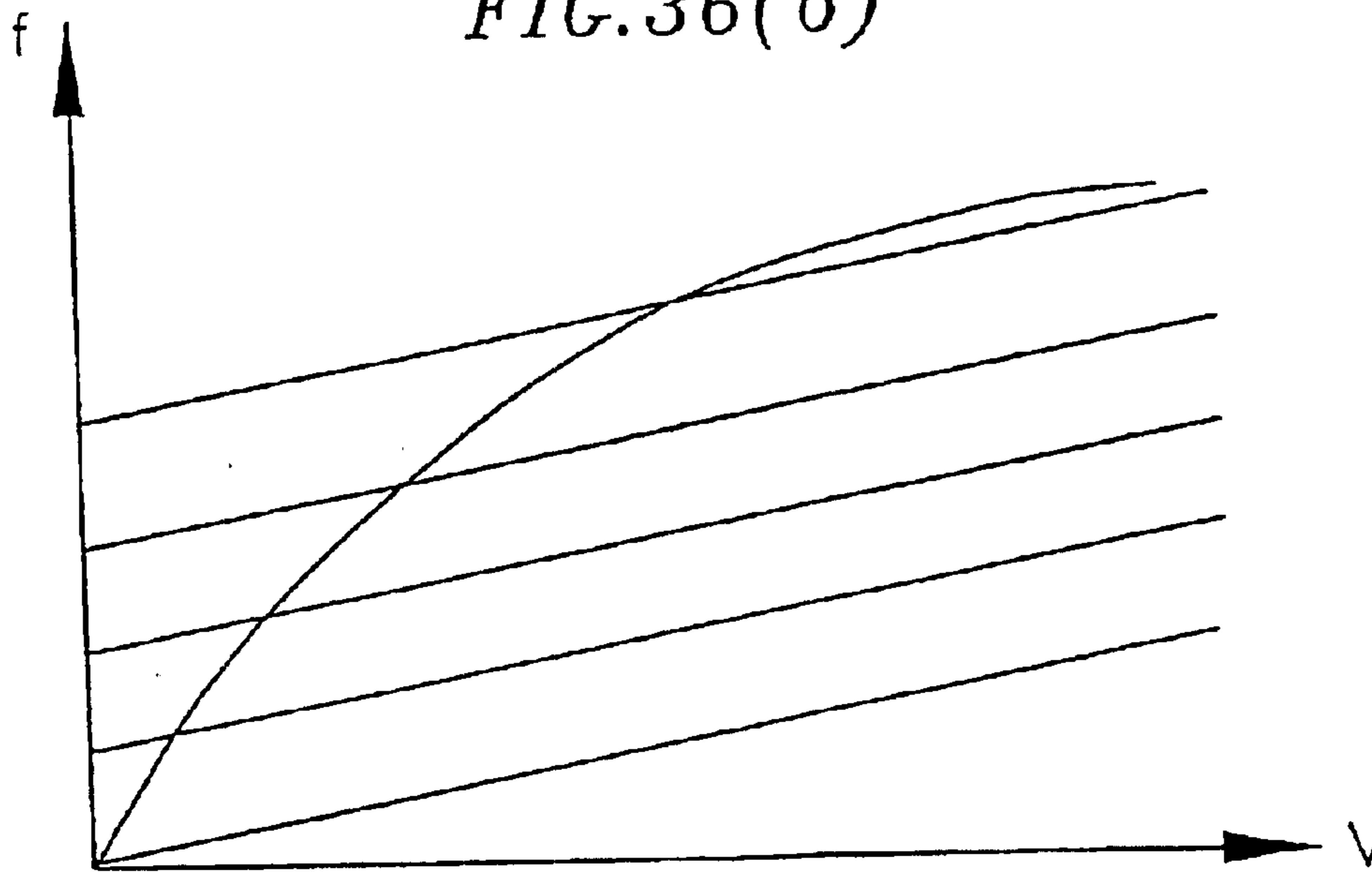
SEGMENTED VCO TUNING CURVE
