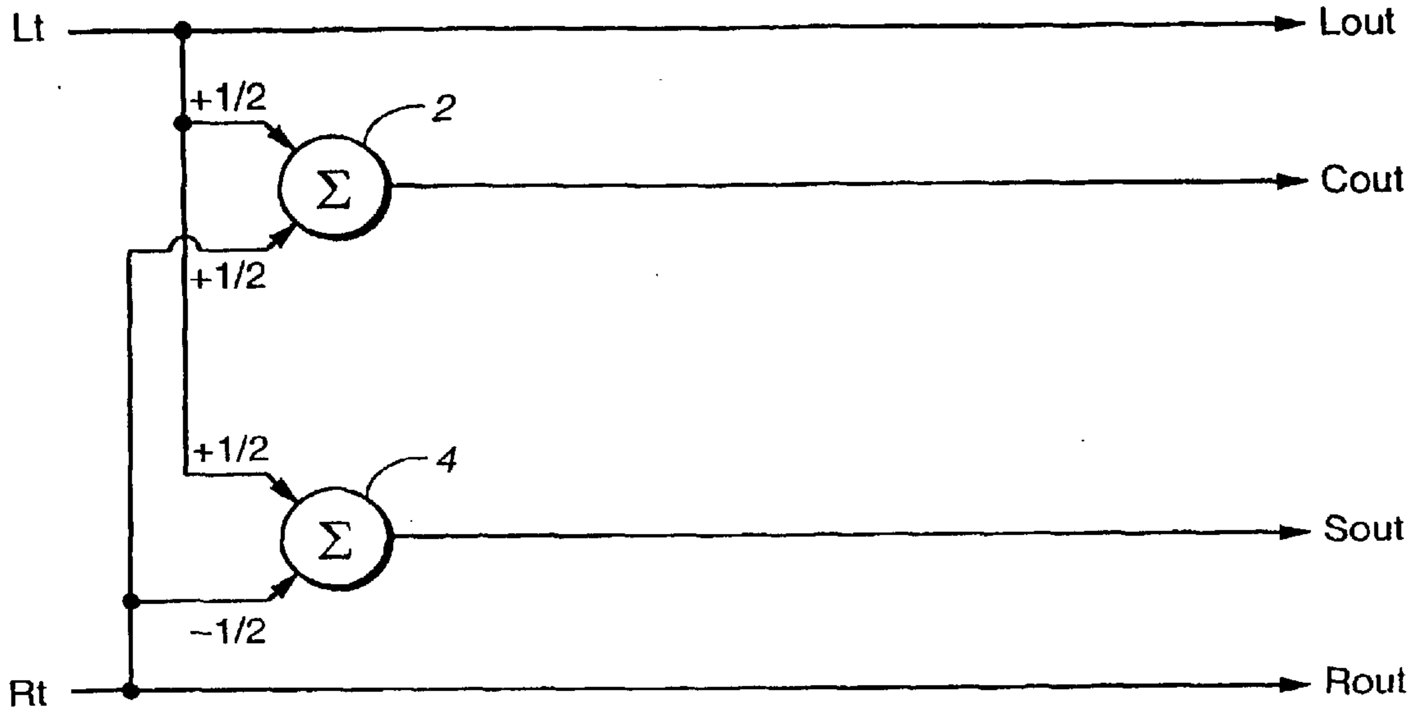
FIG. 1 (PRIOR ART)
