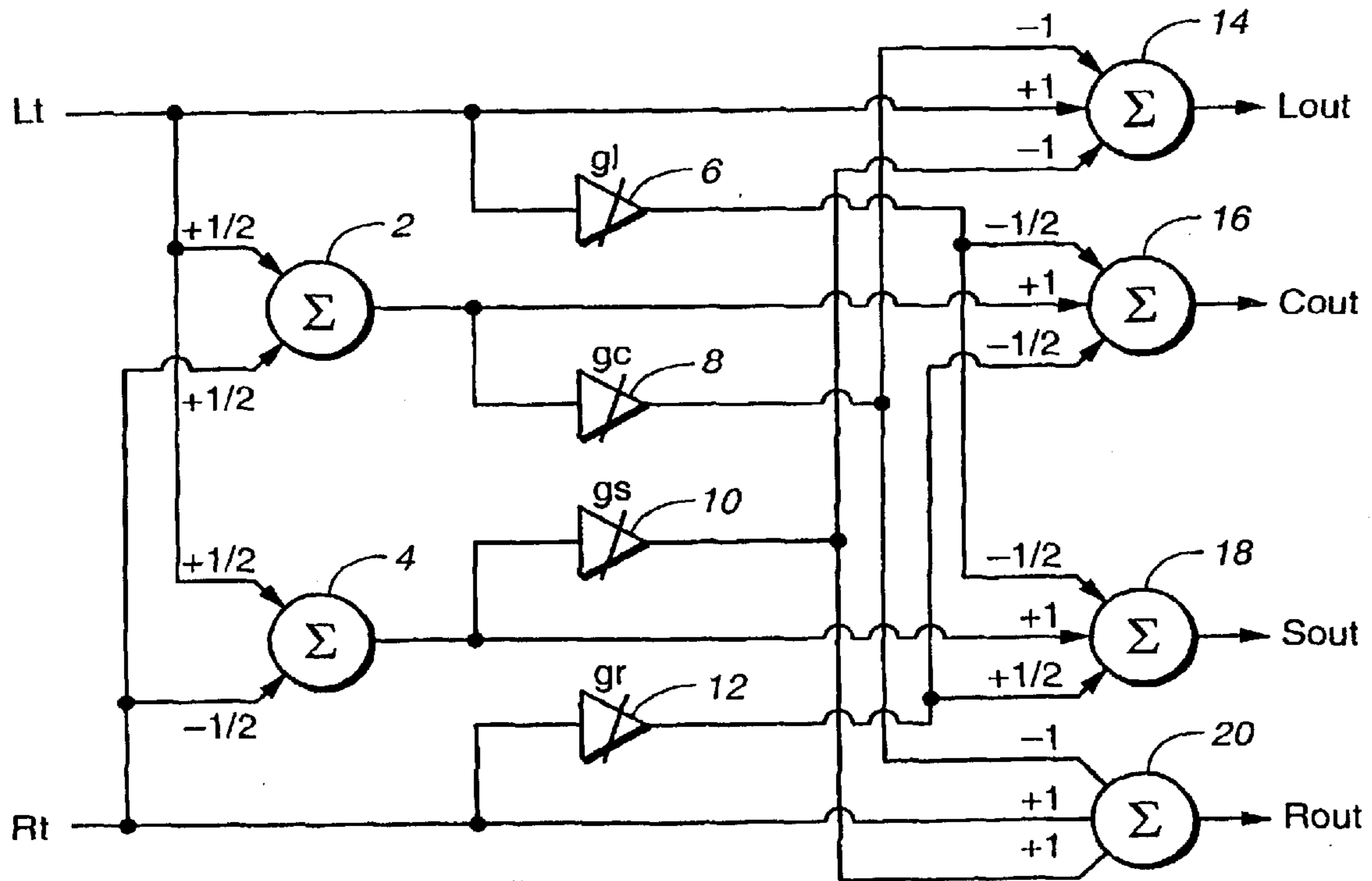
FIG. 2 (PRIOR ART)
