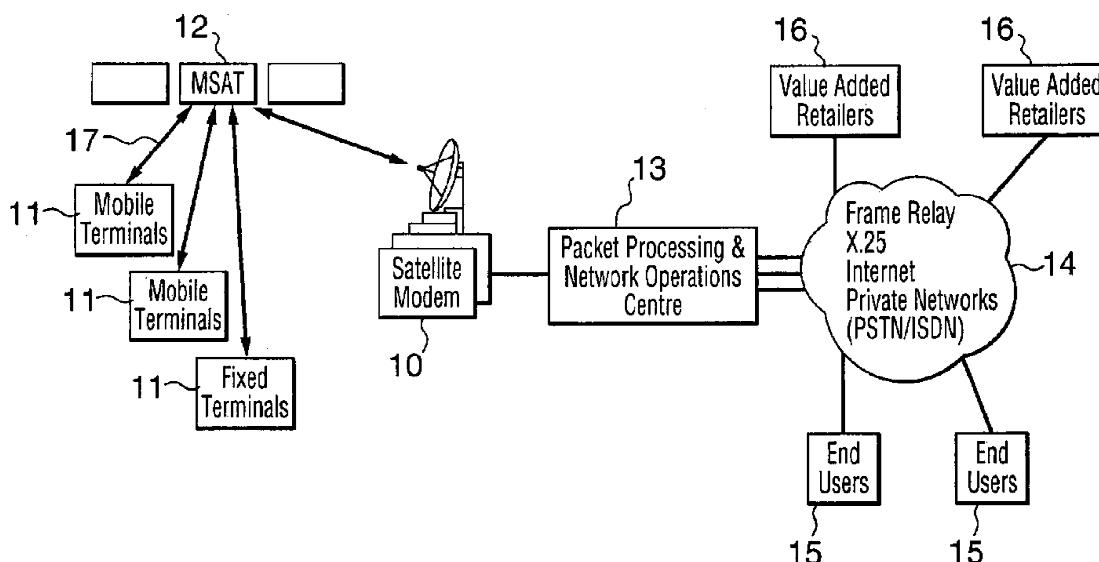
Satellite Packet Data Network Architecture
