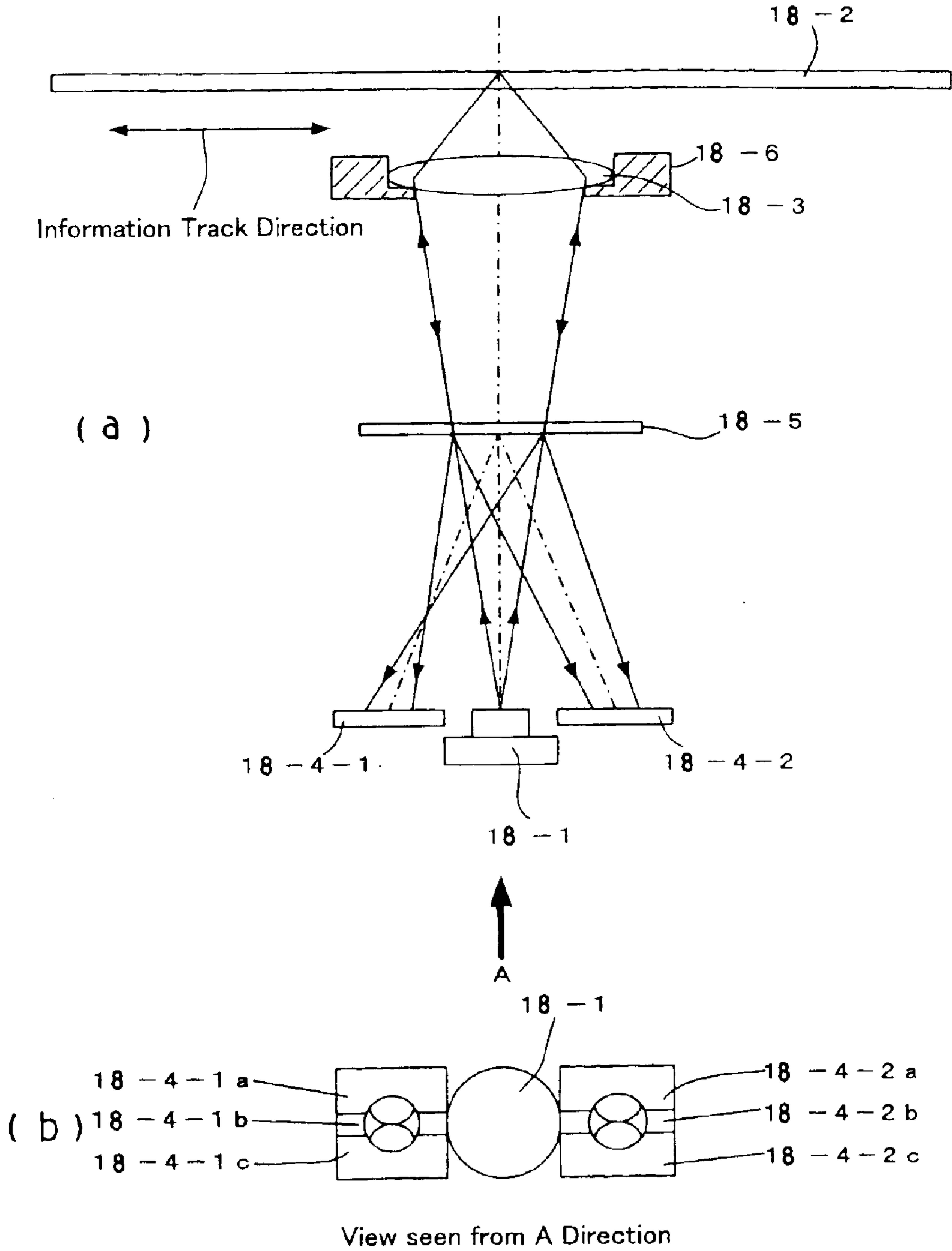
FIG. 18 (PRIOR ART)
