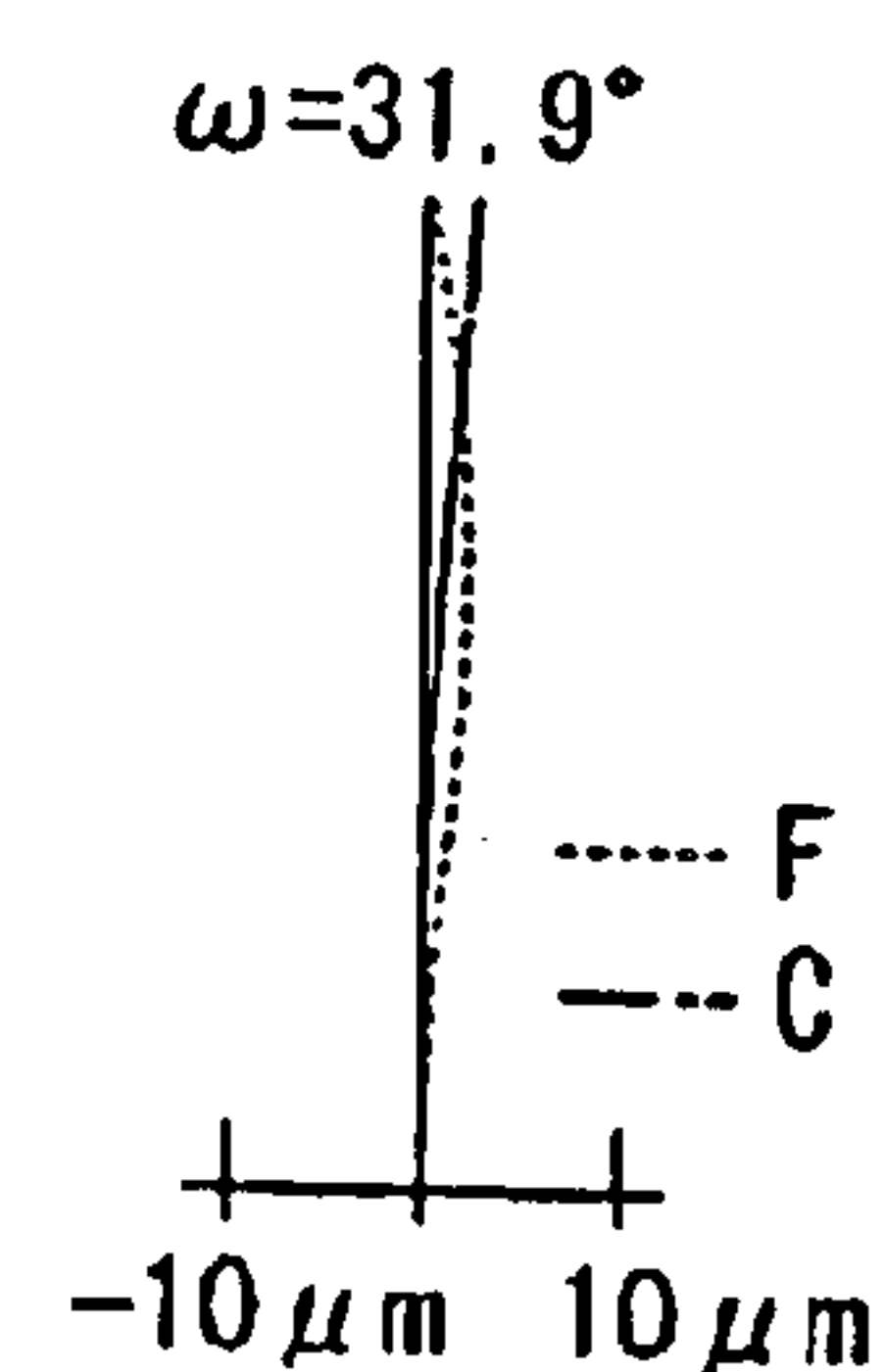
Lateral Color Fig. 2D
