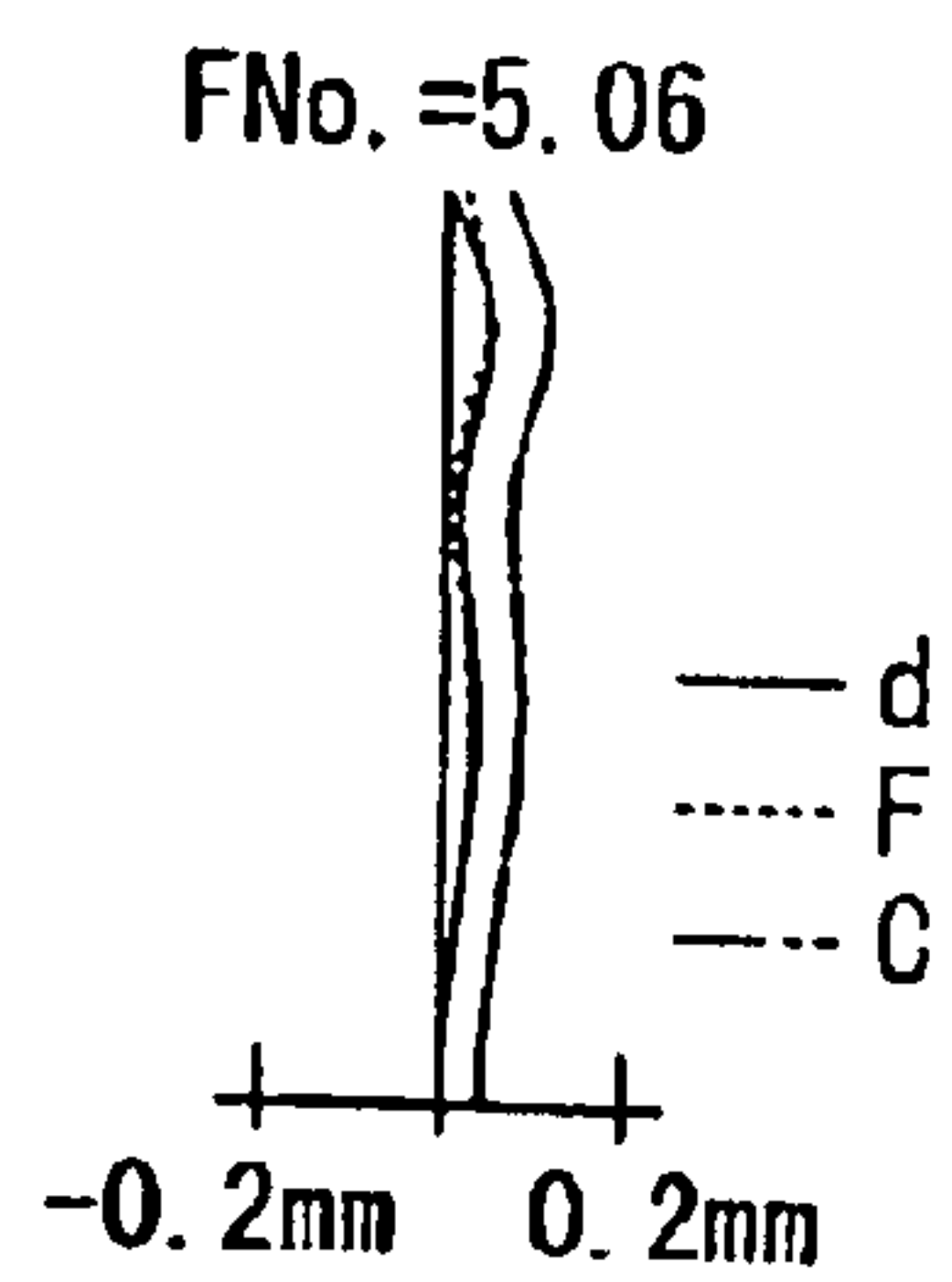
Spherical Aberration Fig. 3A
