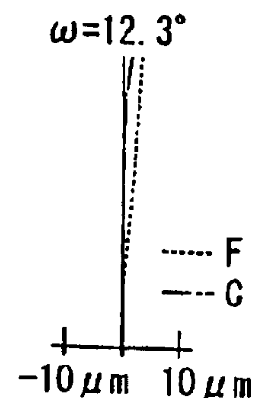
Lateral Color Fig. 3D
