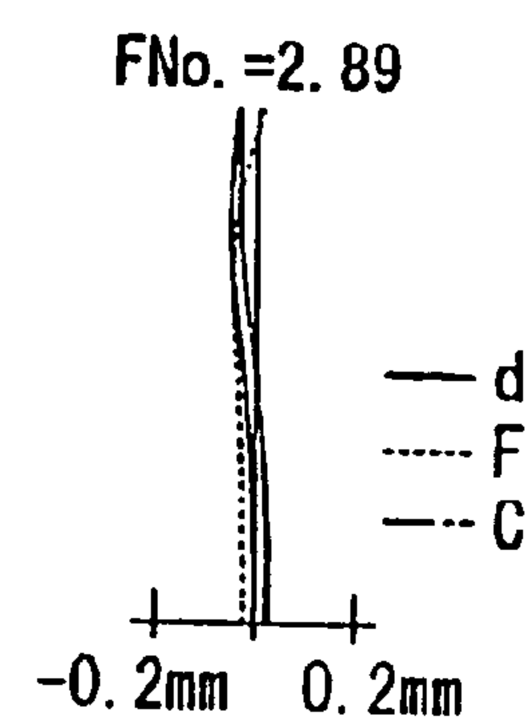
Spherical Aberration Fig. 2A
