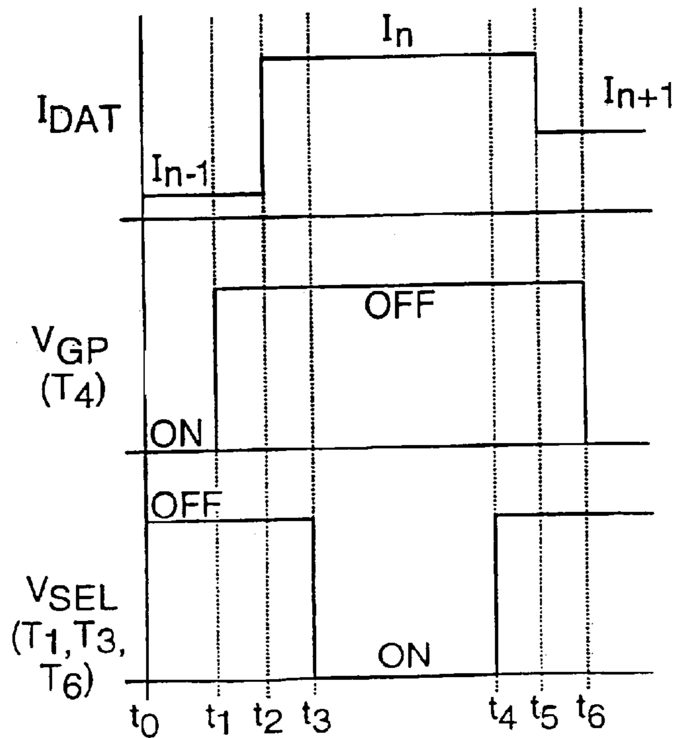
DRIVING WAVEFORM
