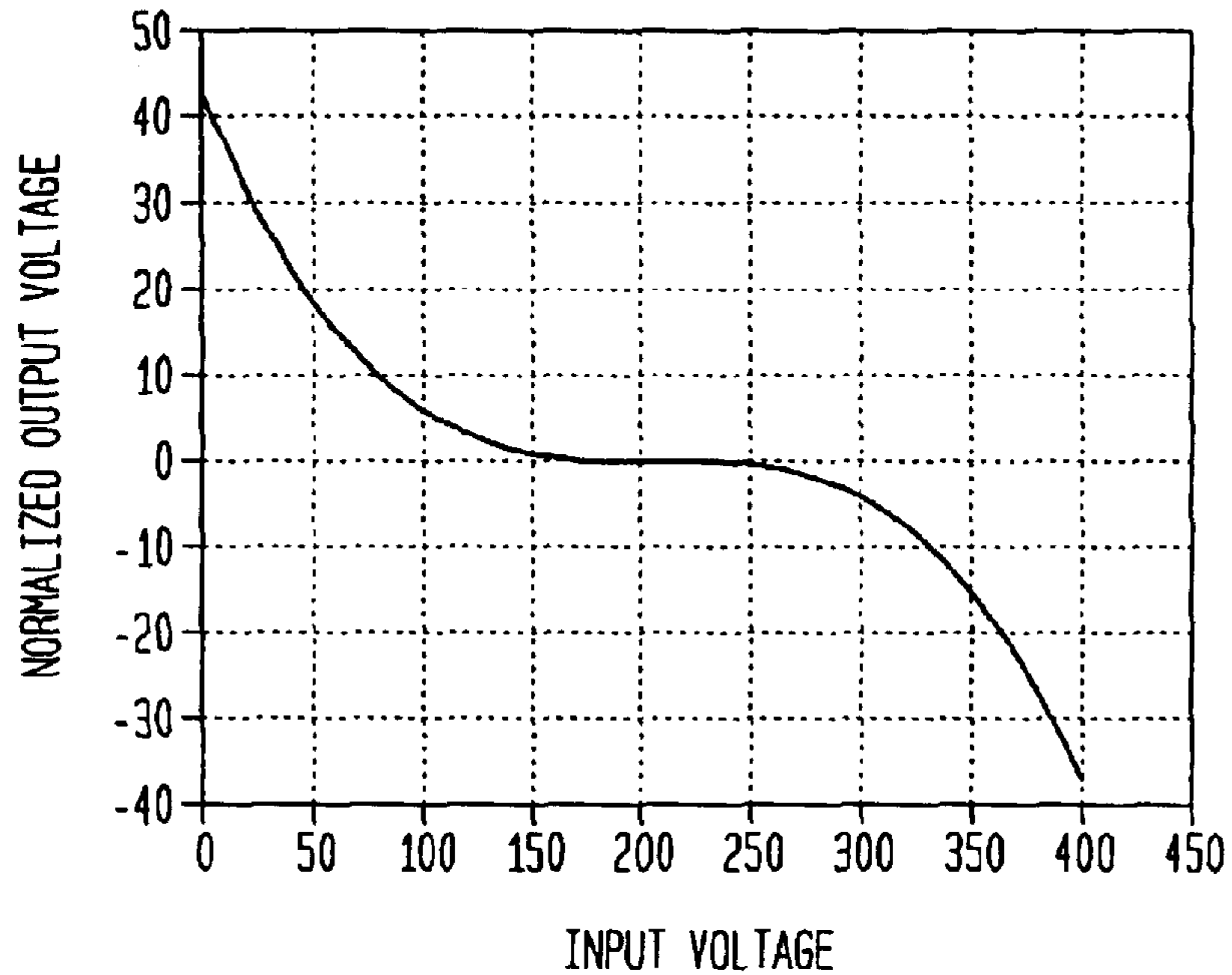
AM-AM CHARACTERISTIC
