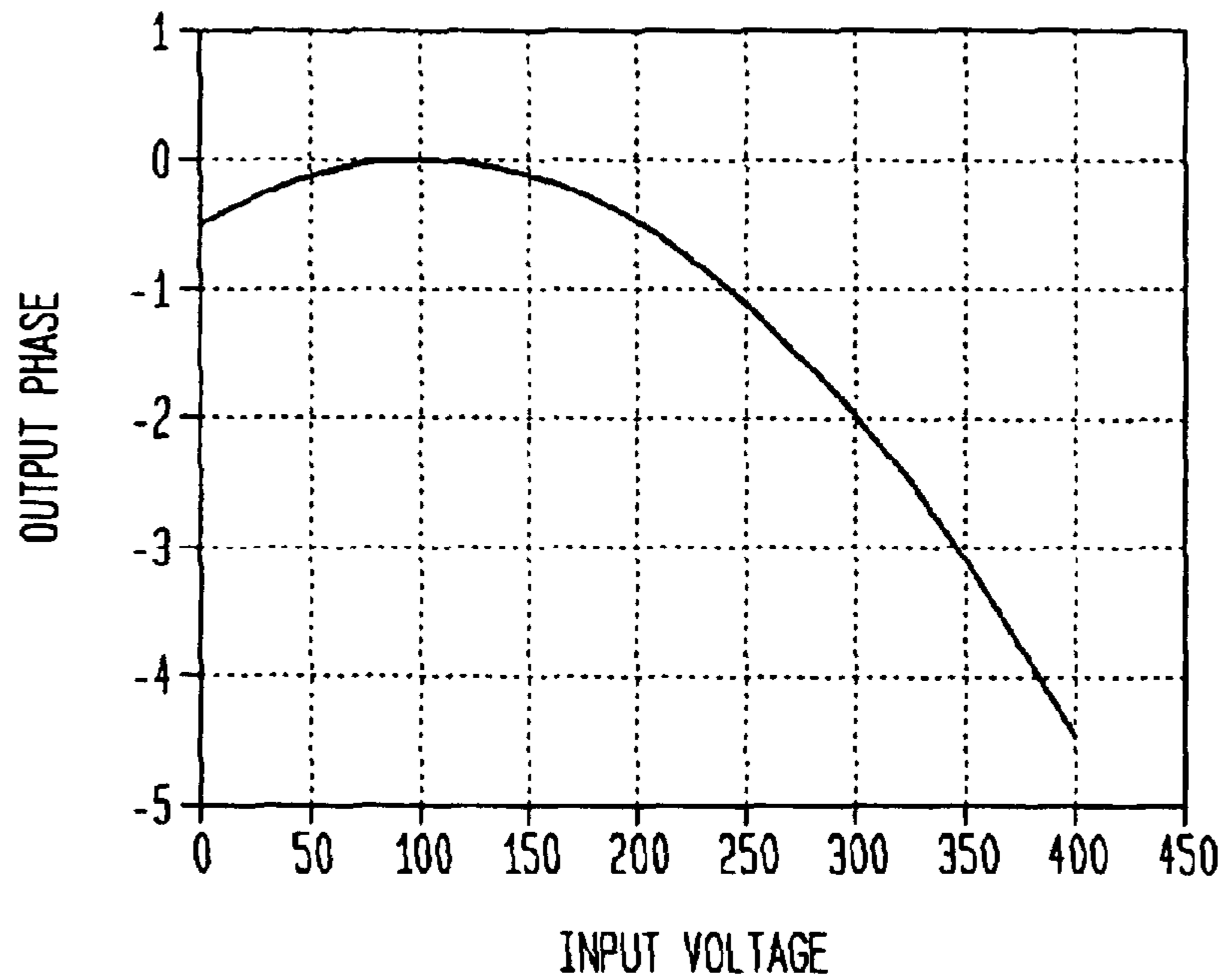
AM-PM CHARACTERISTIC
