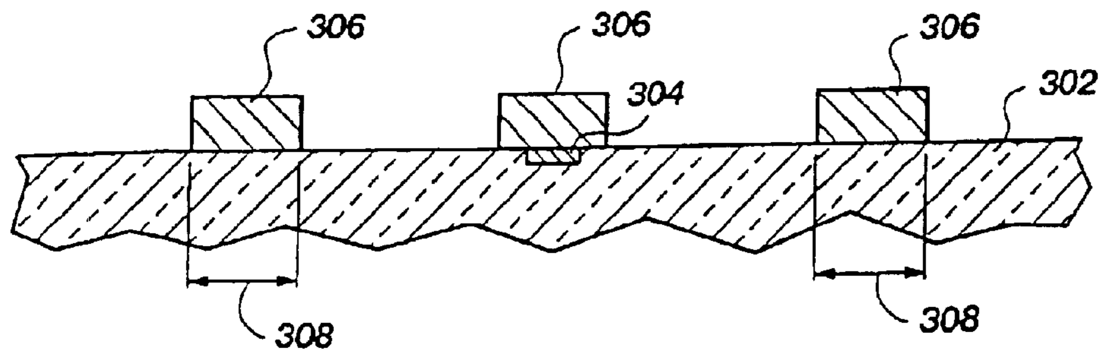
Fig. 43 (PRIOR ART)
