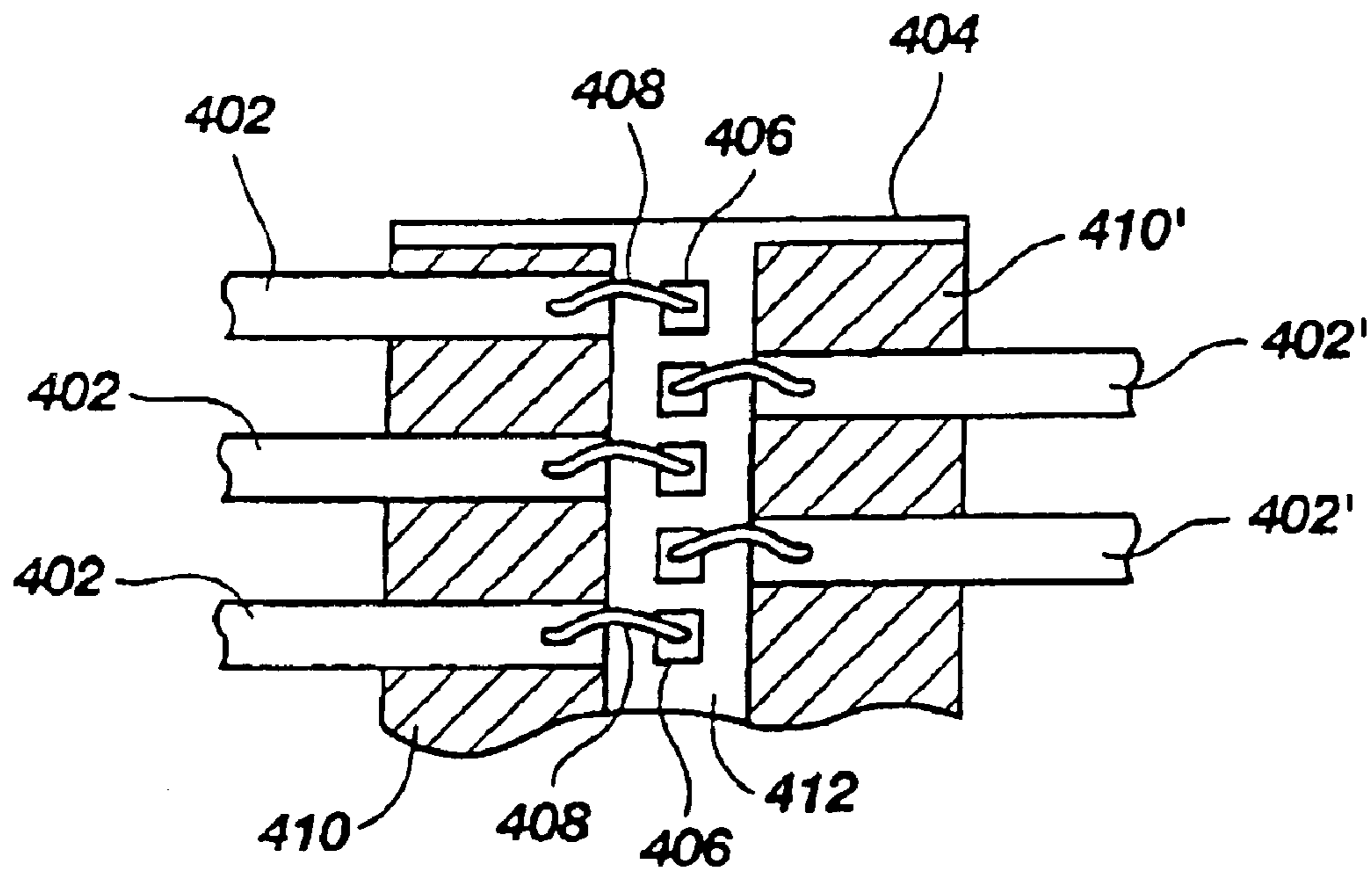
Fig. 50 (PRIOR ART)
