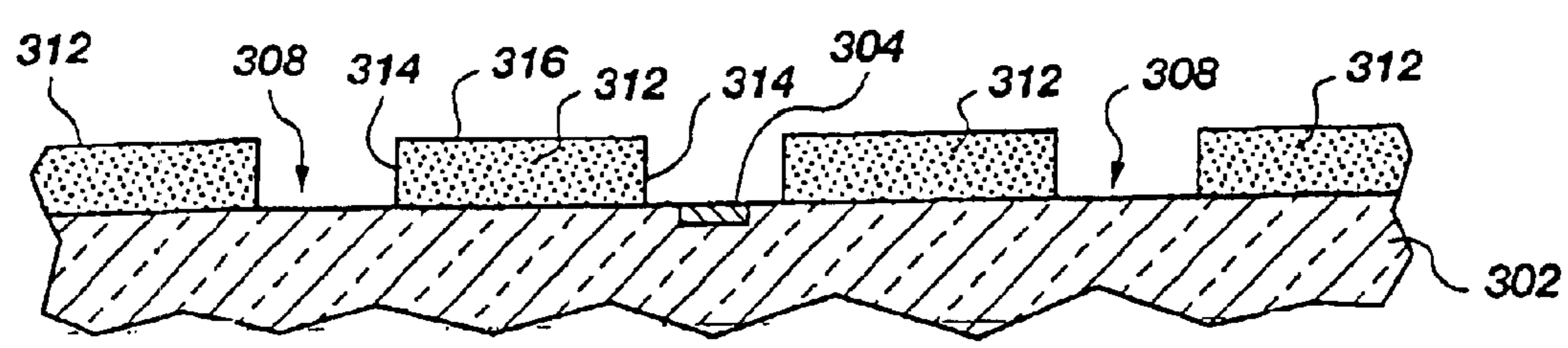
Fig. 45 (PRIOR ART)
