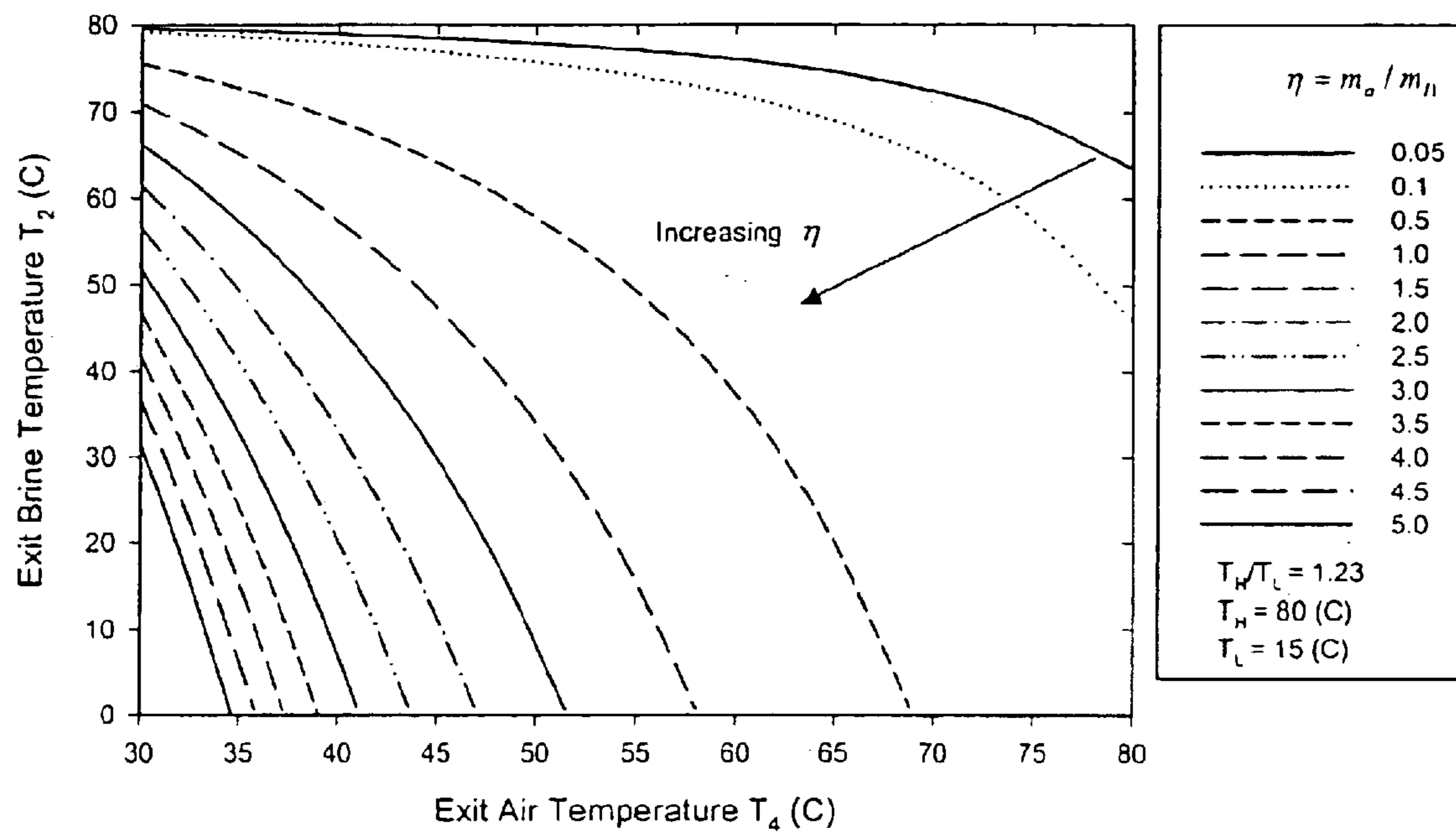
Variation of exit brine temperature with exit air temperature for T_H = 80 \text{ }^\circ\text{C} .
