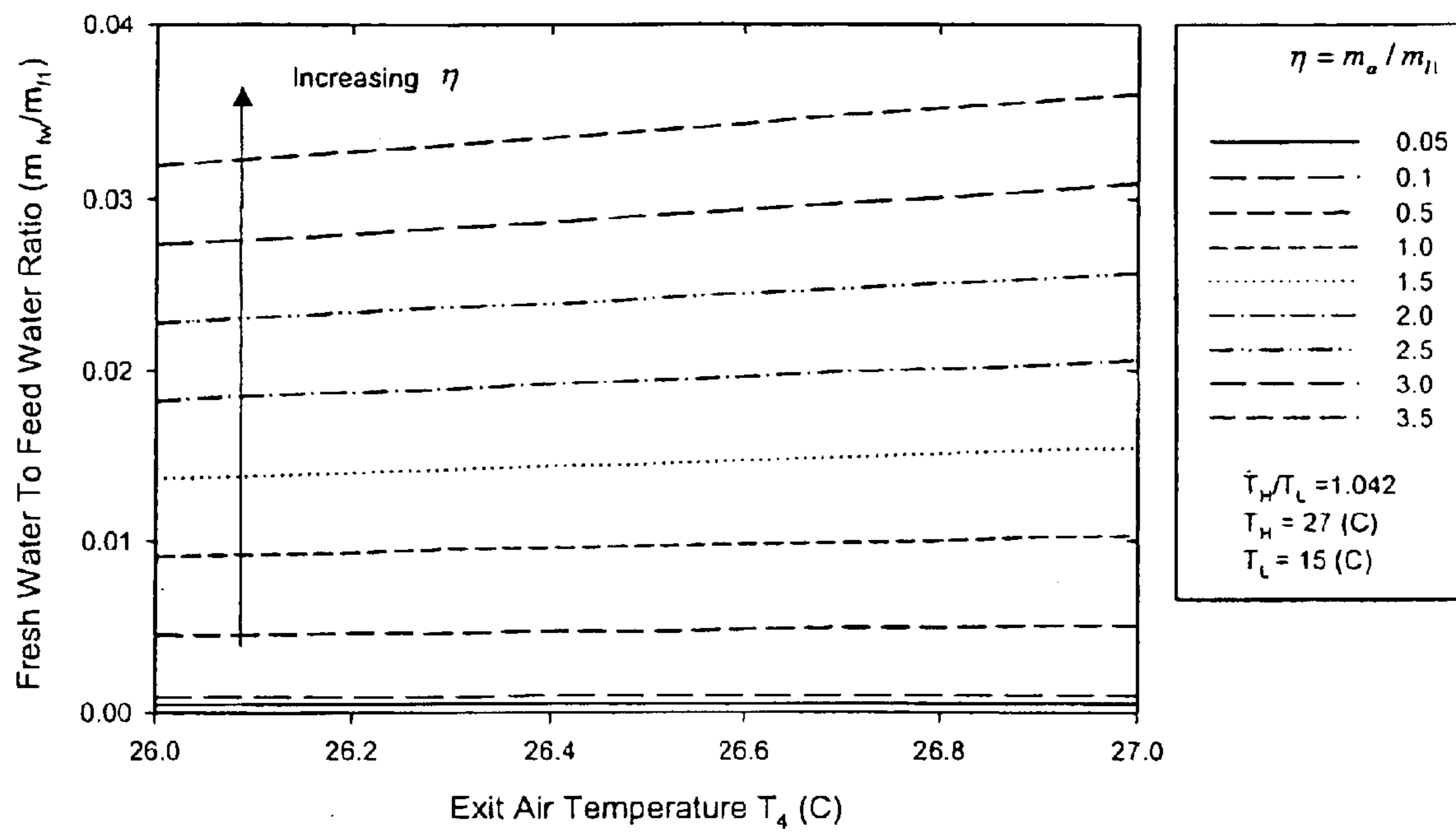
Fresh water production efficiency for T_H = 27 \text{ }^\circ\text{C} .
