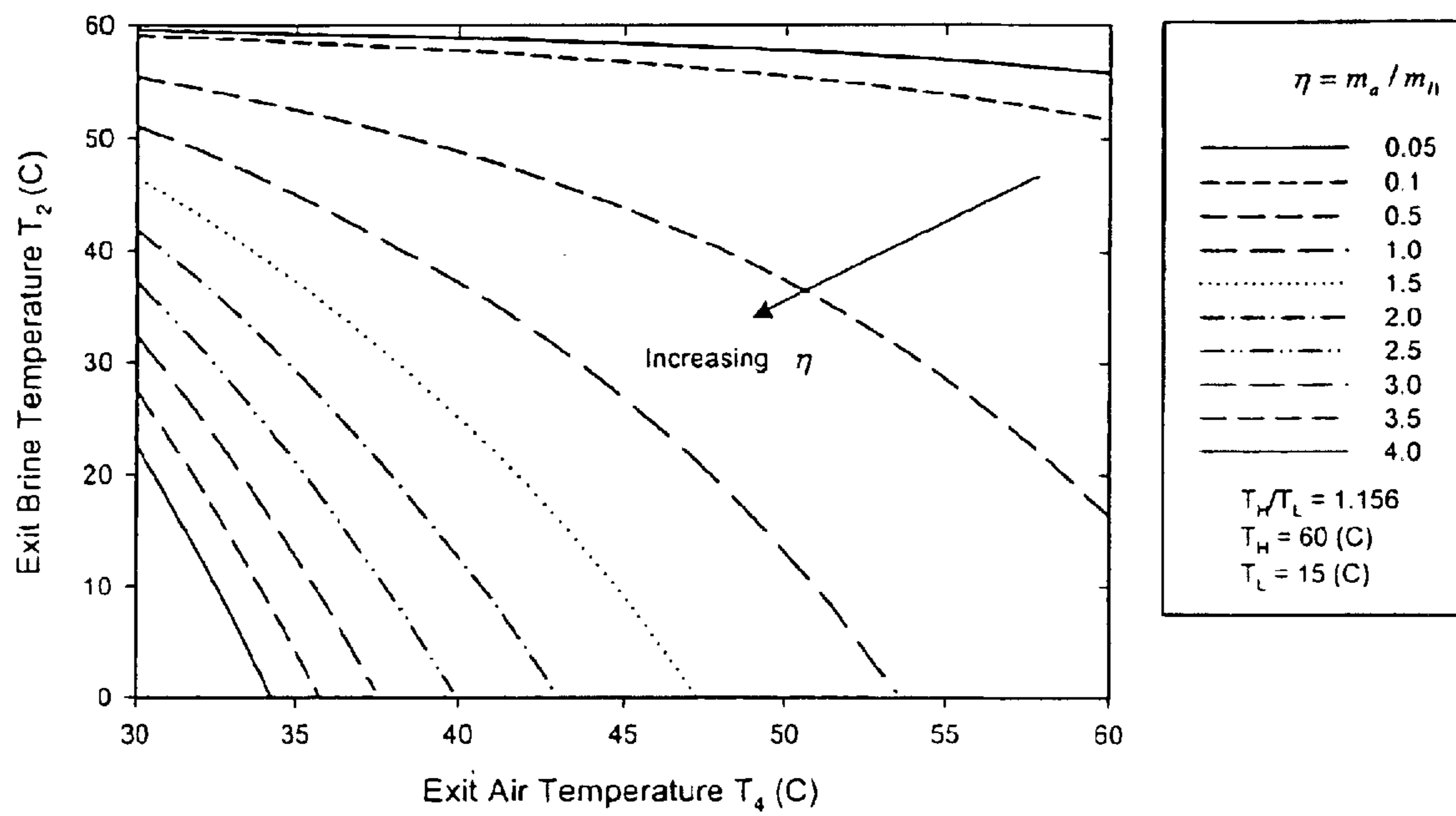
Variation of exit brine temperature with exit air temperature for T_H = 60 °C.
