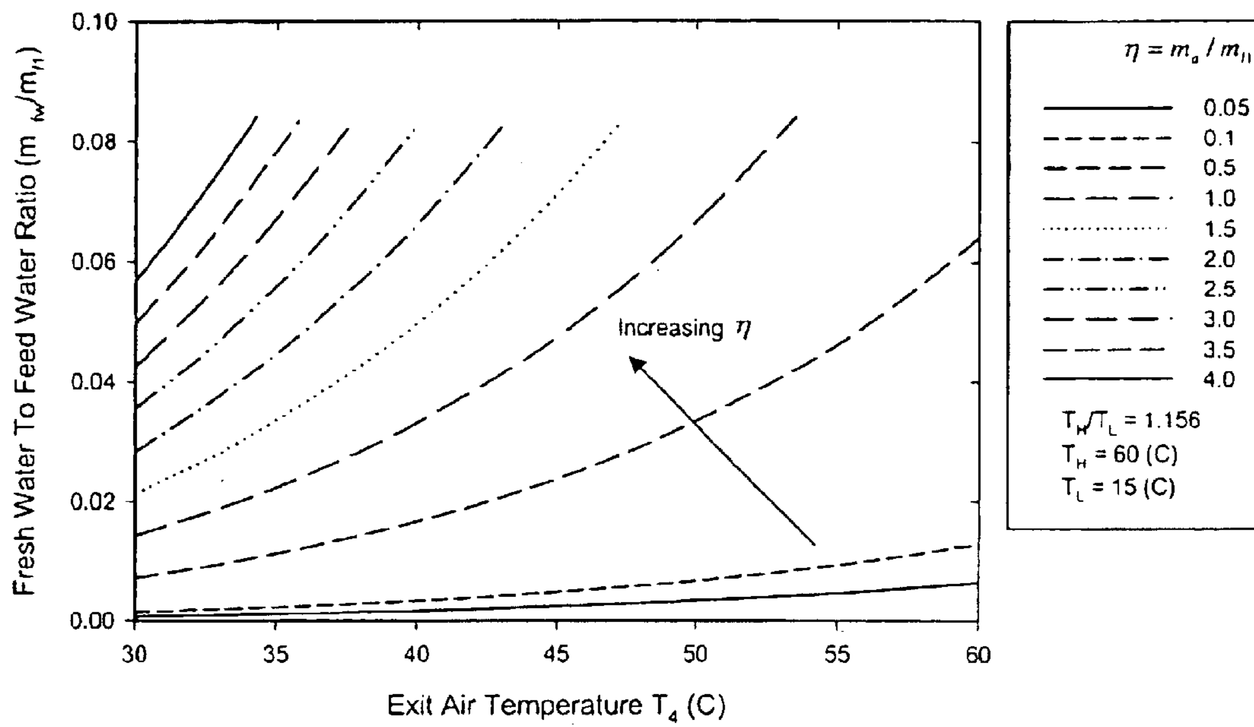
Fresh water production efficiency for T_H = 60 °C.
