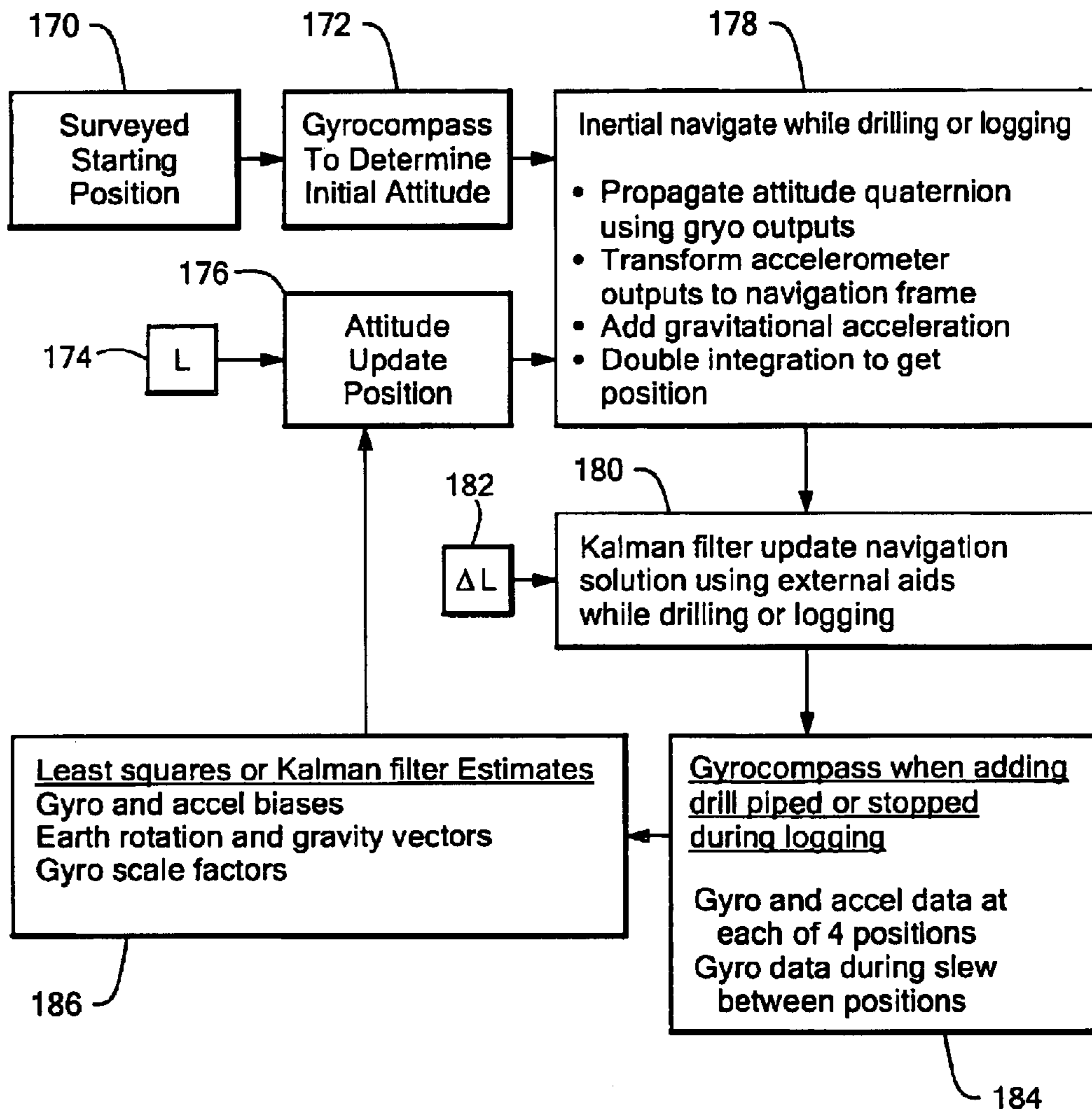
INERTIAL NAVIGATION WHILE DRILLING OR LOGGING
