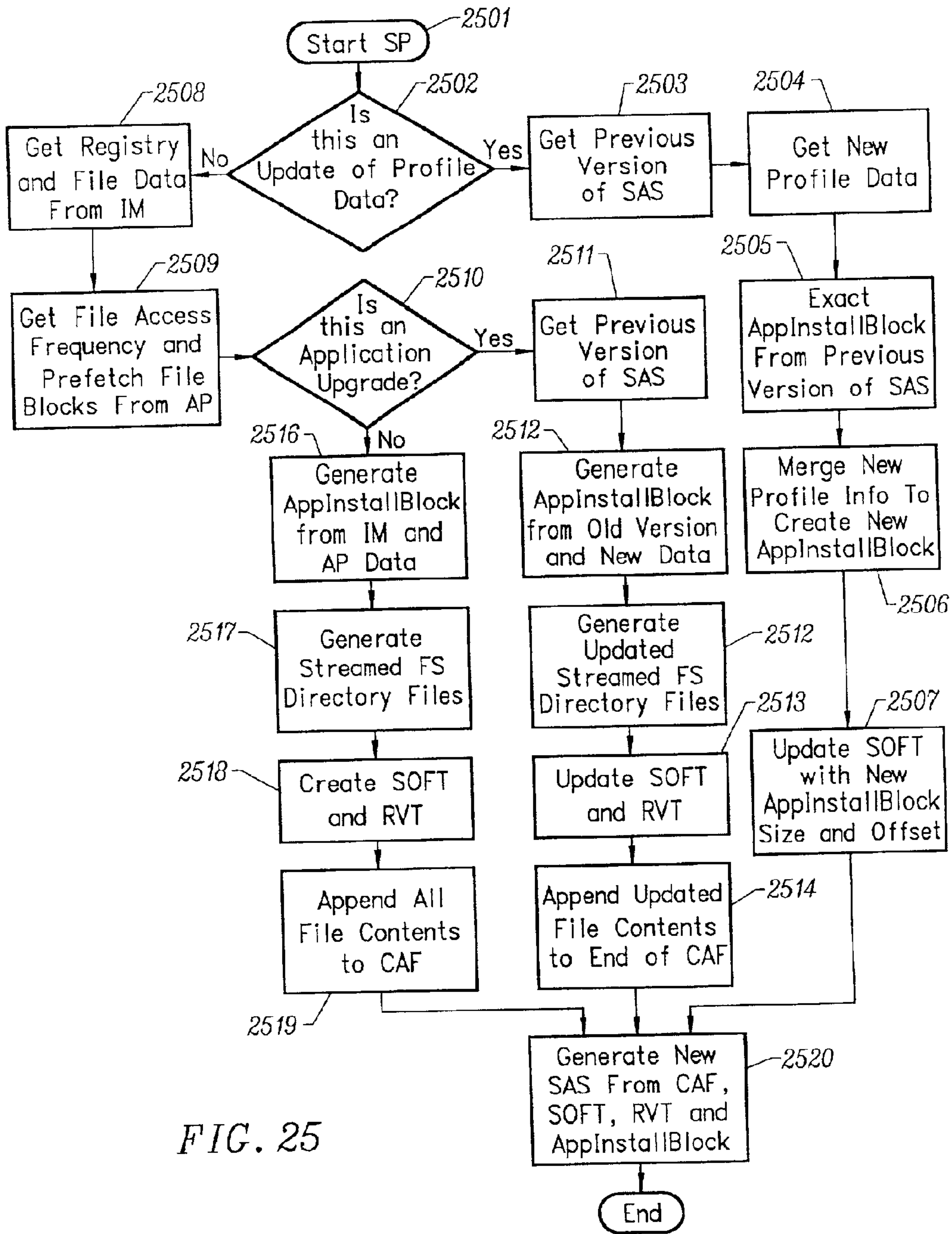
Builder SAS Packager (SP) Control Flow Diagram
