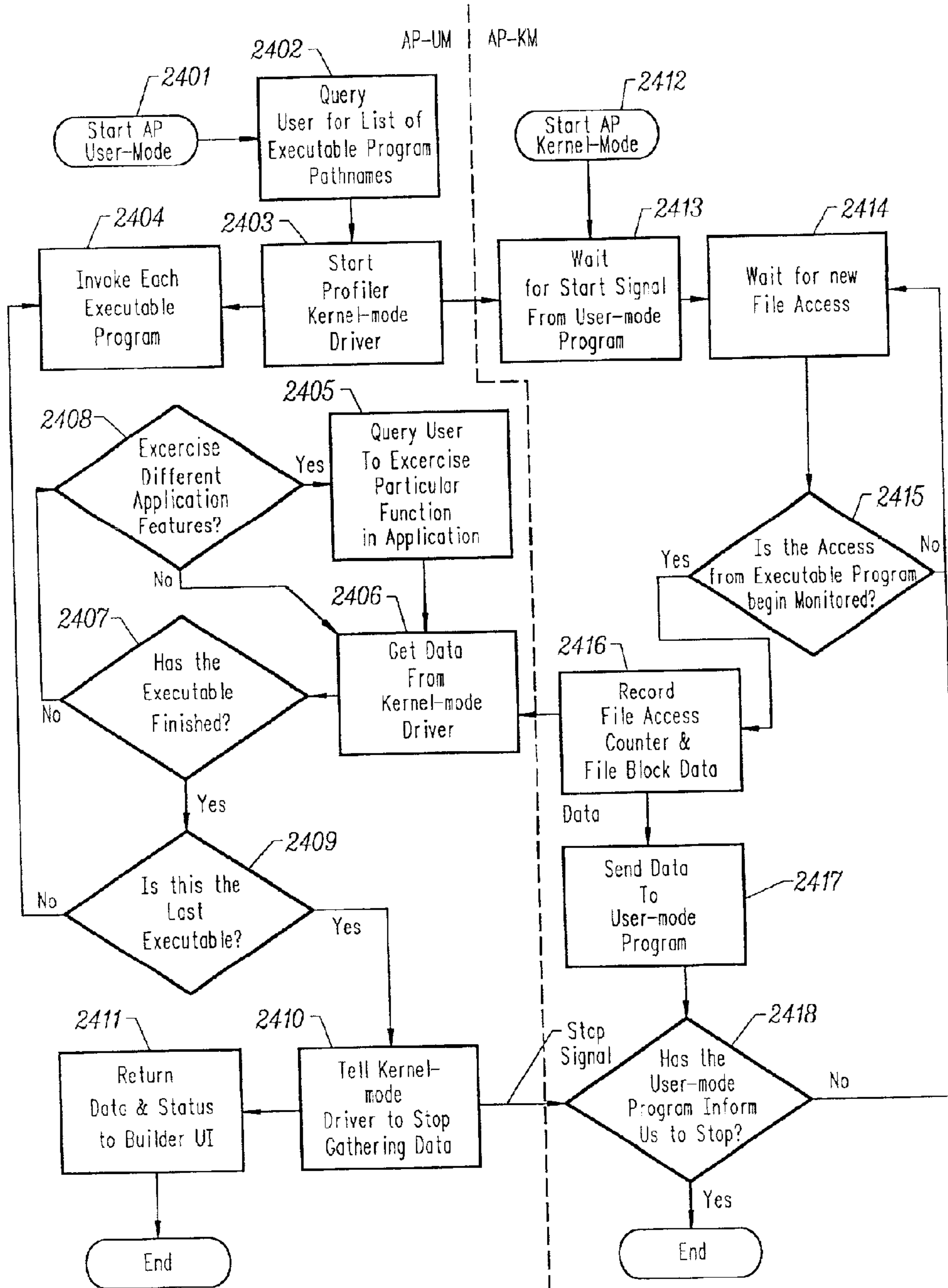
Builder Application Profiler (AP) Control Flow Diagram
