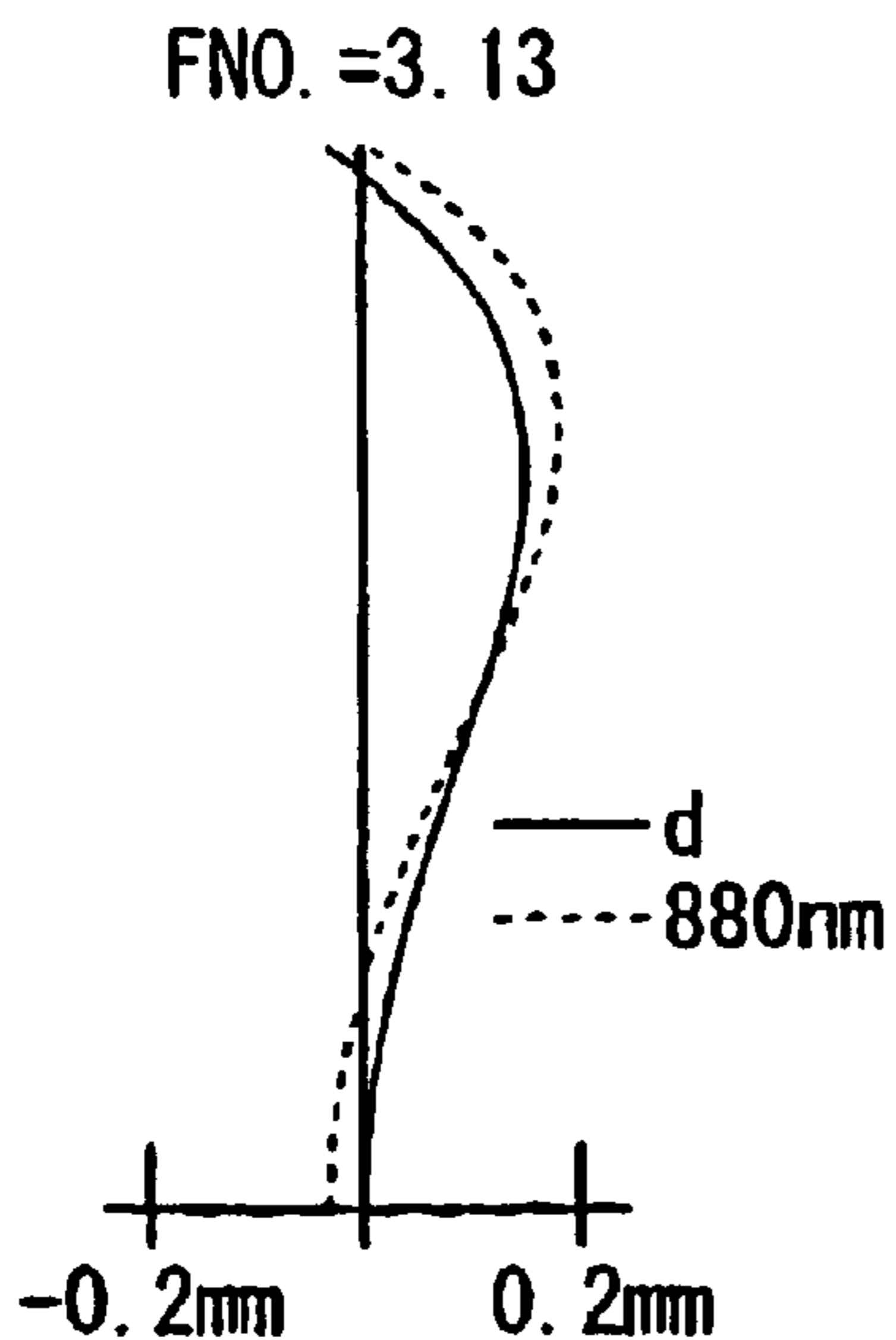
Spherical Aberration Fig. 3A
