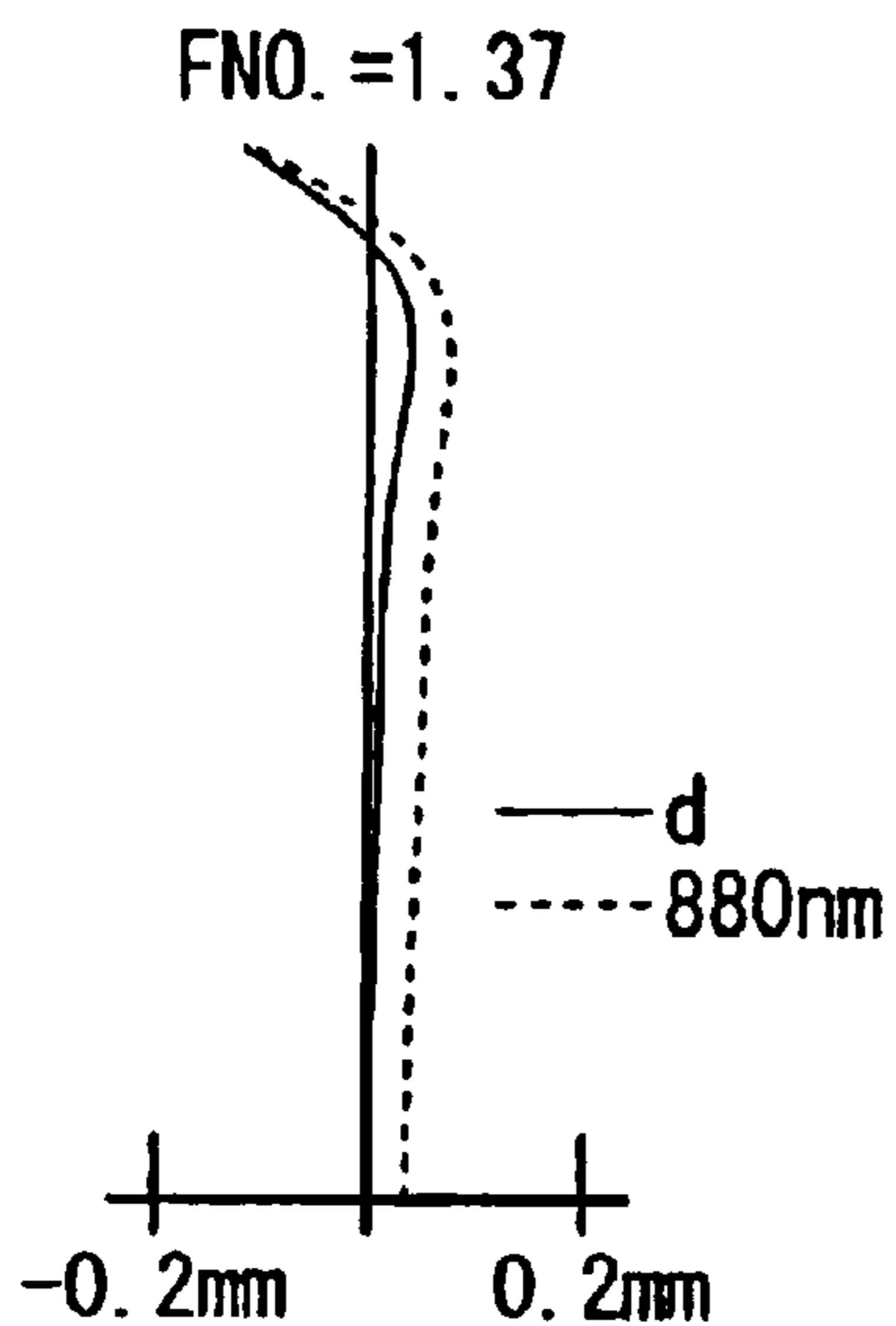
Spherical Aberration Fig. 2A
