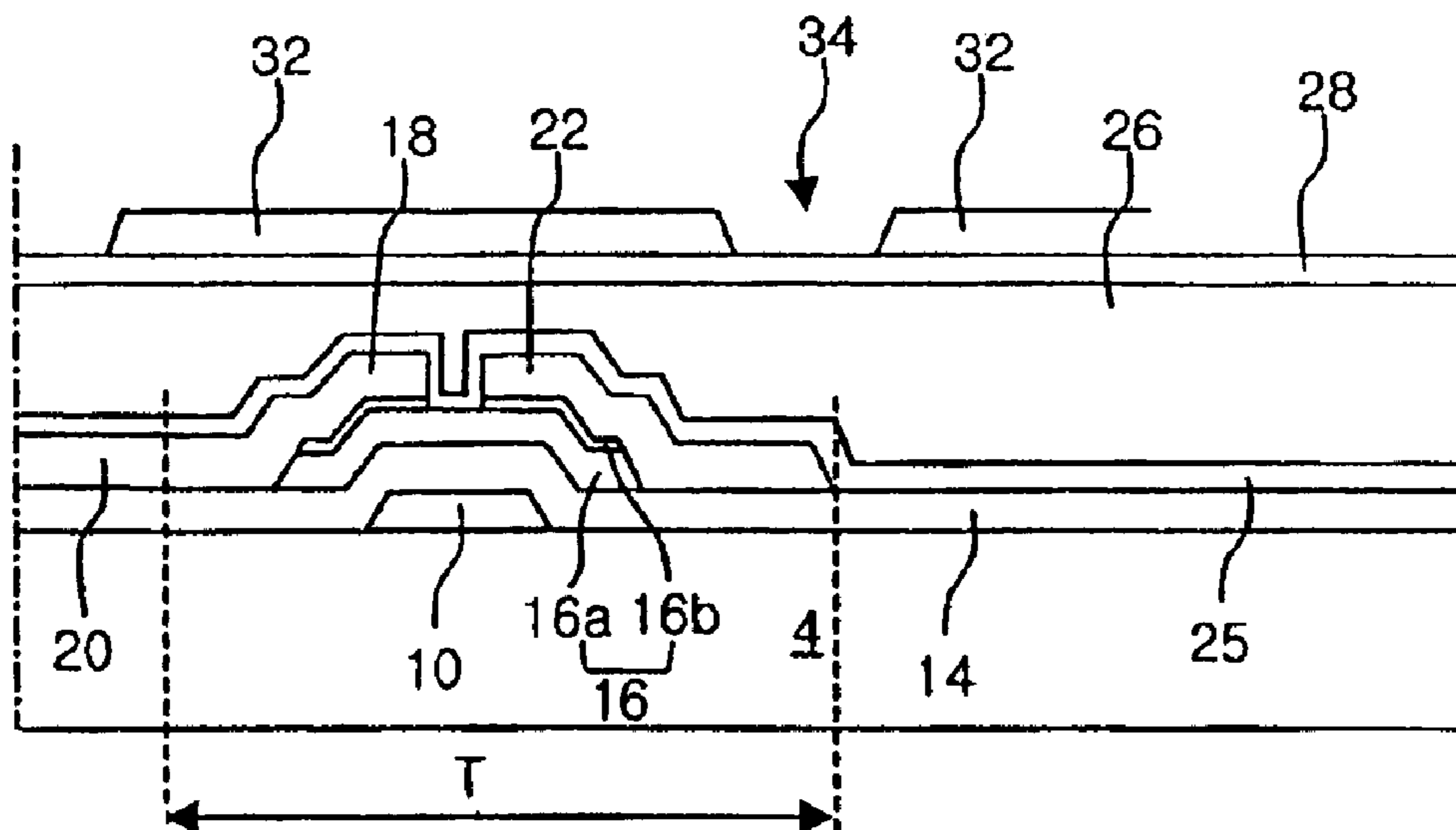
(related art) FIG. 2E
