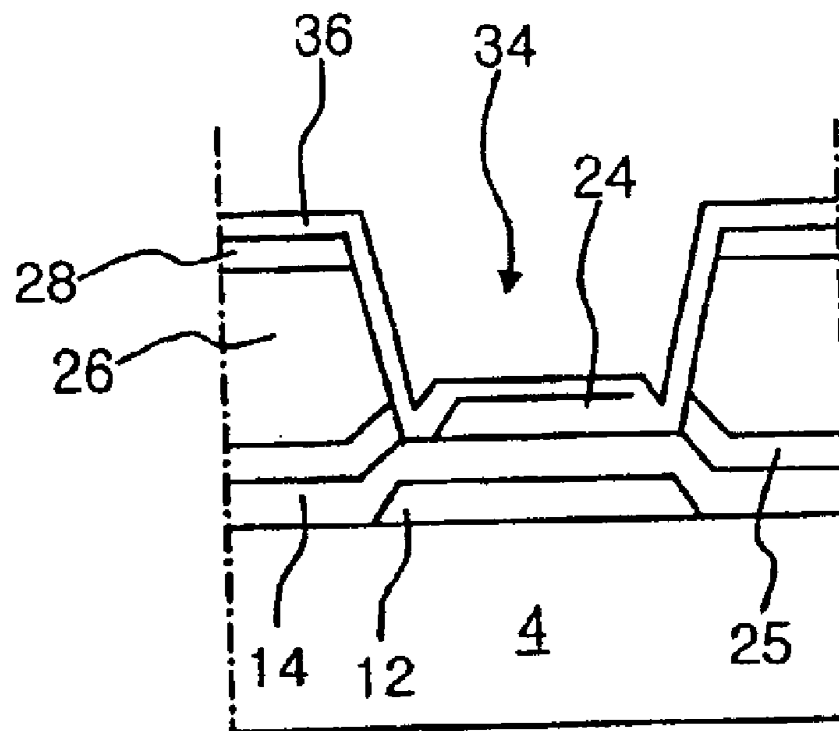
(related art) FIG. 3G
