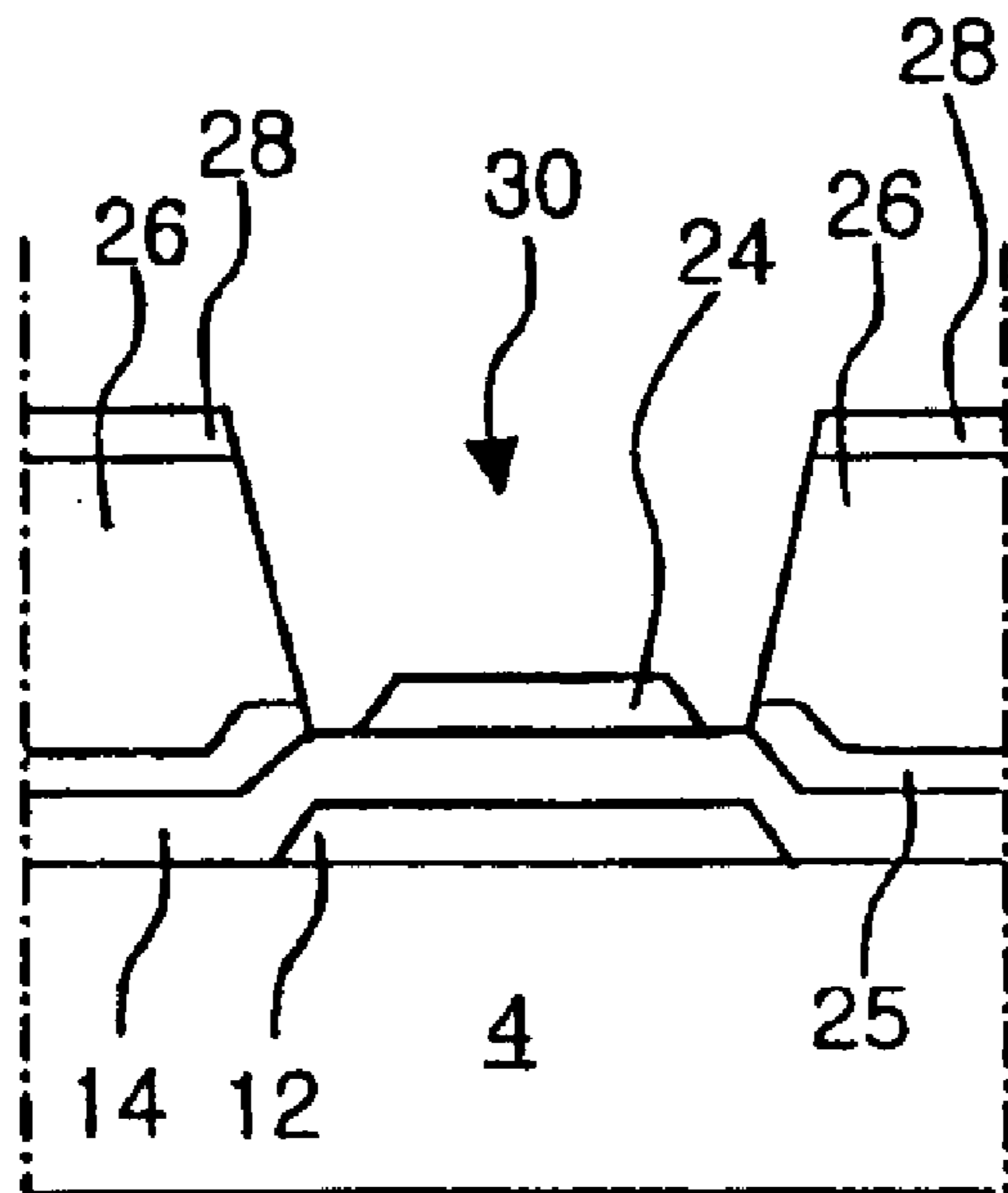
(related art) FIG. 3E
