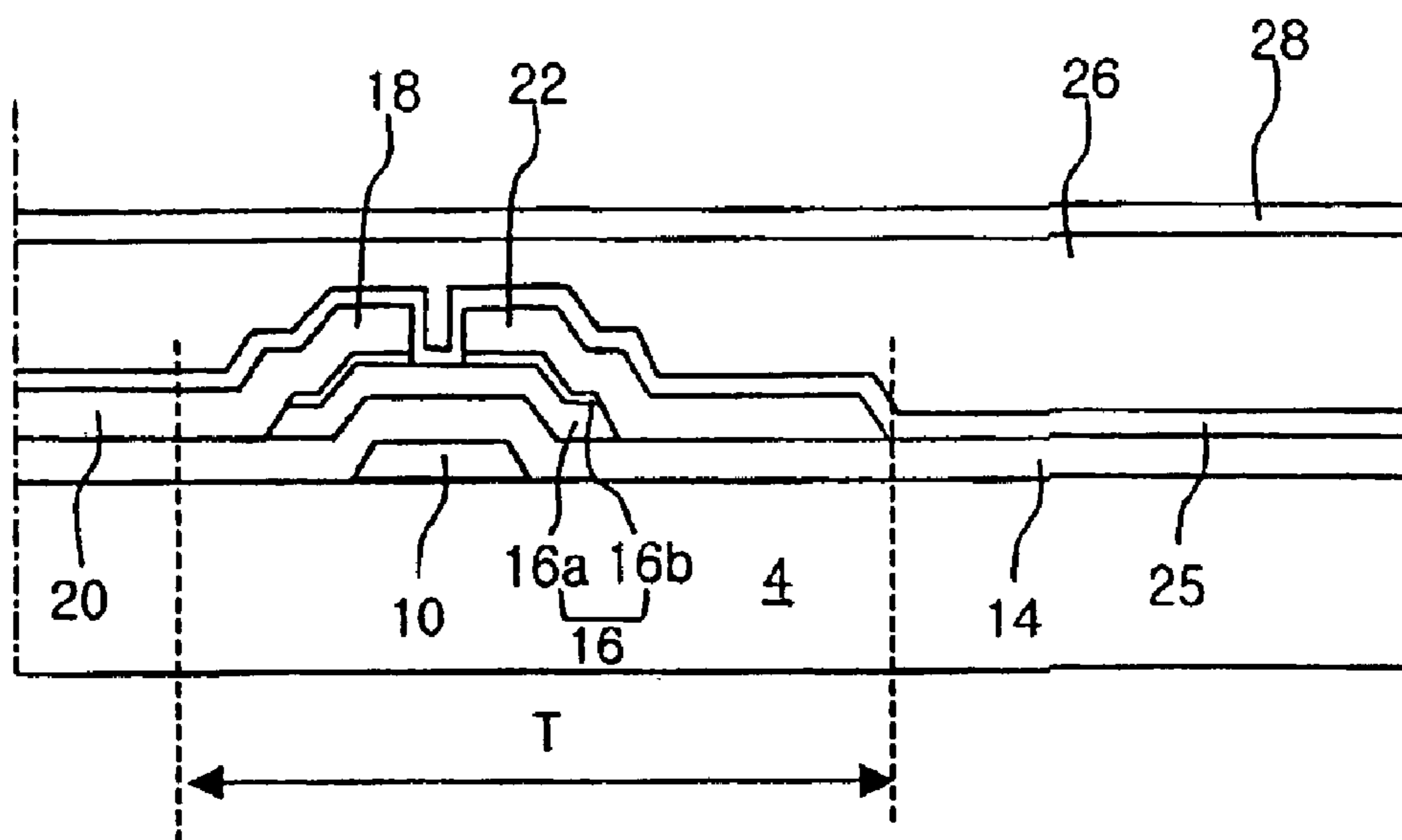
(related art) FIG. 2D
