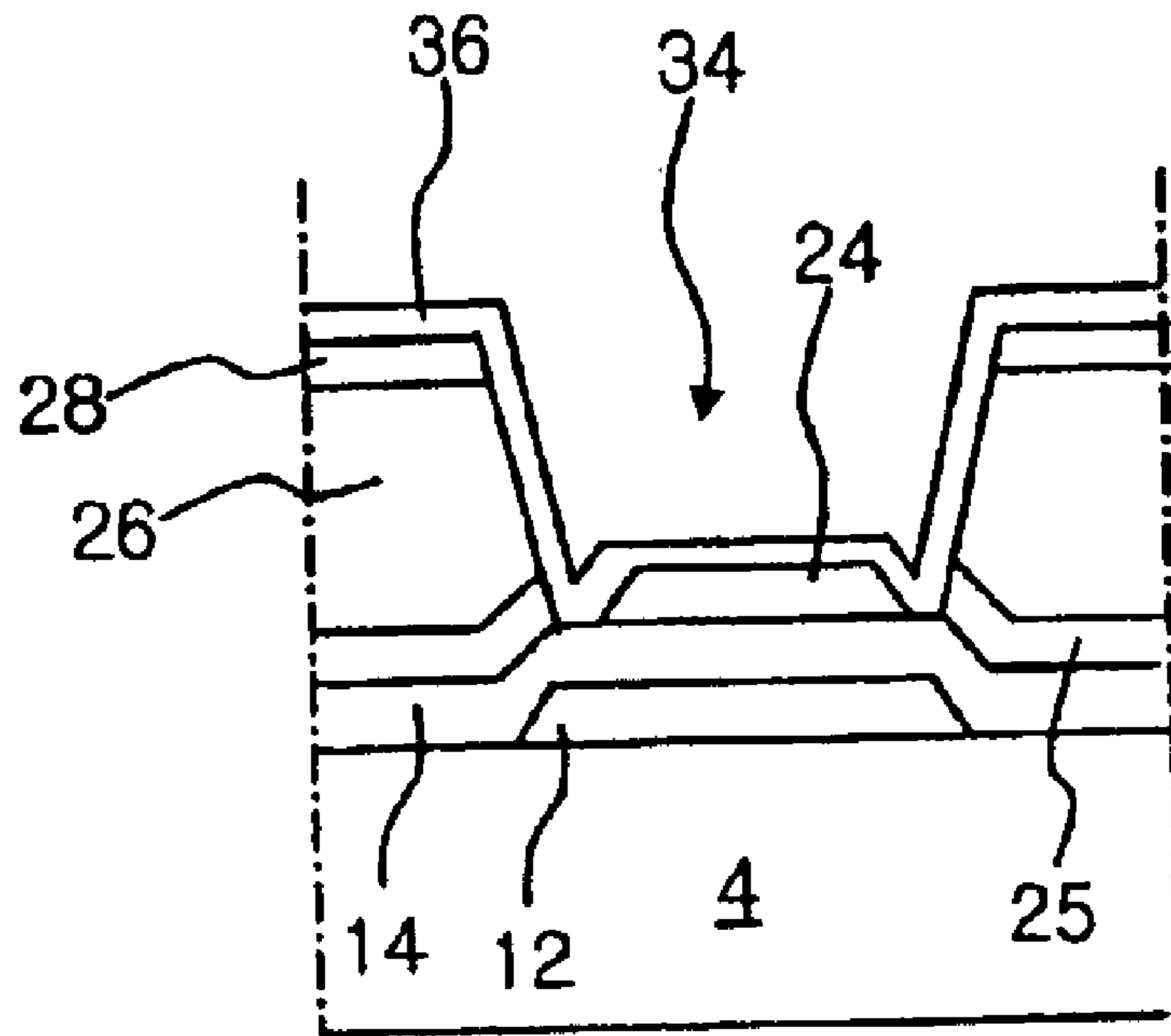
(related art) FIG. 3F
