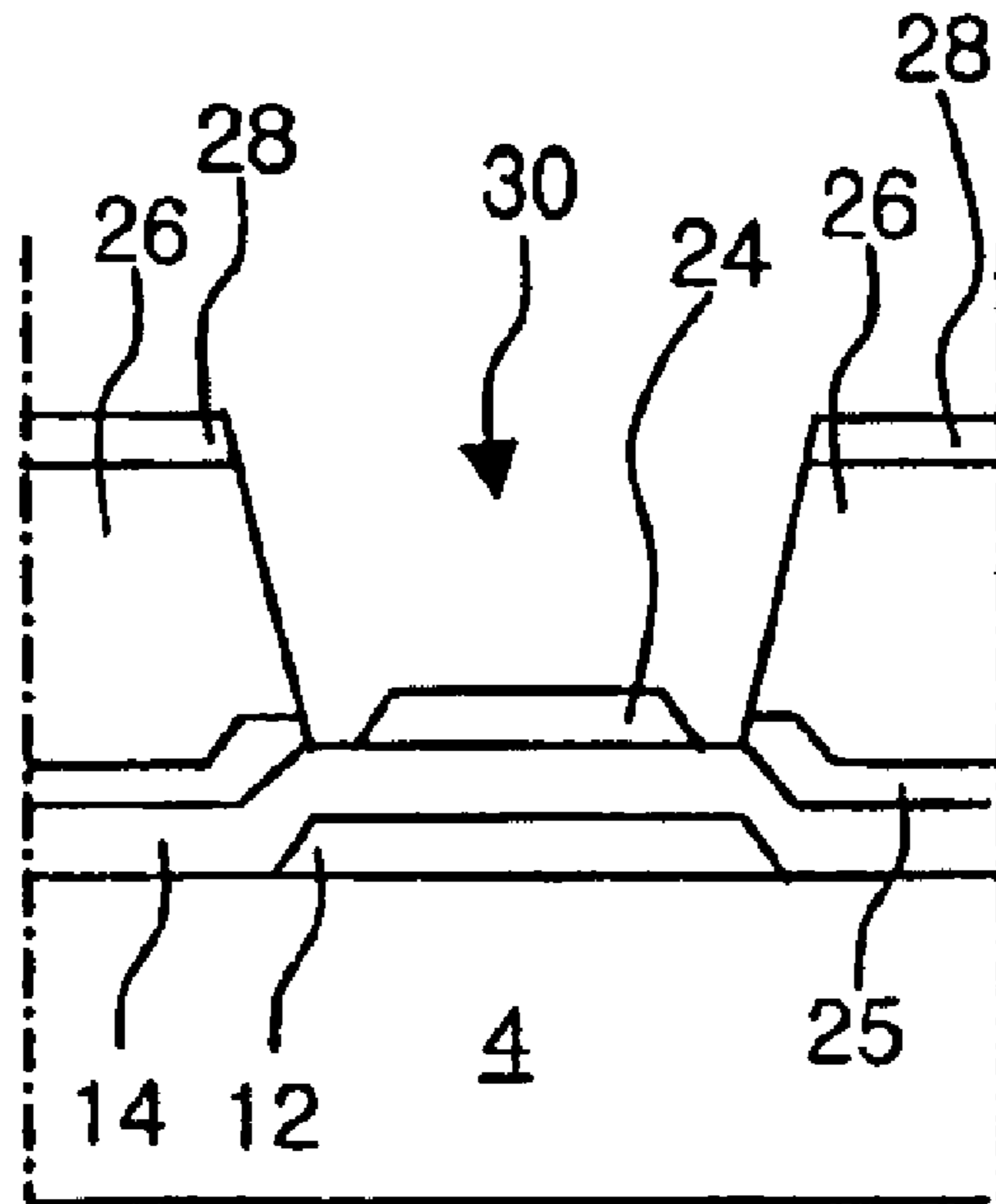
(related art) FIG. 3D
