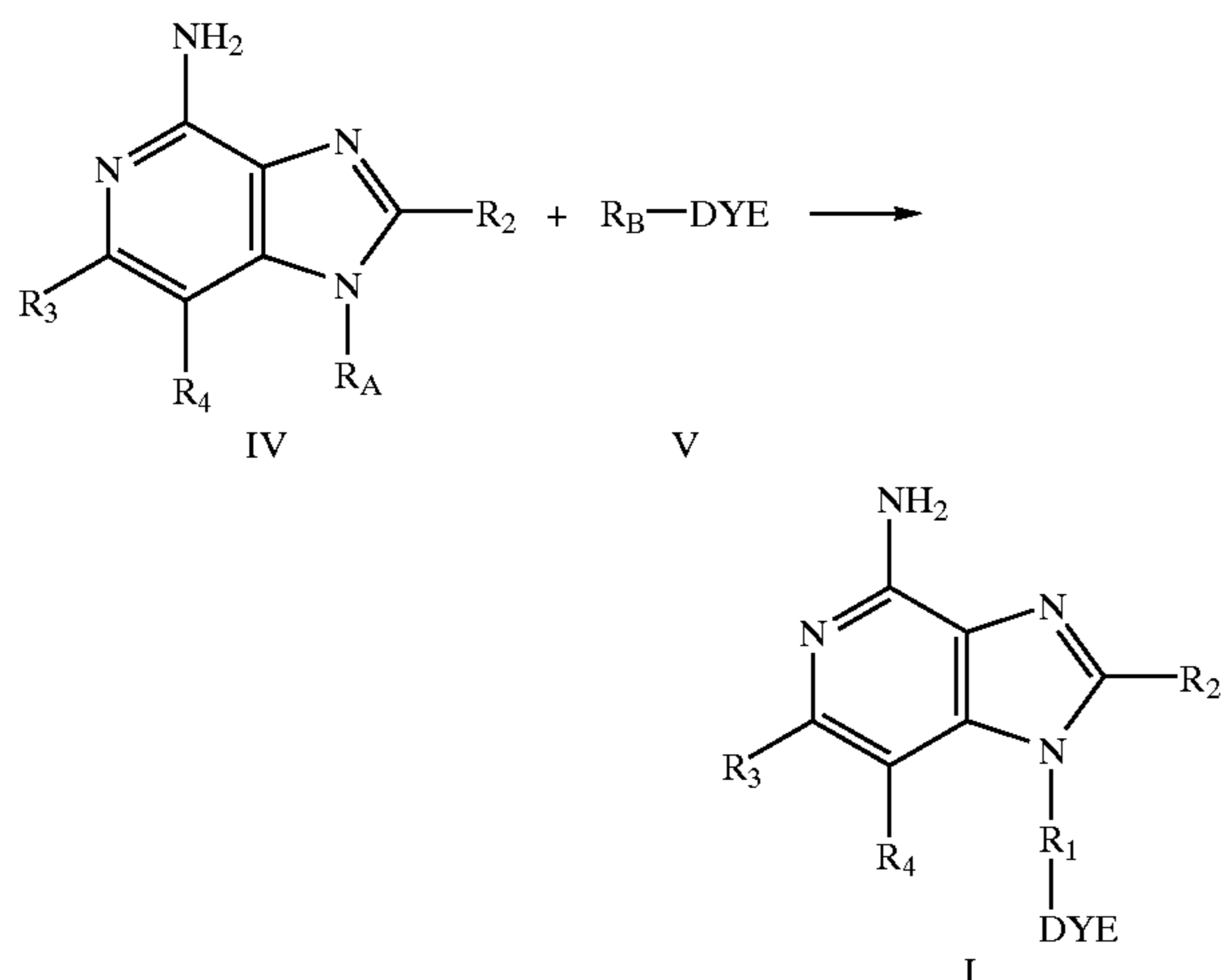
Reaction Scheme I
