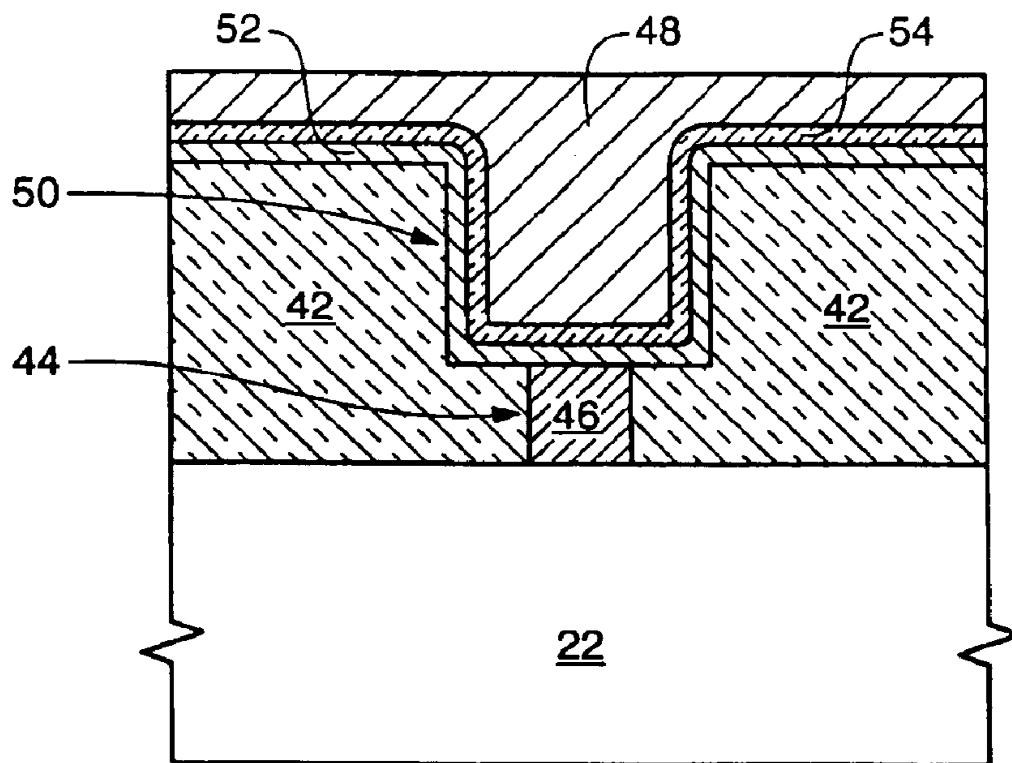
FIG. 8 (PRIOR ART)
