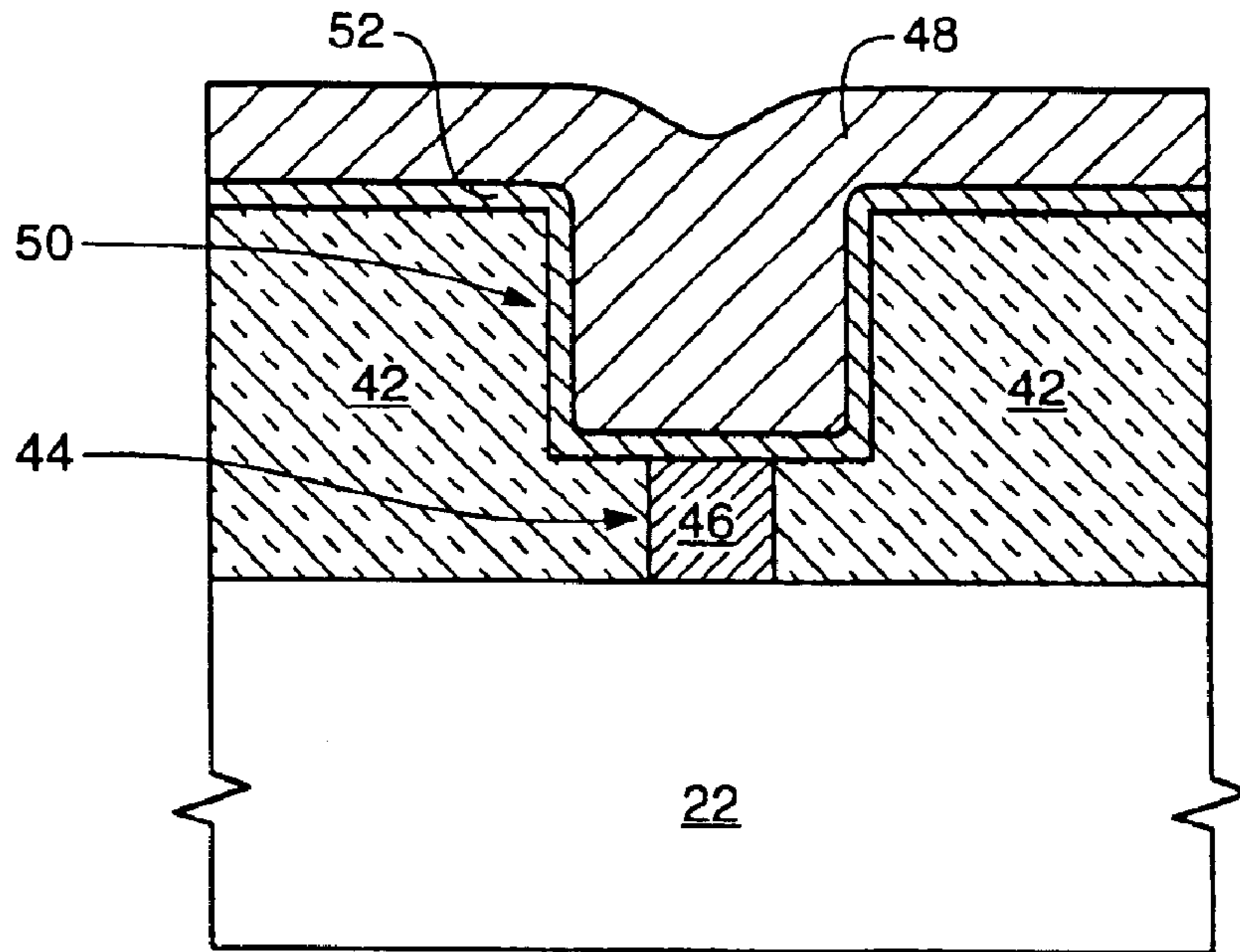
FIG. 7 (PRIOR ART)
