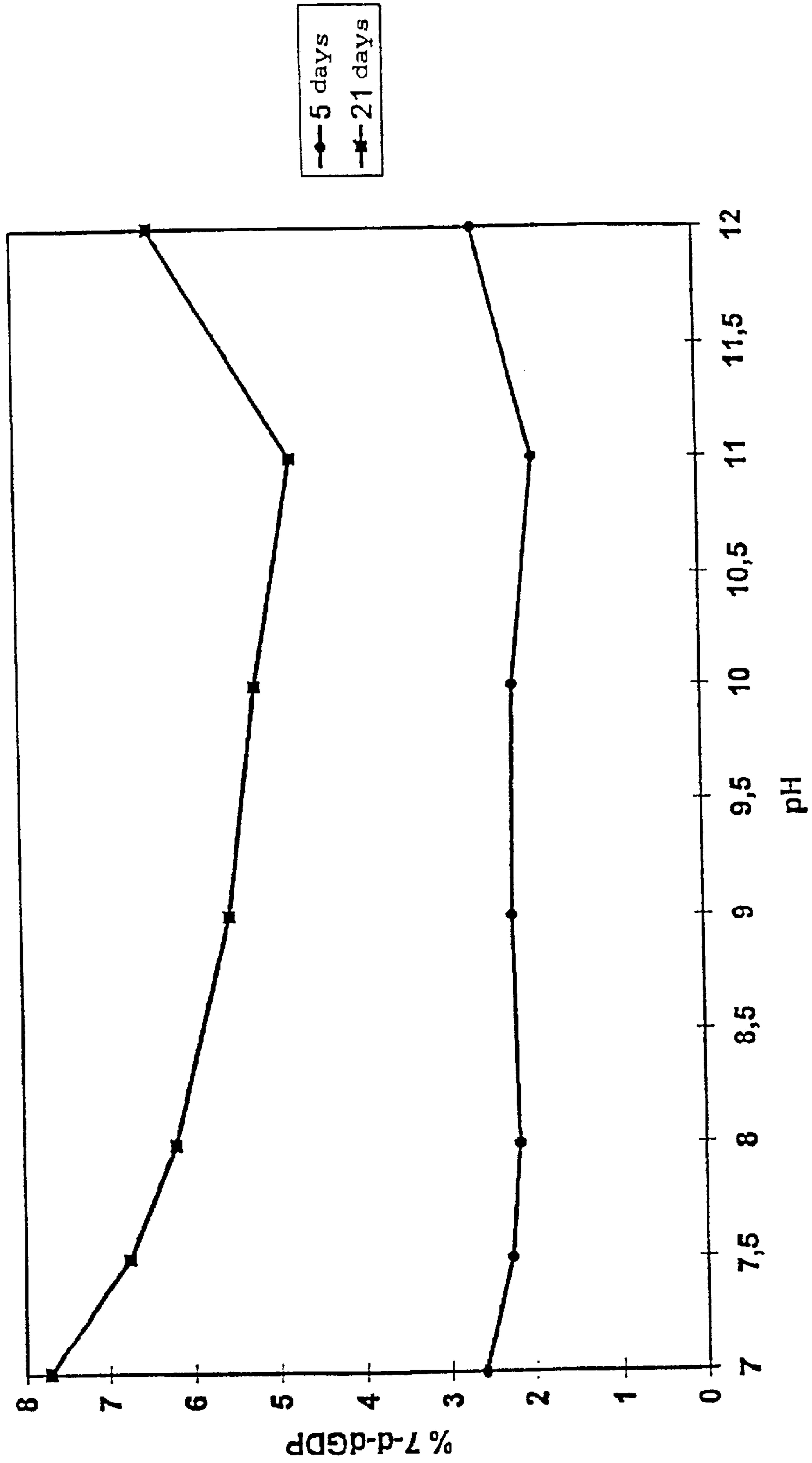
Fig. 12 stability 7-deaza-d-GTP
