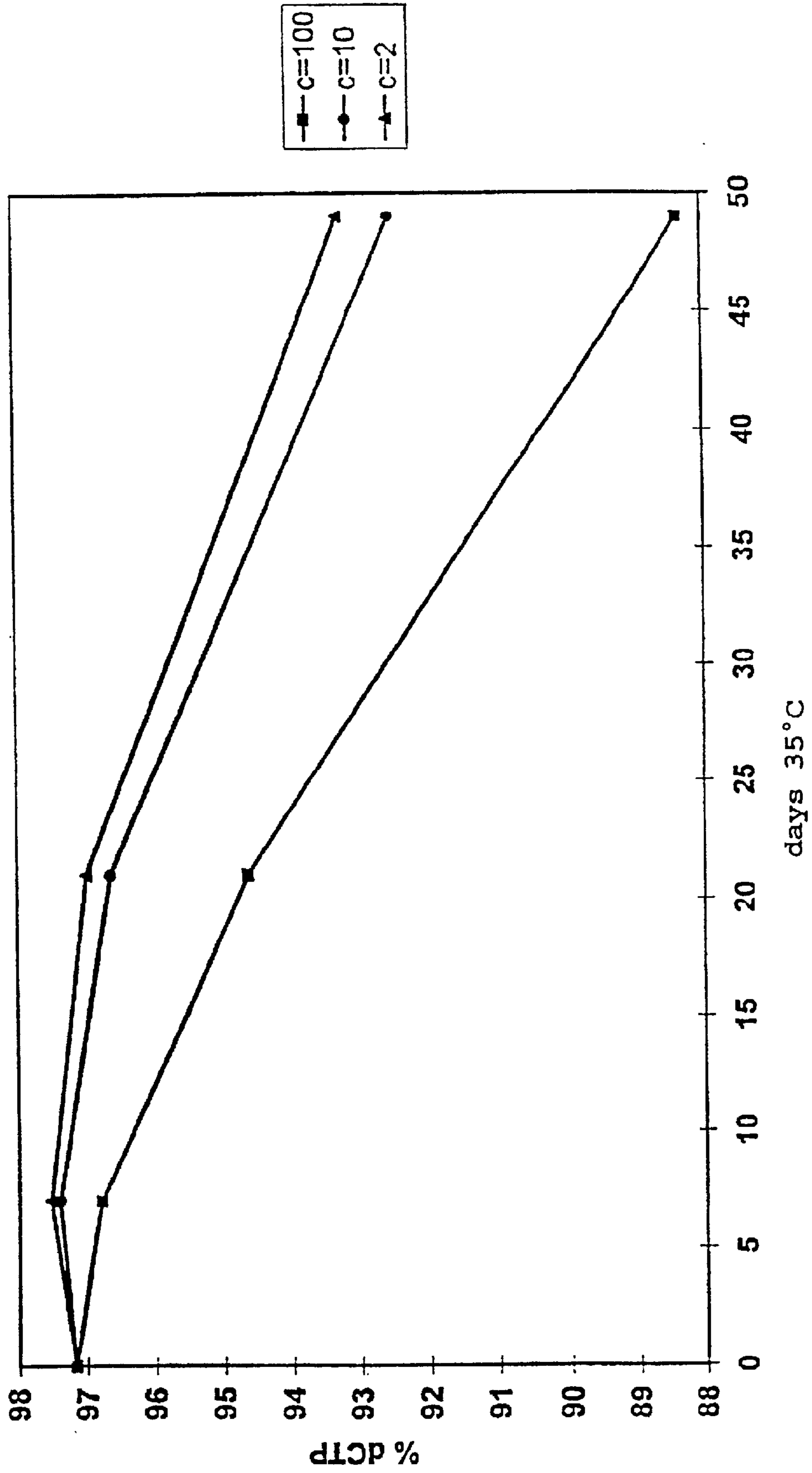
Fig. 15 Stability dCTP
