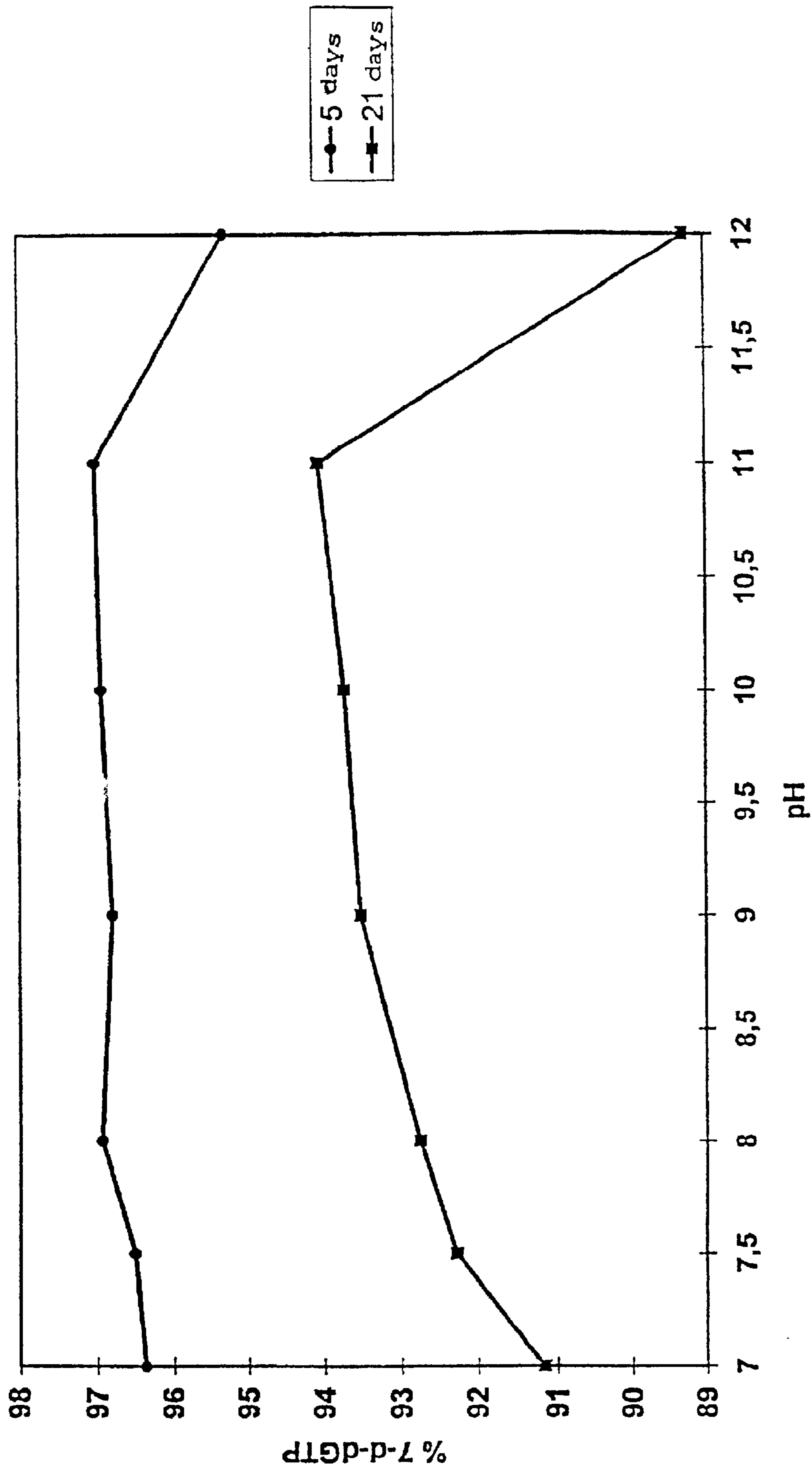
Fig. 11 stability 7-deaza-d-GTP
