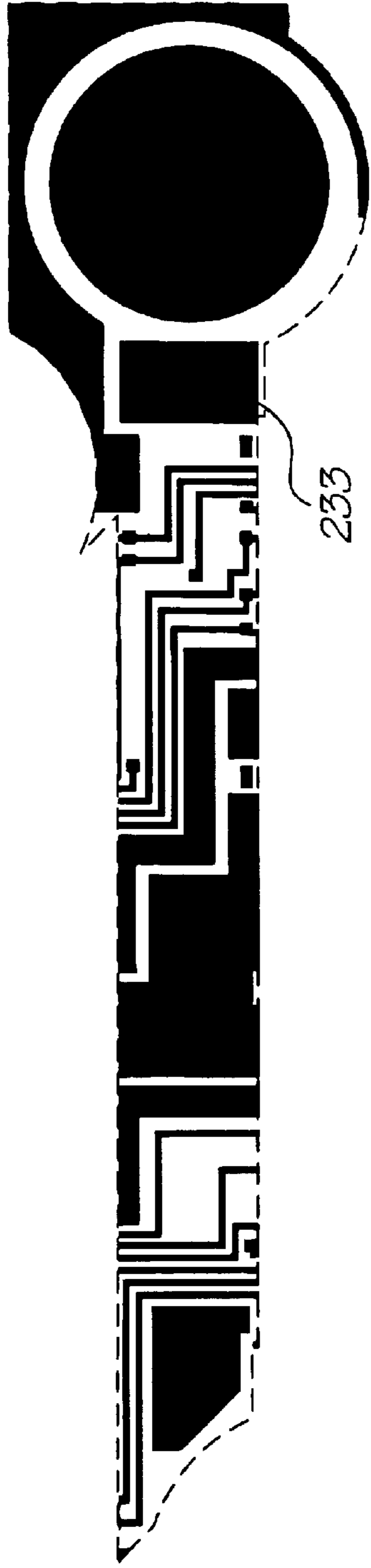
Metal 2 mask
