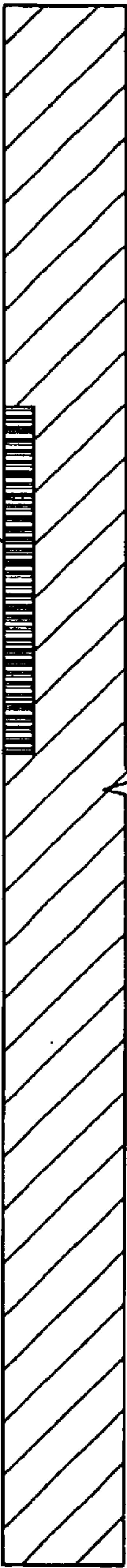
Implant N-Well
