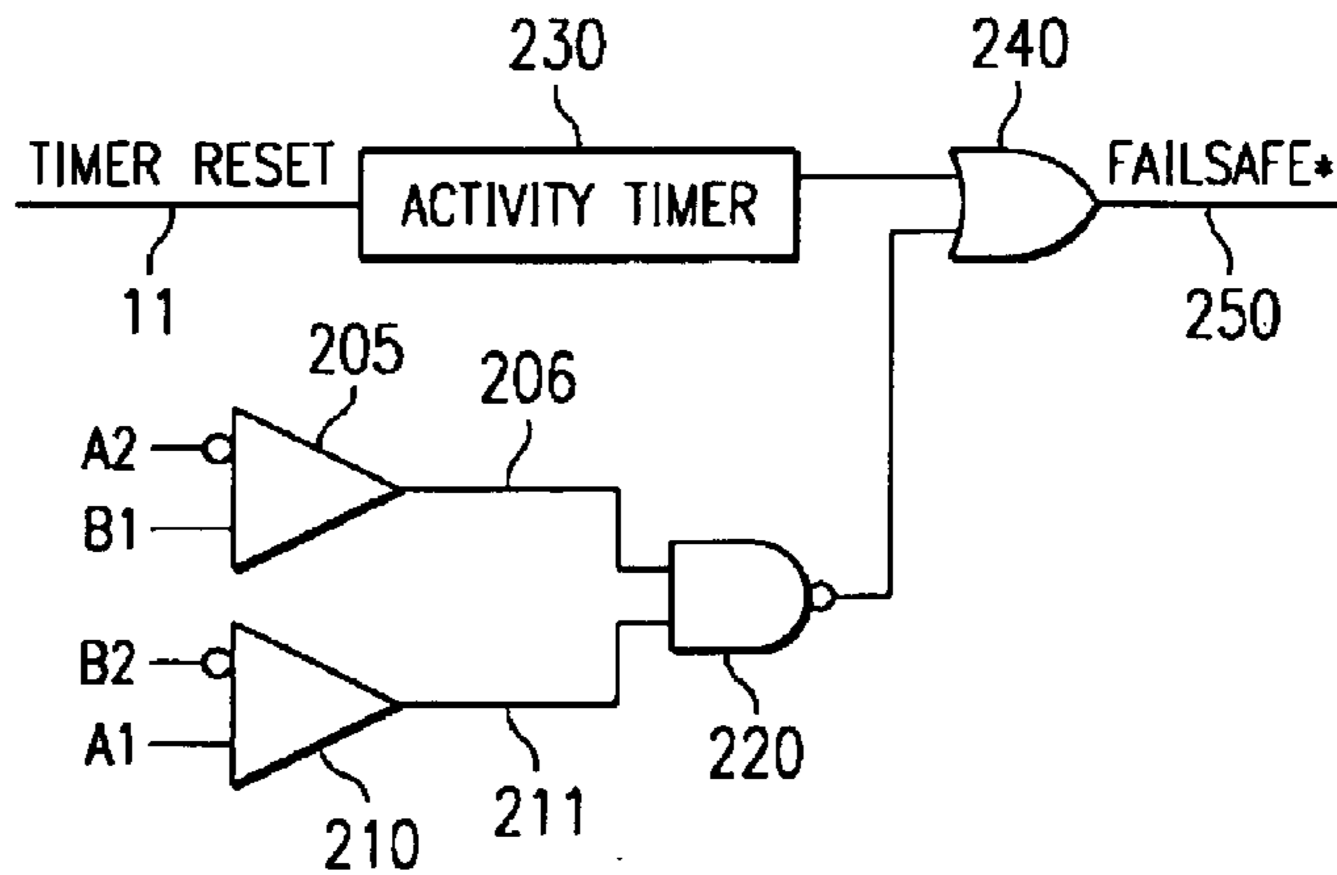
FIG. 2 (PRIOR ART)
