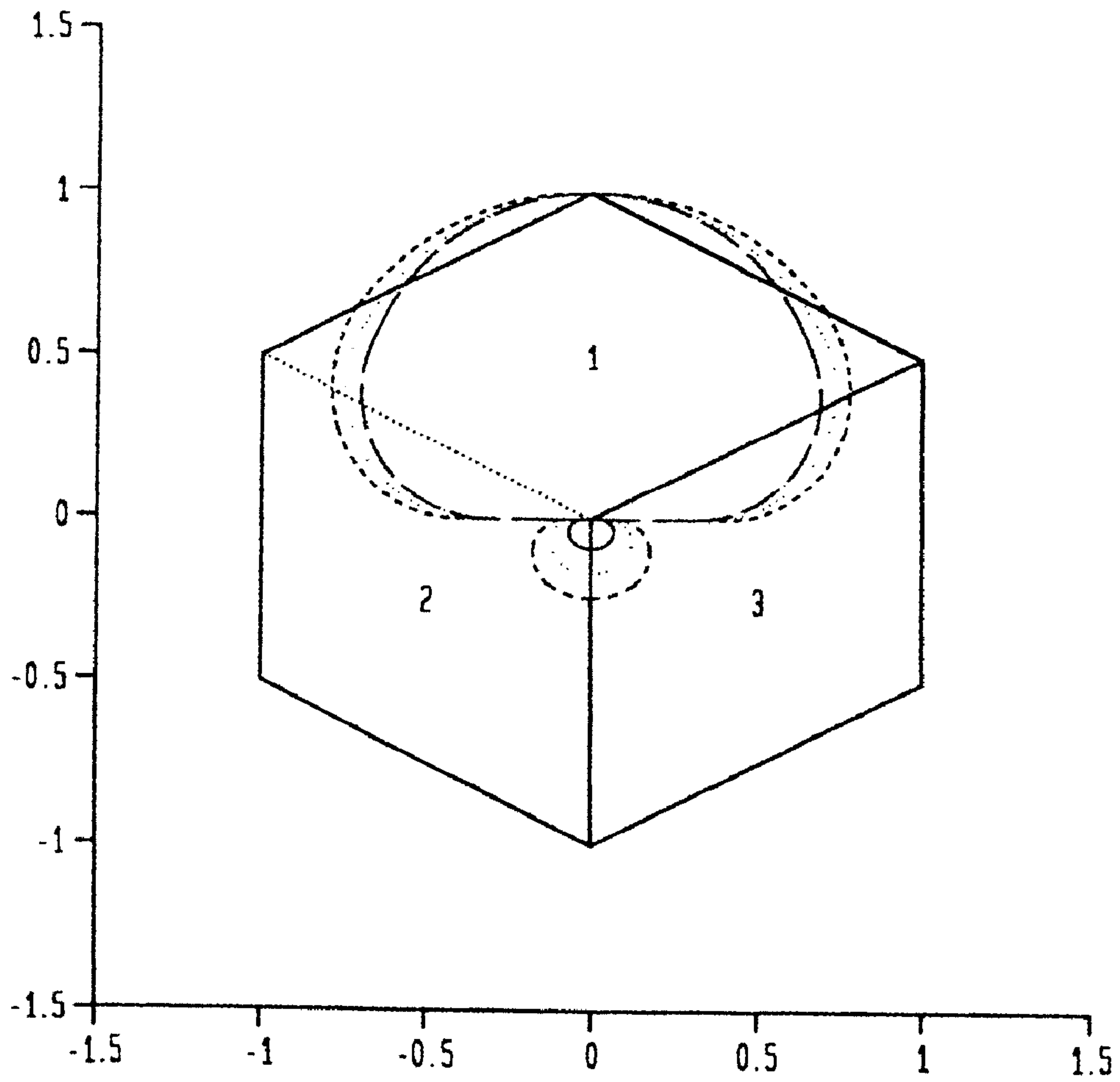
FIG. 3 (PRIOR ART)
