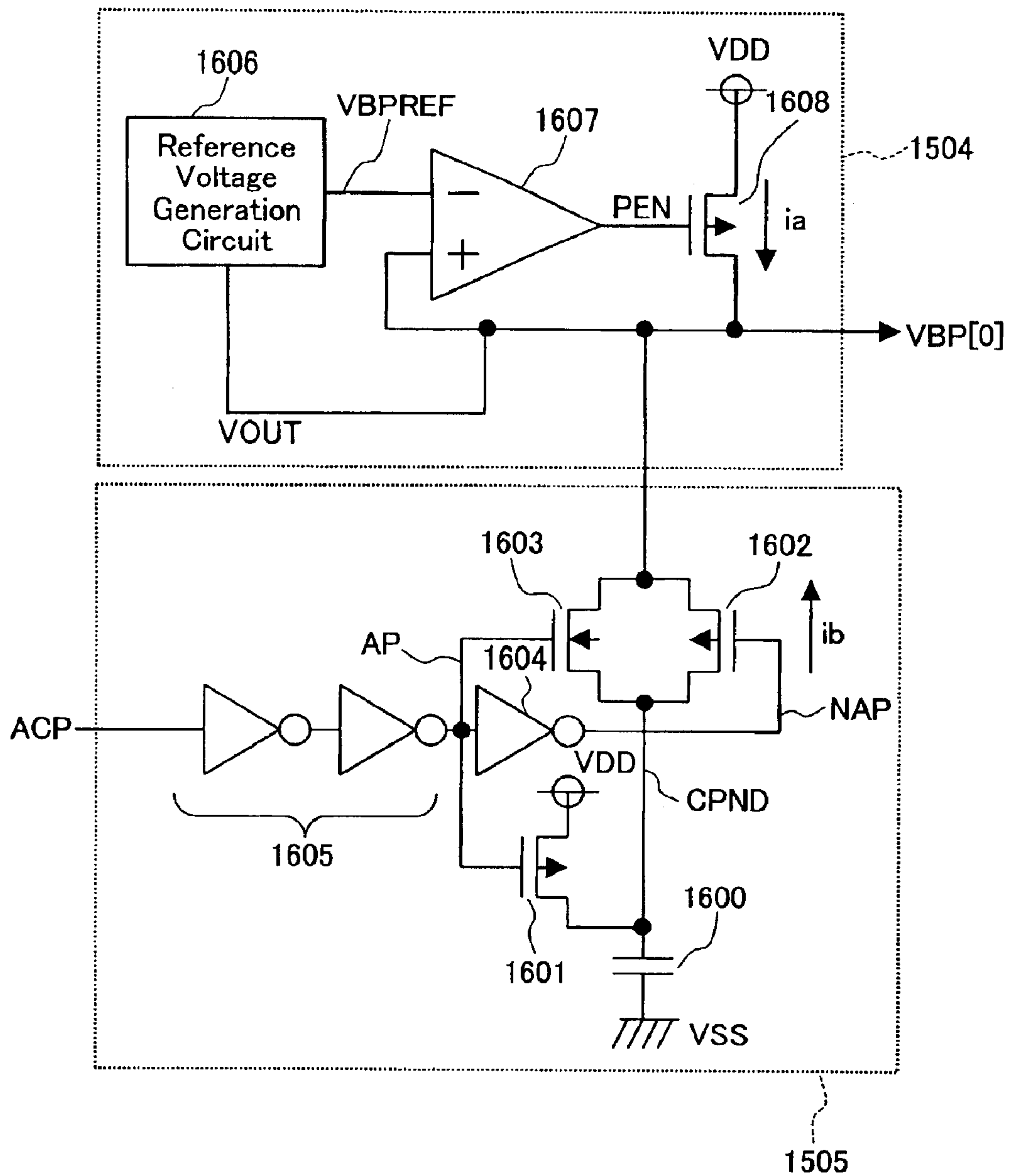
FIG.16 PRIOR ART
