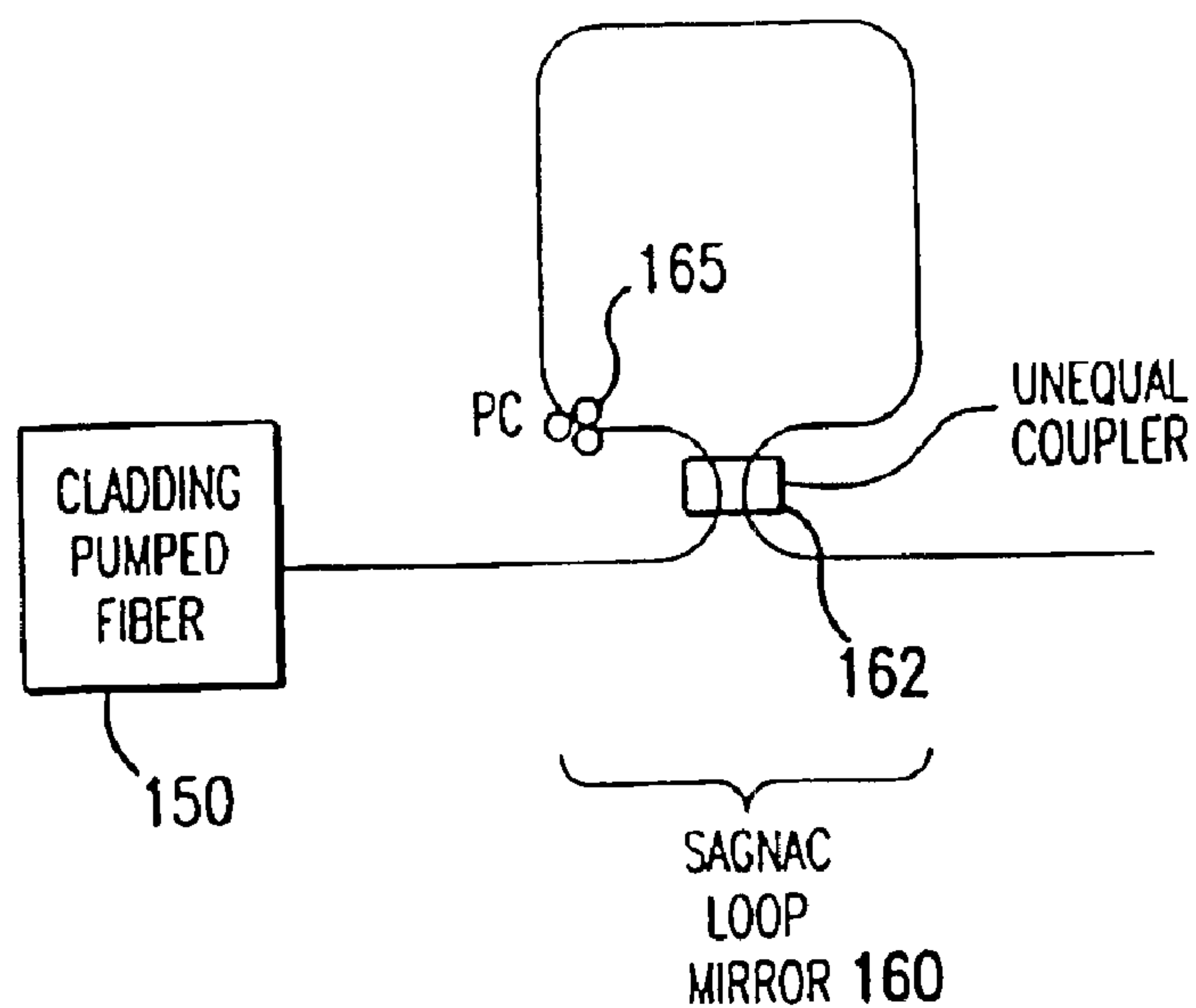
FIG.14b PRIOR ART
