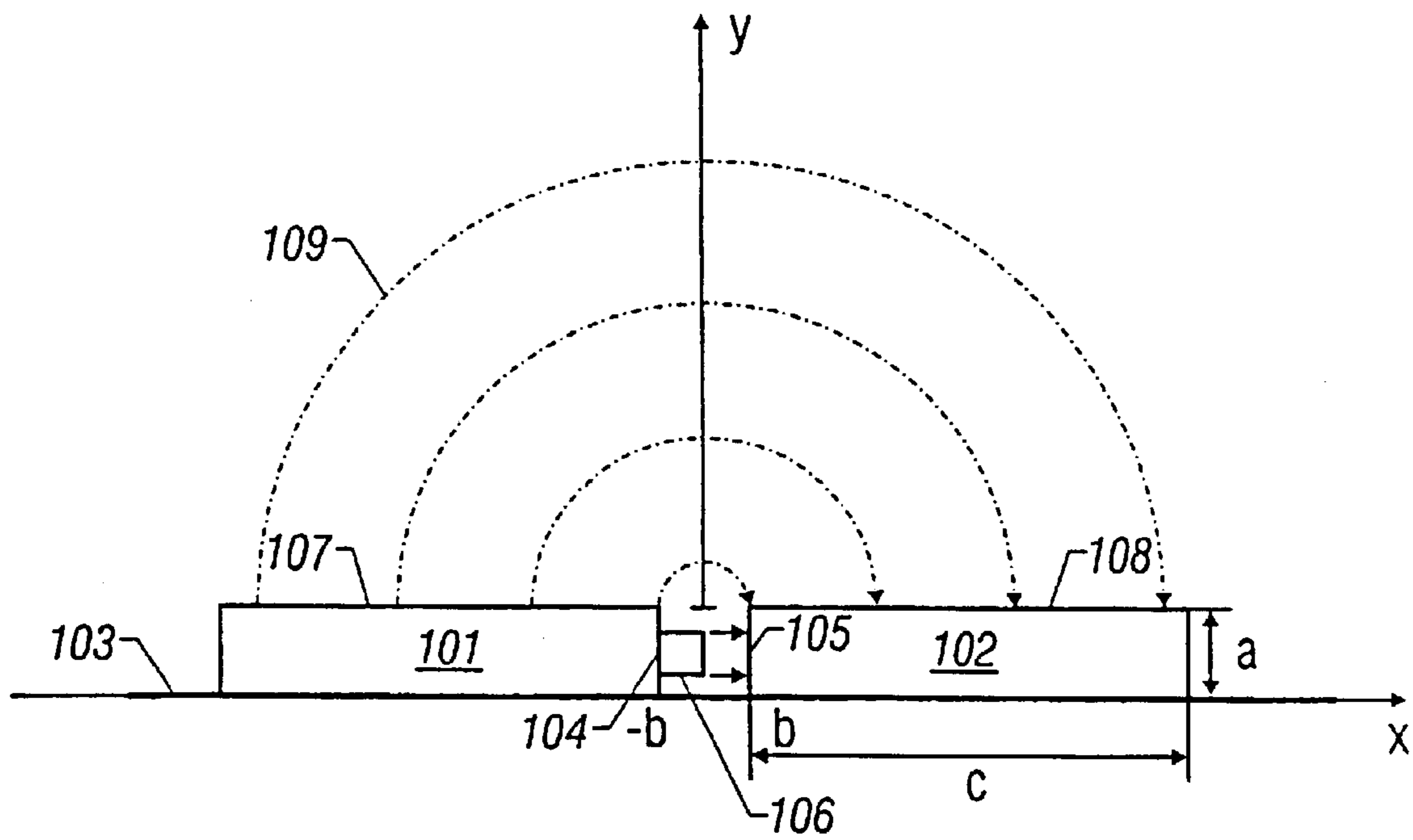
FIG. 1 (PRIOR ART)
