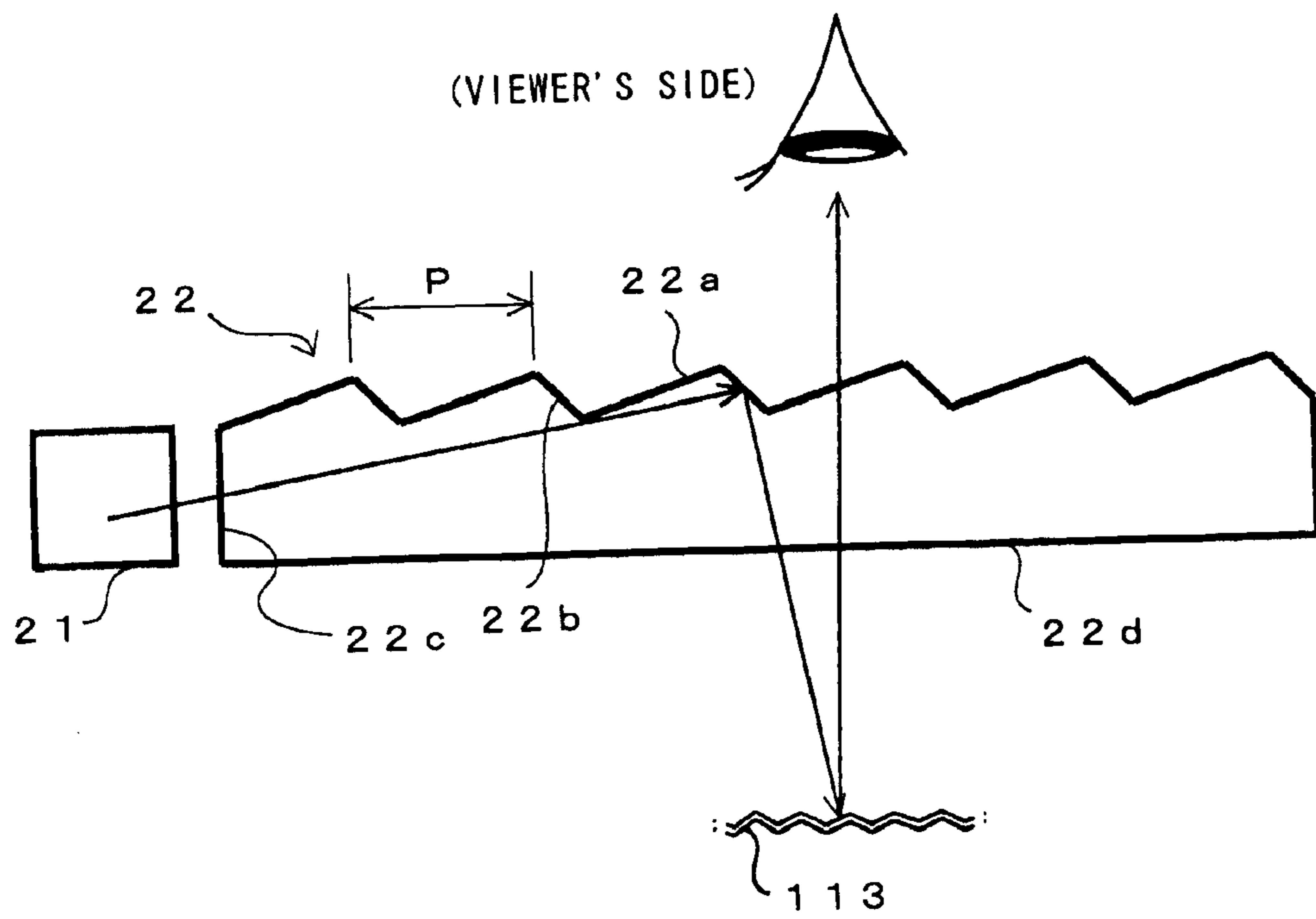
FIG. 3 PRIOR ART
