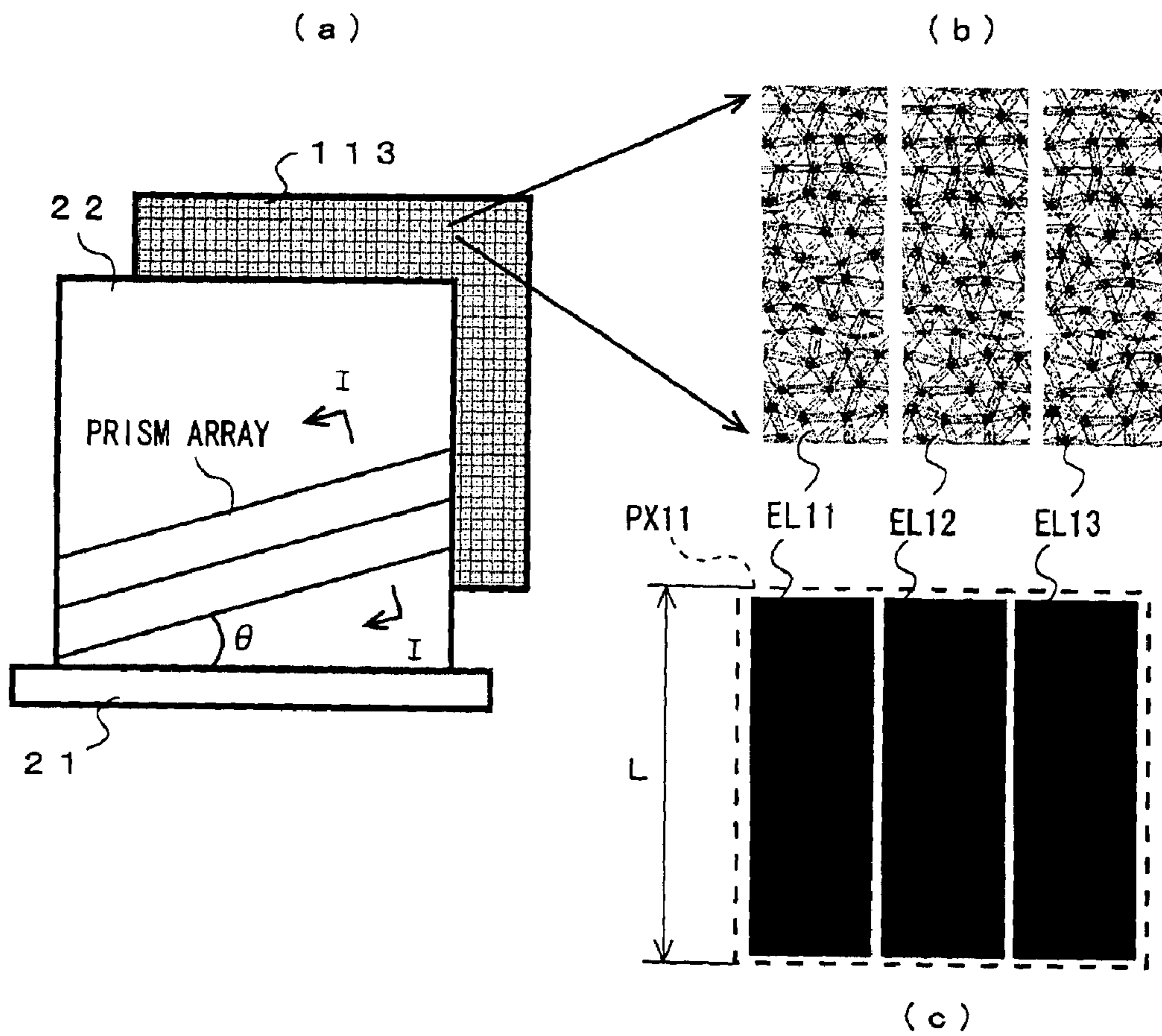
FIG. 2 PRIOR ART
