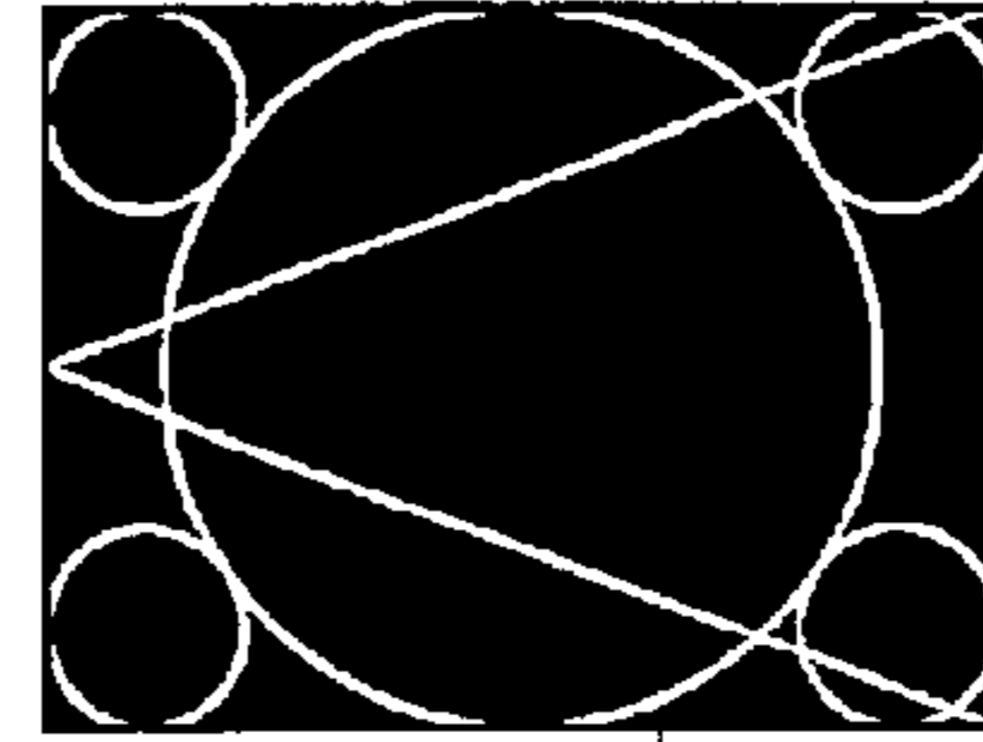
IMAGE A
