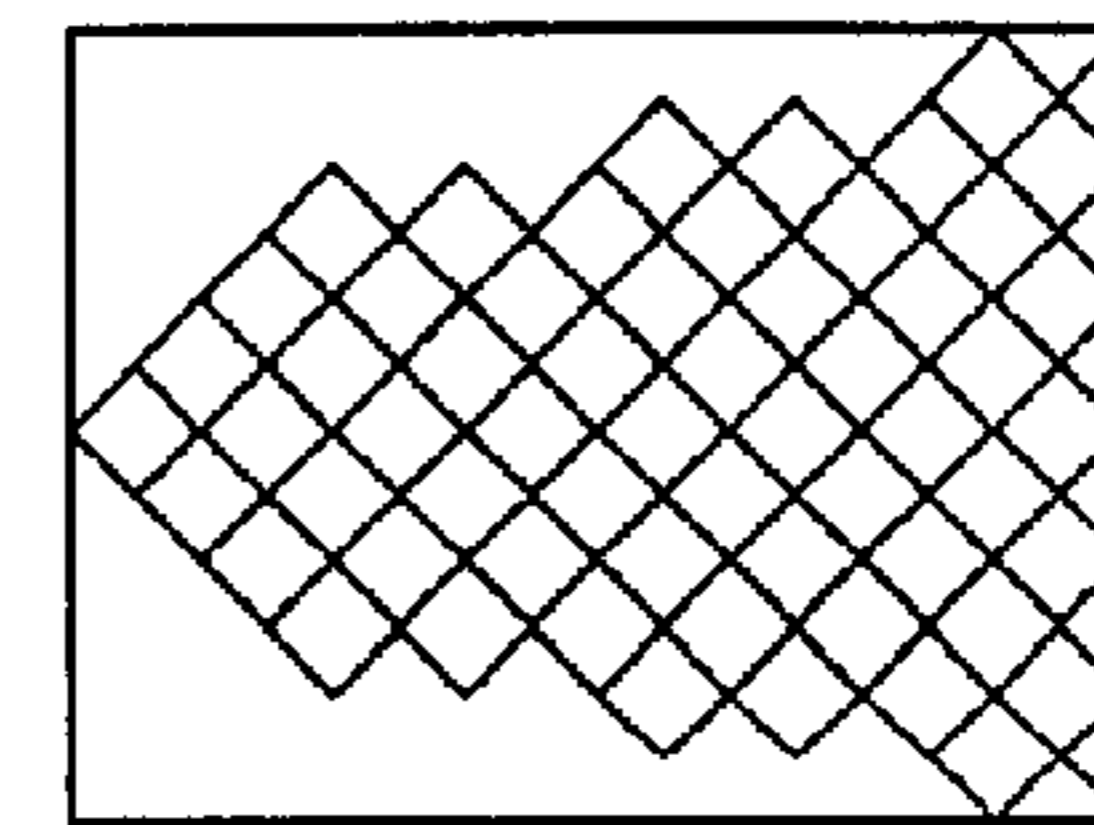
IMAGE B
