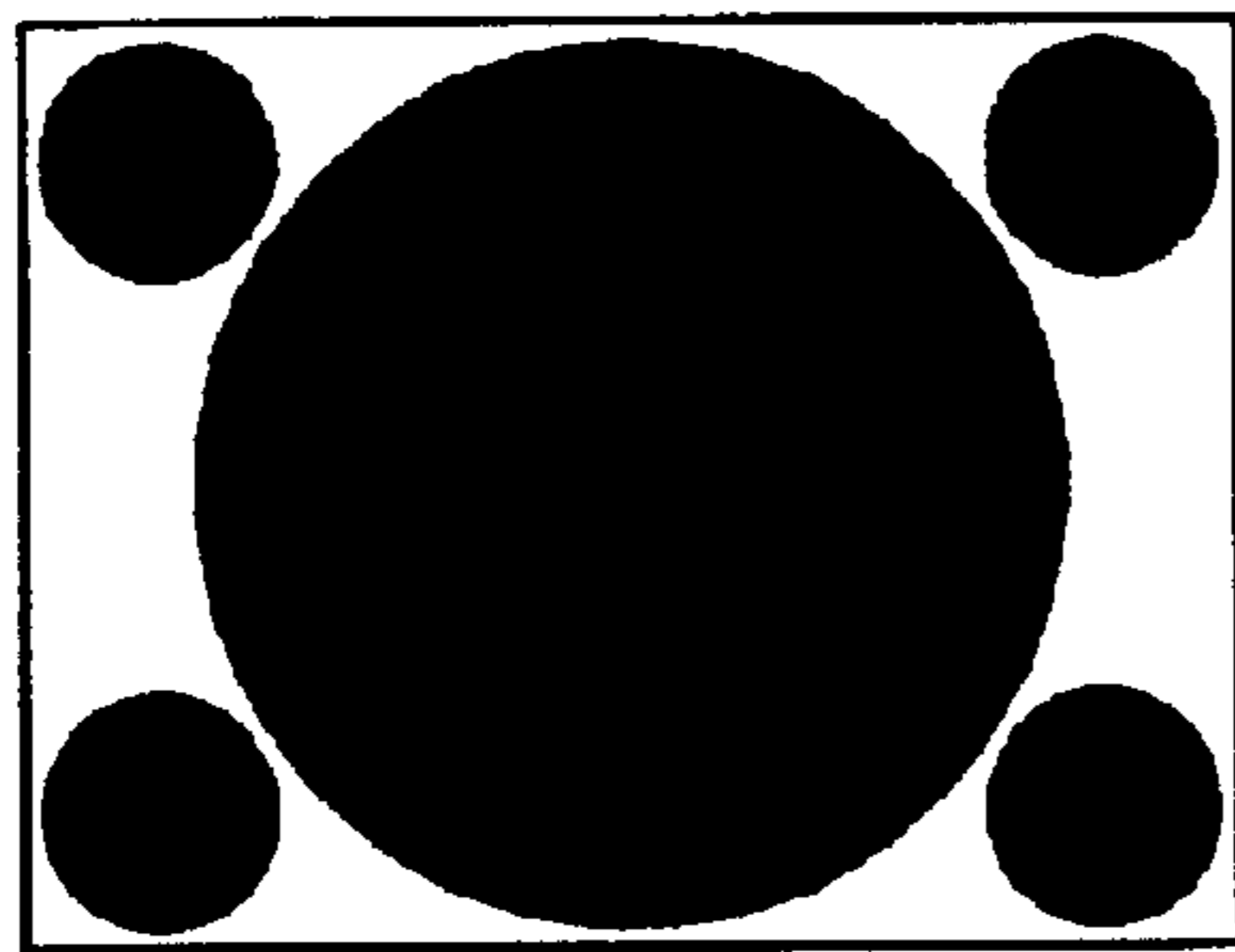
IMAGE A(128 × 96)
