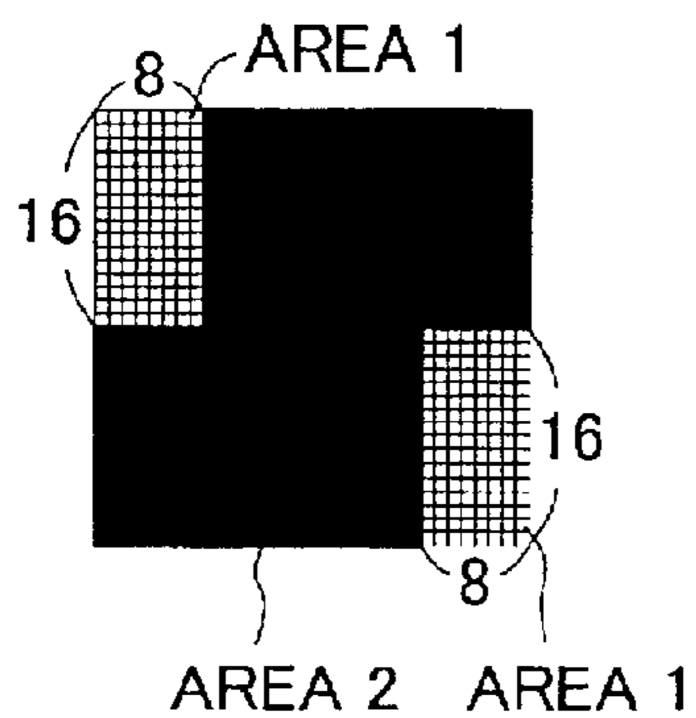
MASK 4 (32 × 32)
