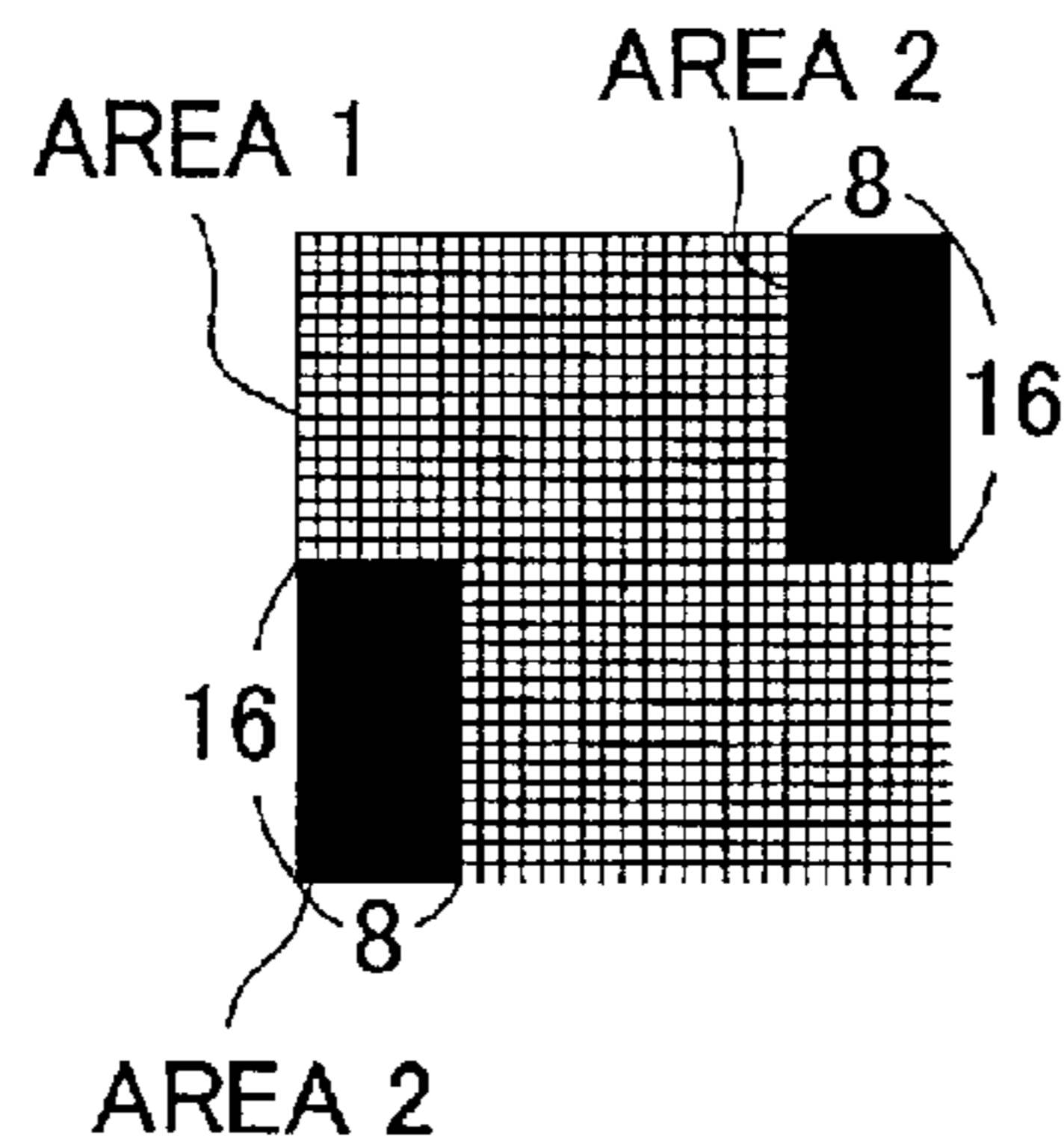
MASK 2 (32 × 32)
