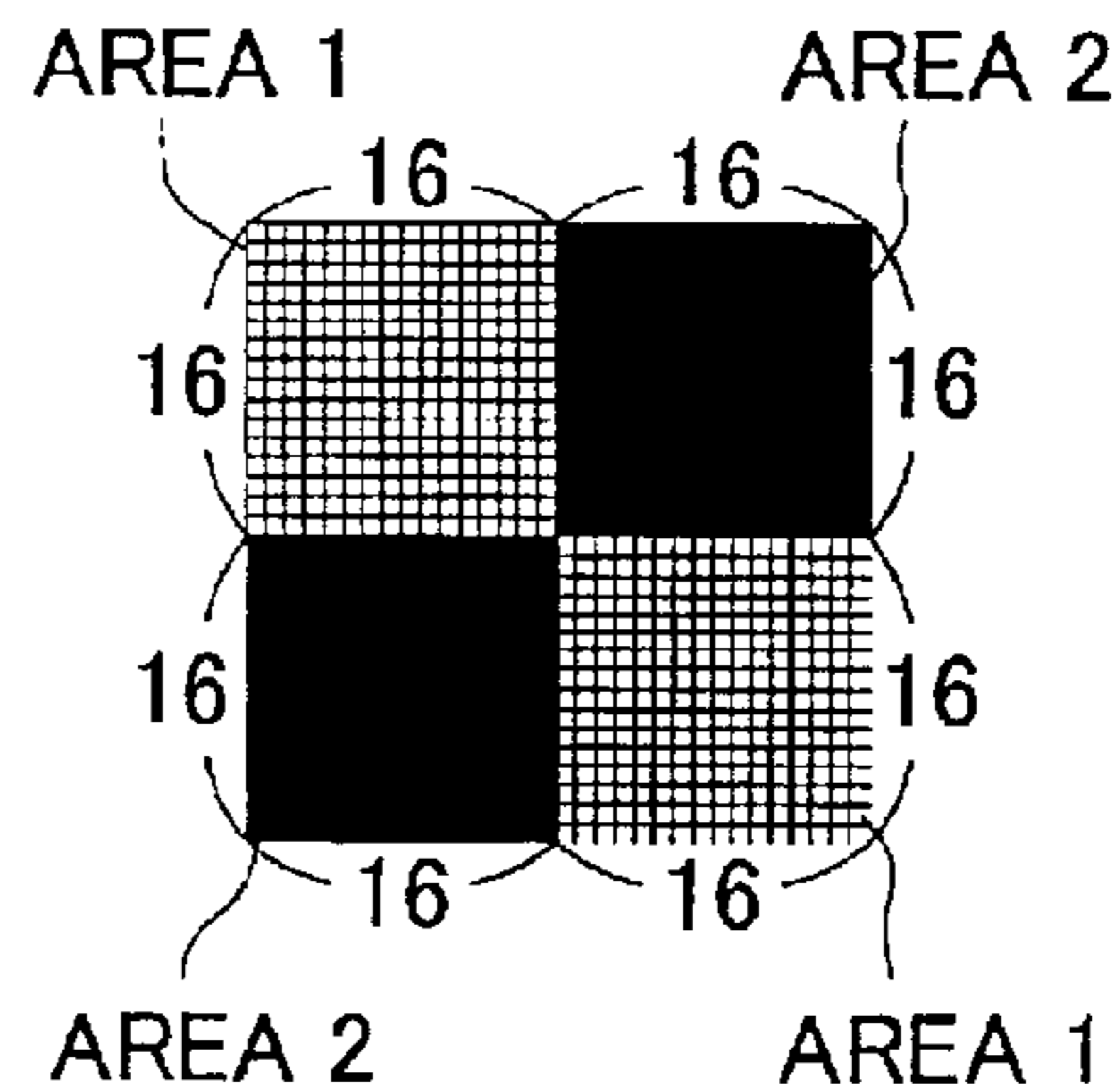
MASK 3 (32 × 32)
