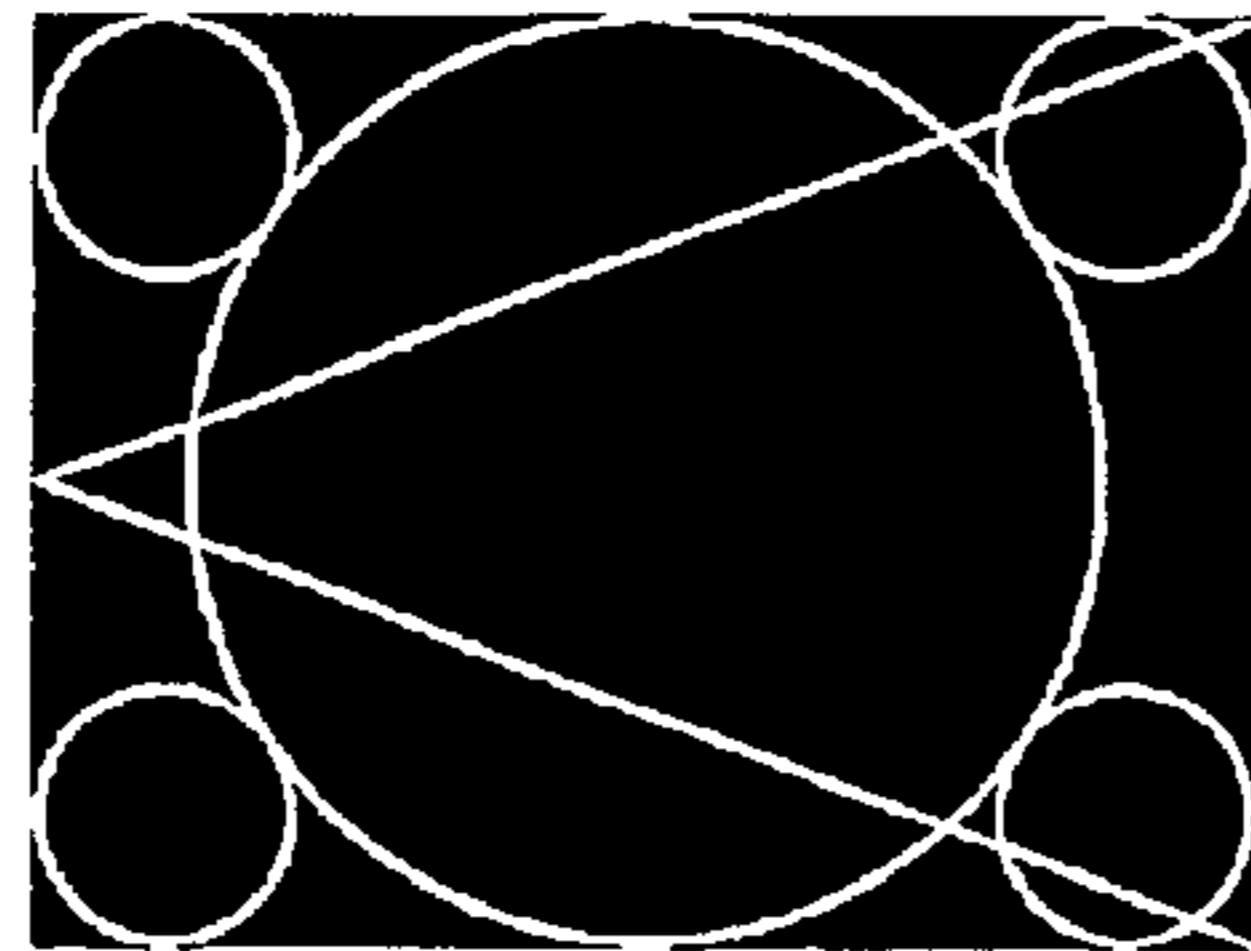
IMAGE A(128 × 96)
