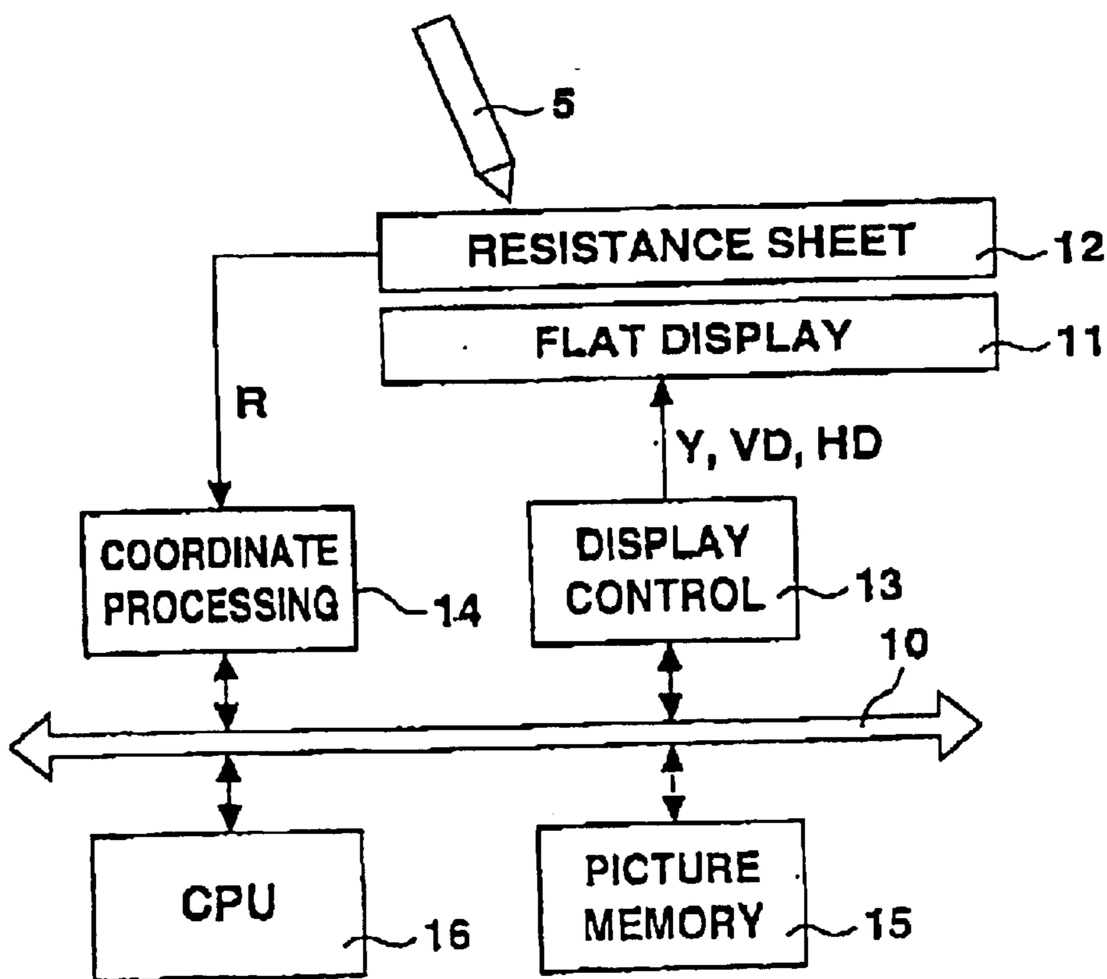
Fig. 6 PRIOR ART
