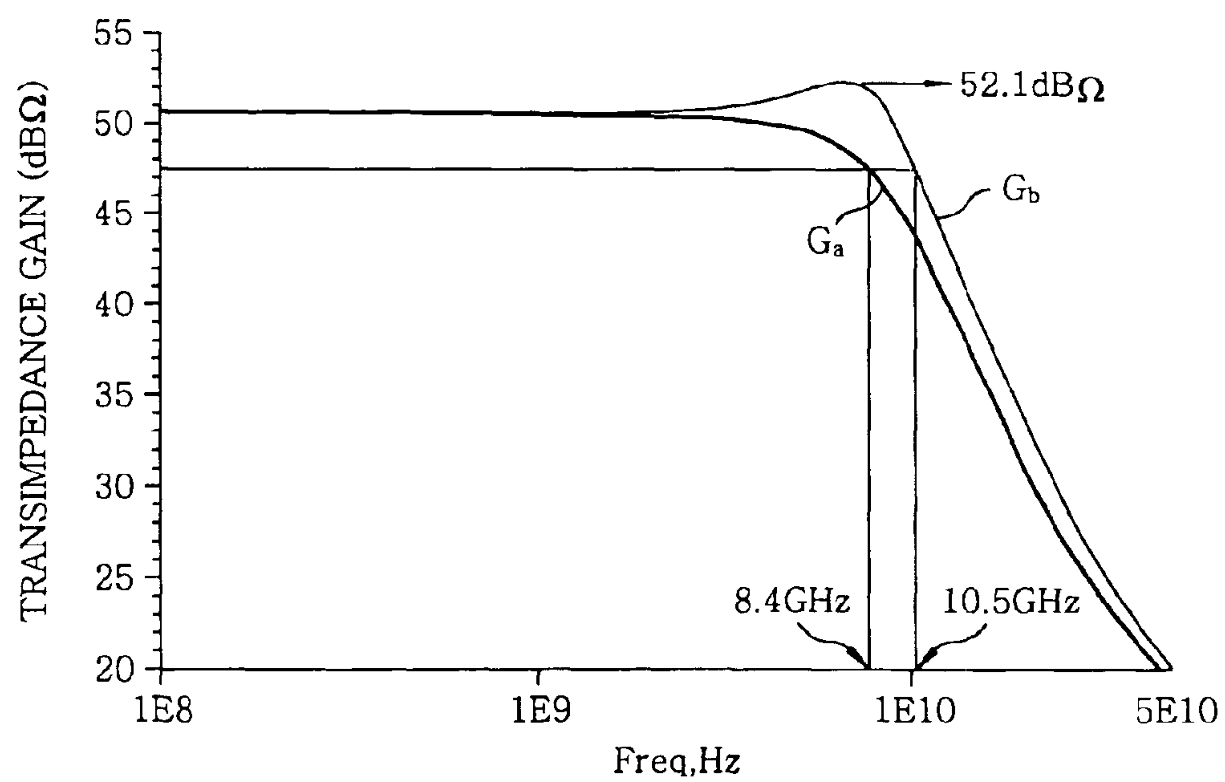
FIG. 2 (PRIOR ART)
