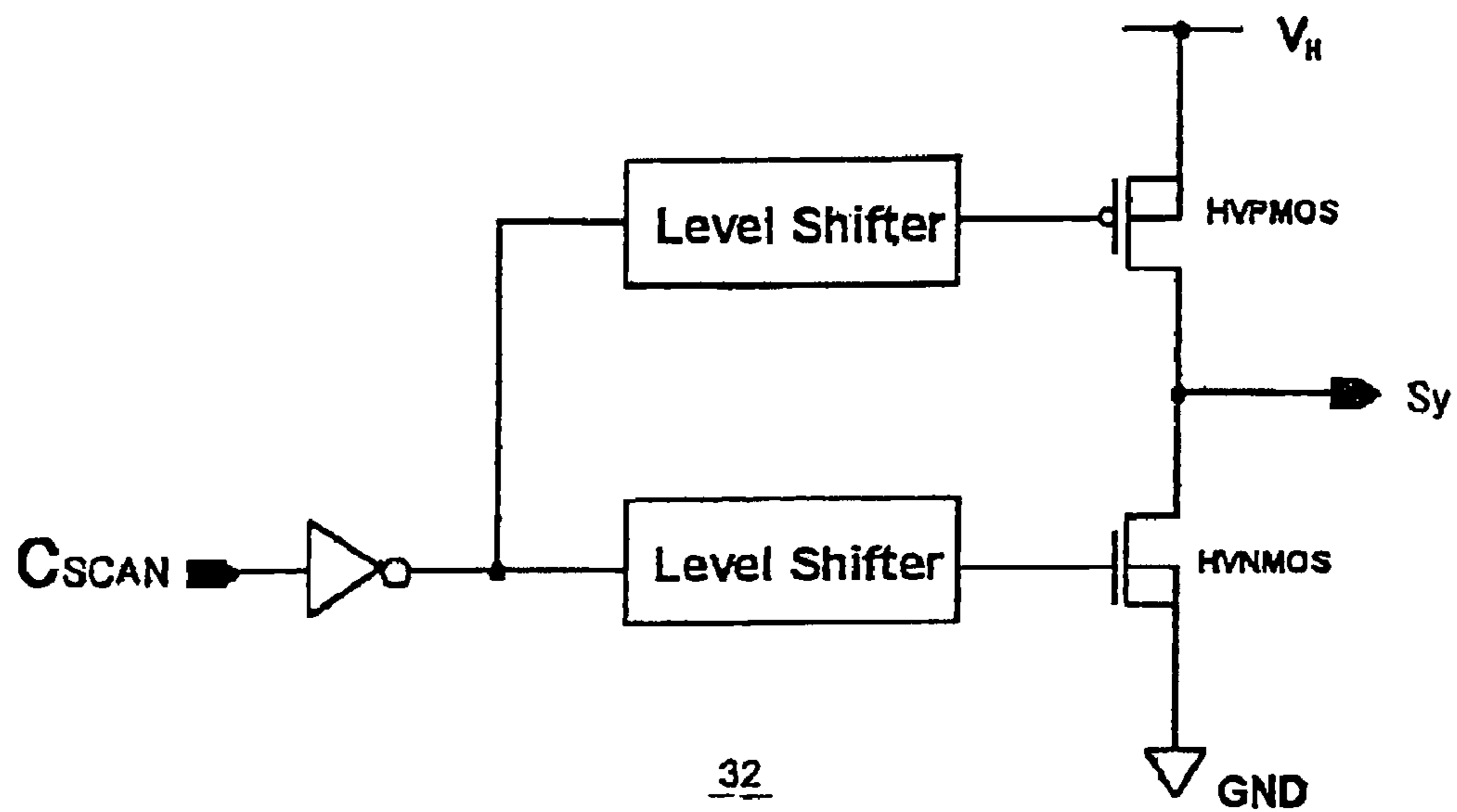
CONVENTIONAL ART
