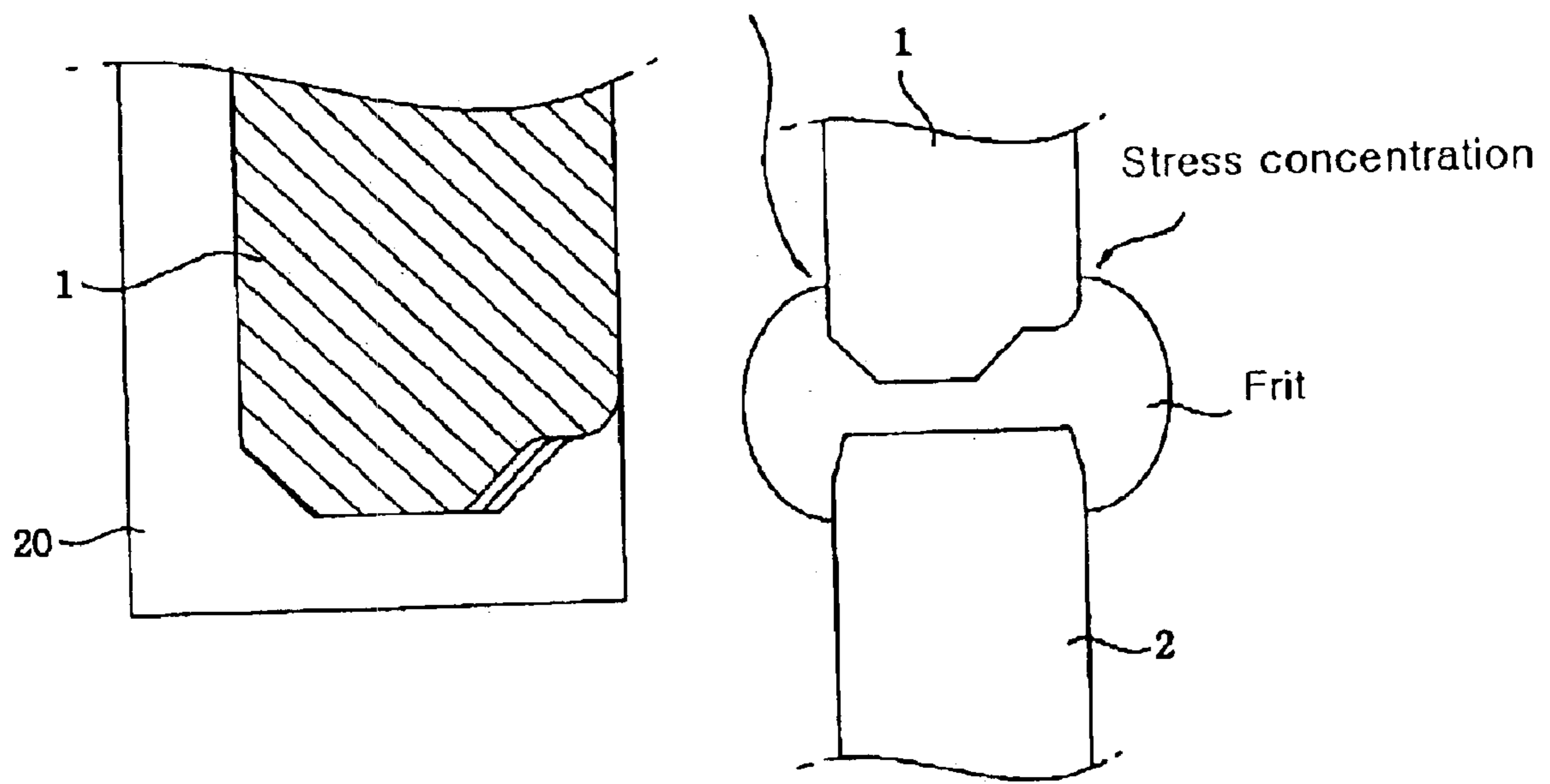
Fig. 6 Stress concentration
