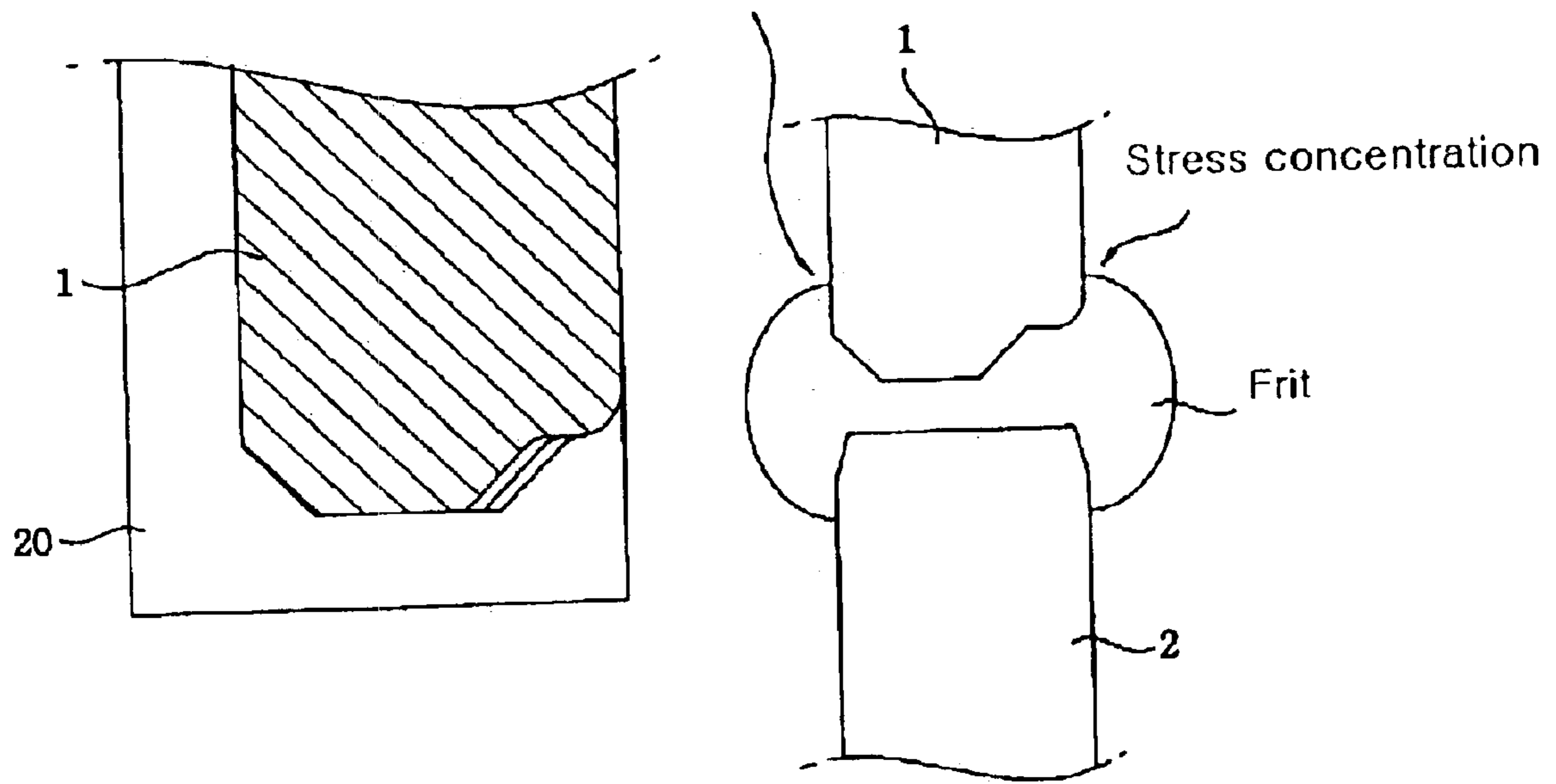
Fig. 6 Stress concentration
