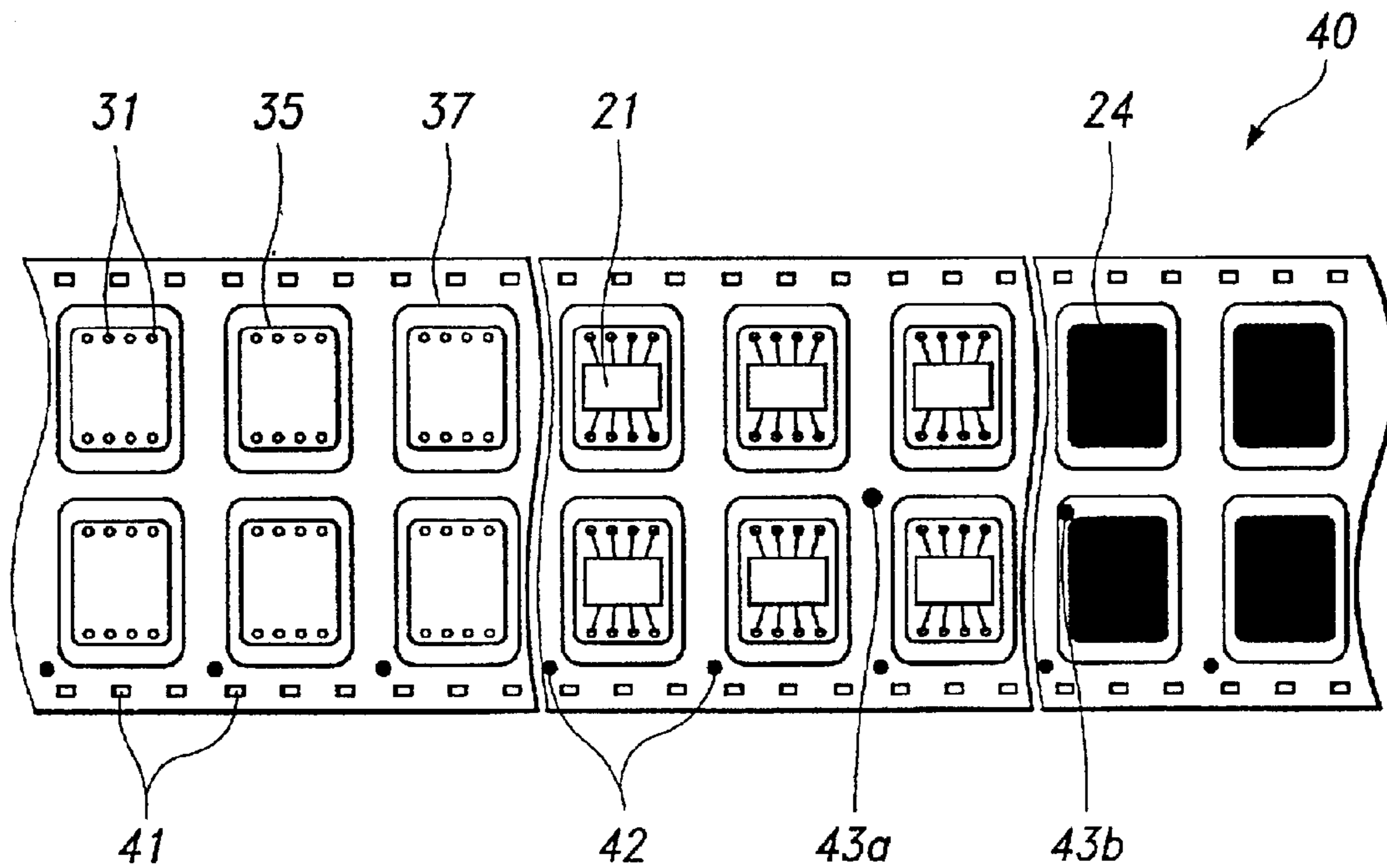
FIG. 5 (Prior Art)
