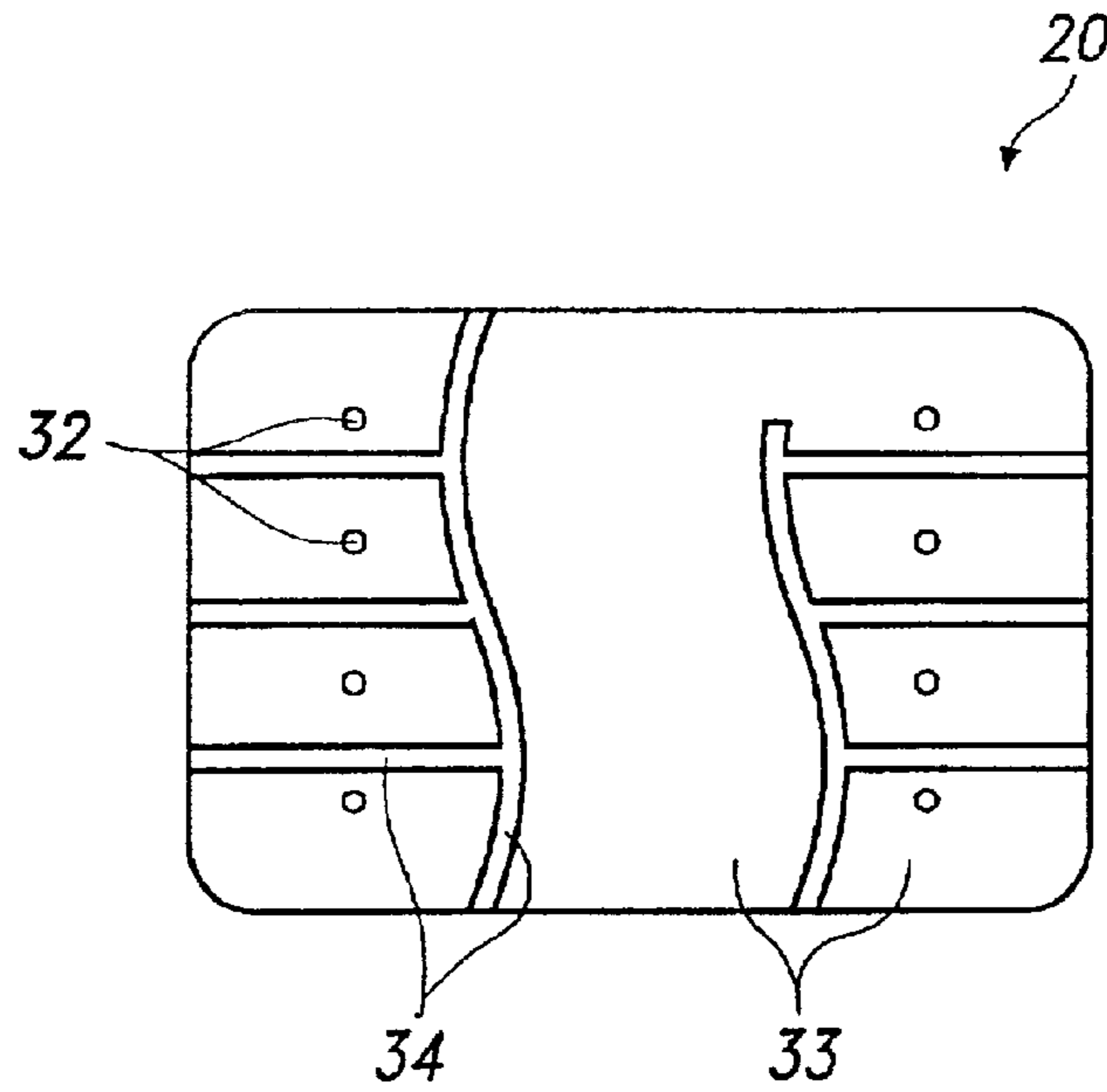
FIG. 4 (Prior Art)
