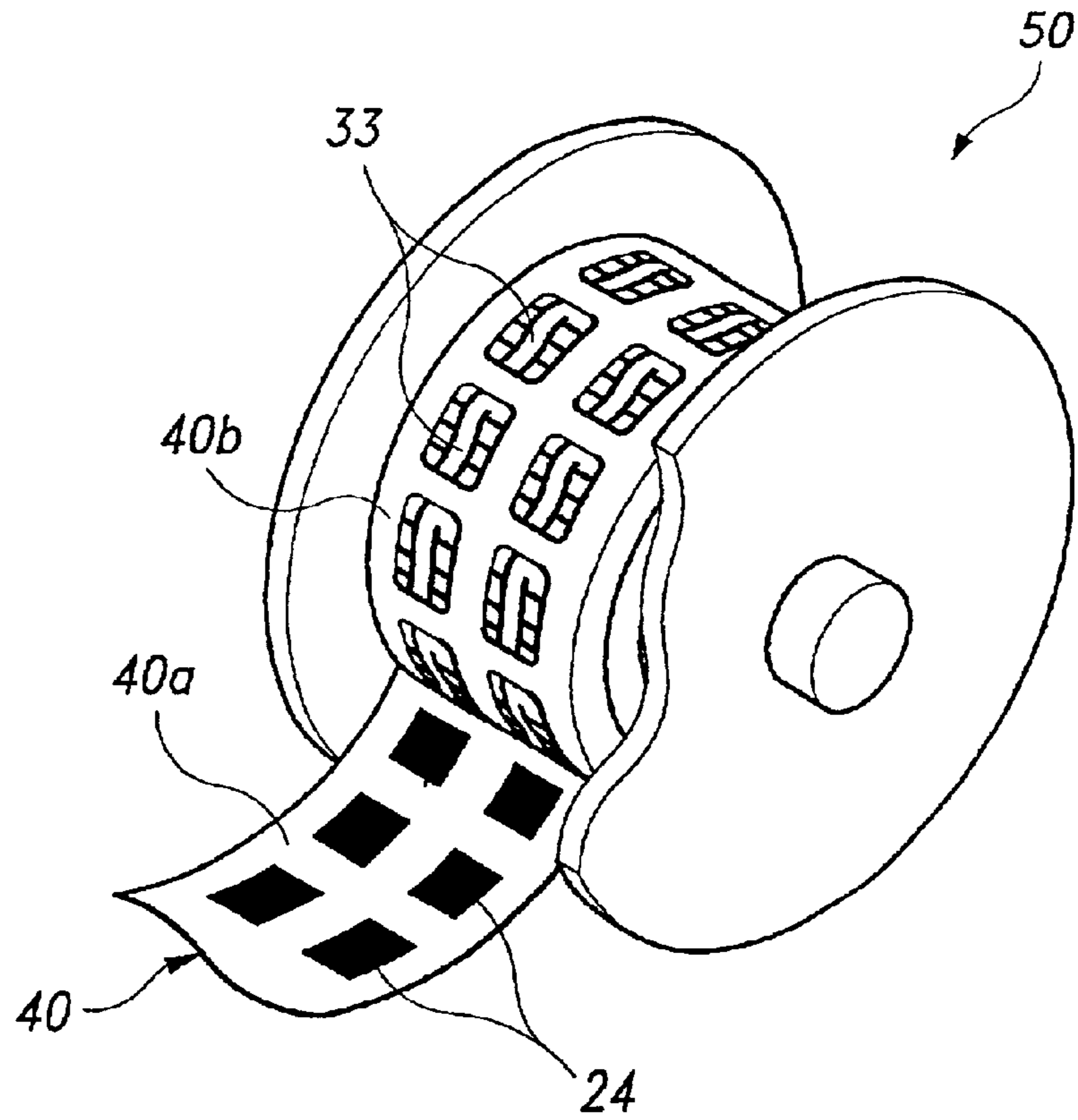
FIG. 6 (Prior Art)
