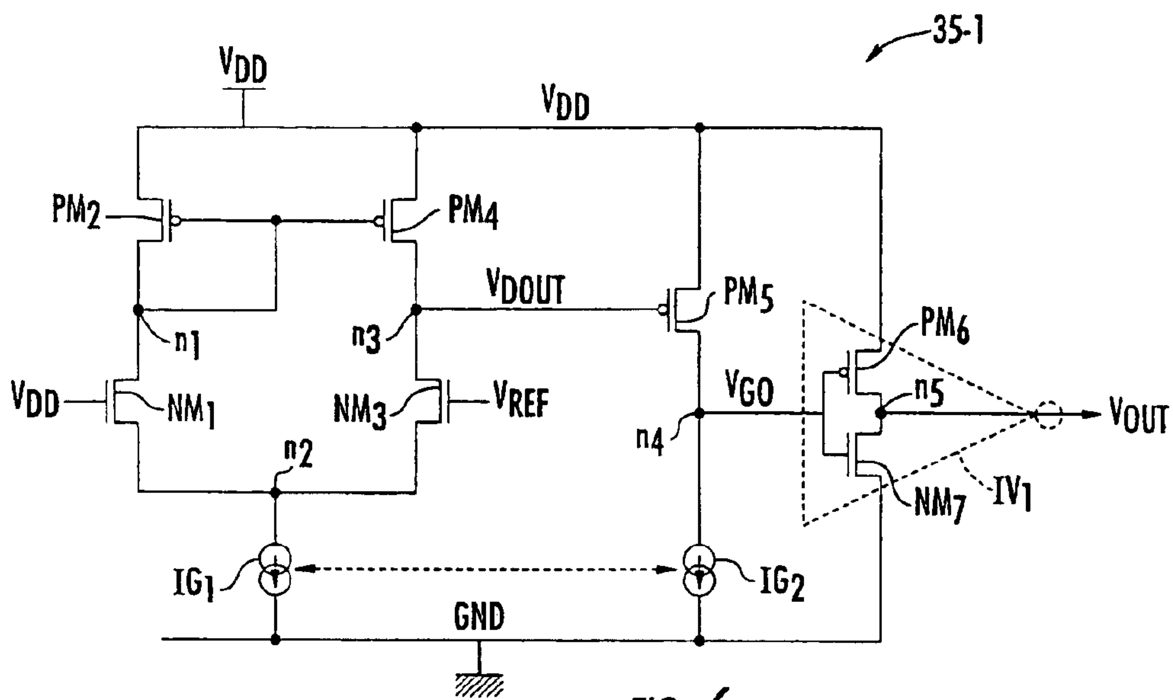
FIG. 6. PRIOR ART
