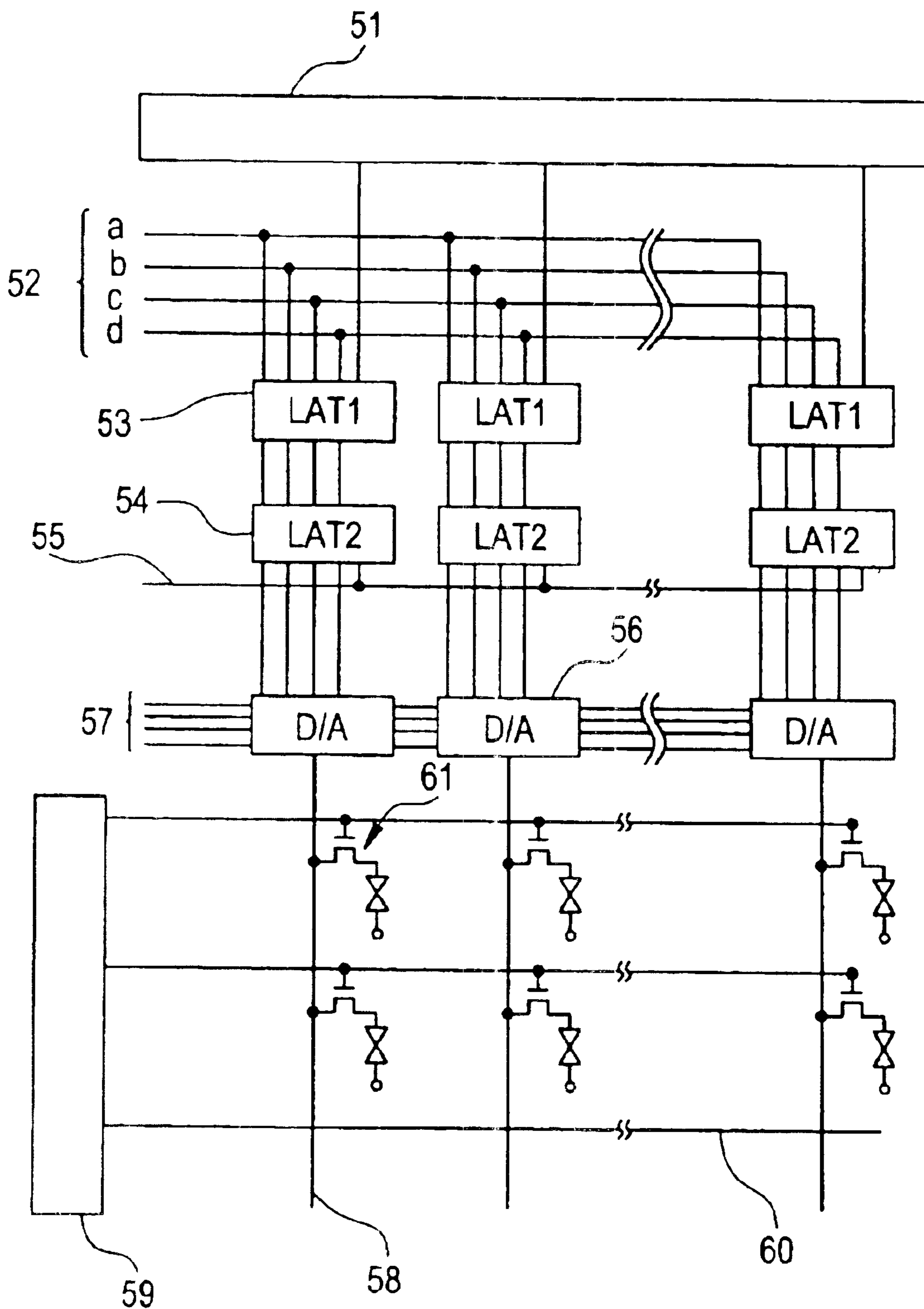
FIG. 34 PRIOR ART
