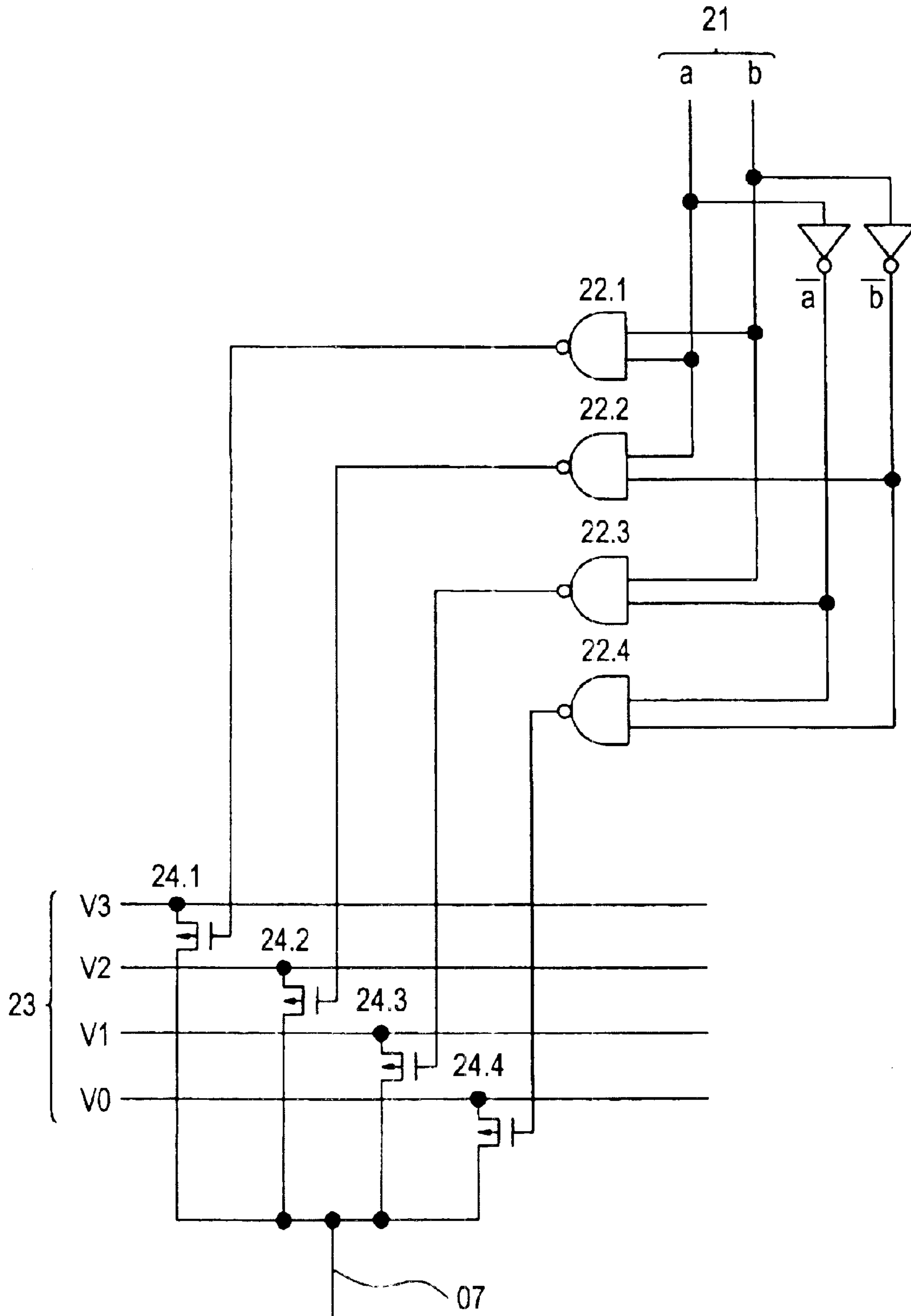
FIG. 32 PRIOR ART
