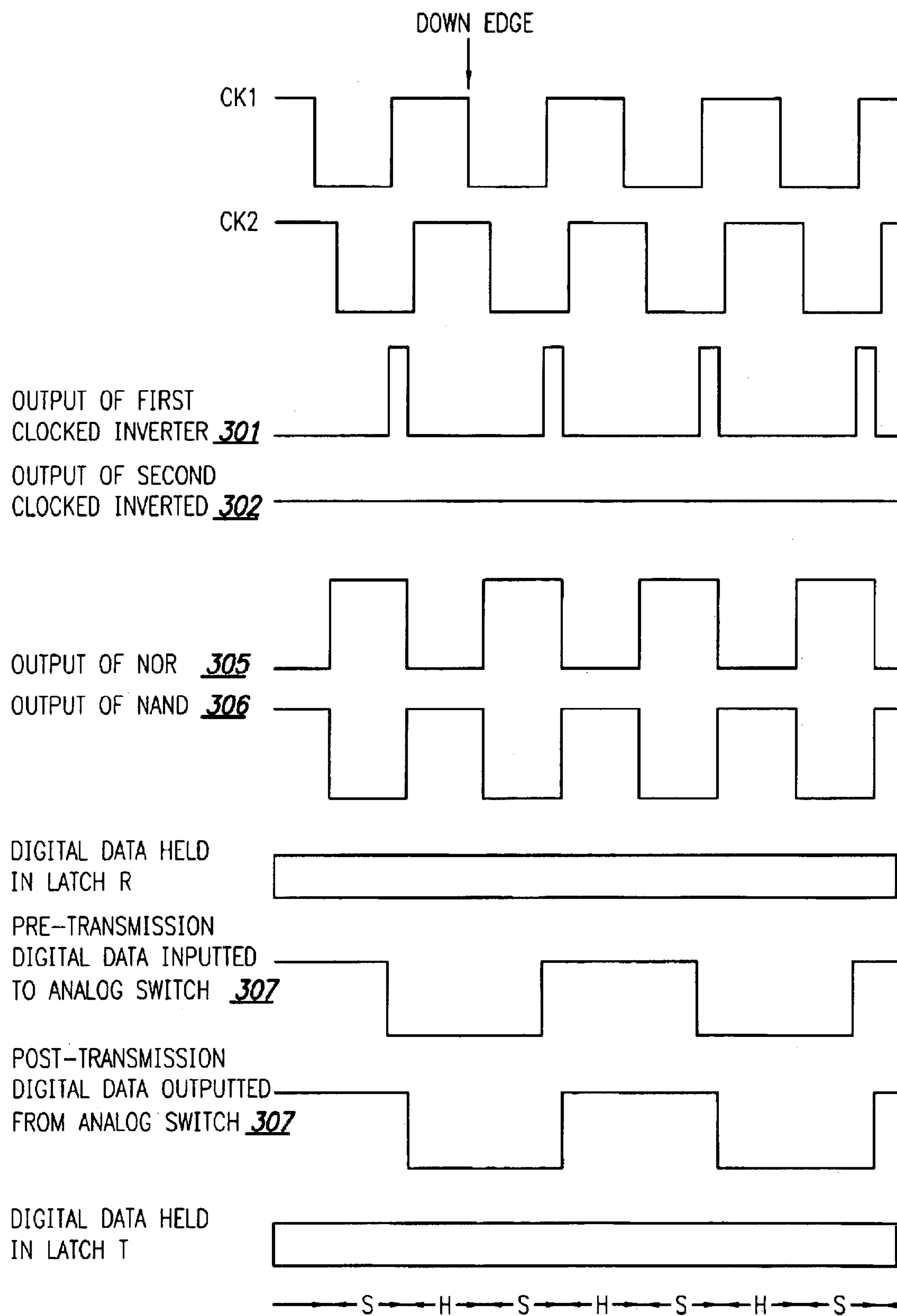
FIG. 6 TIMING CHART FOR CIRCUIT DIAGRAM OF FIG. 4
