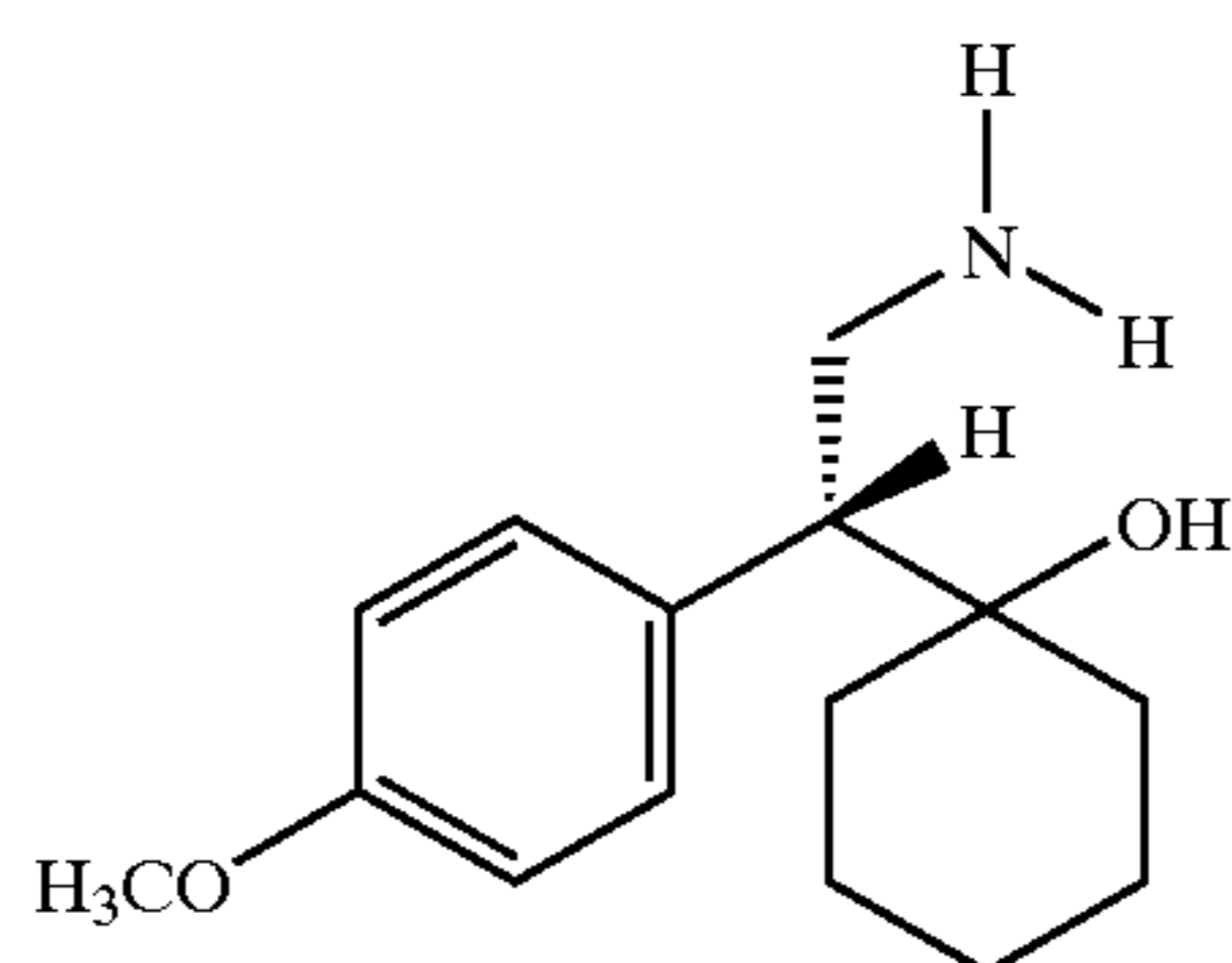
(-)-N,N-didesmethylvenlafaxine
