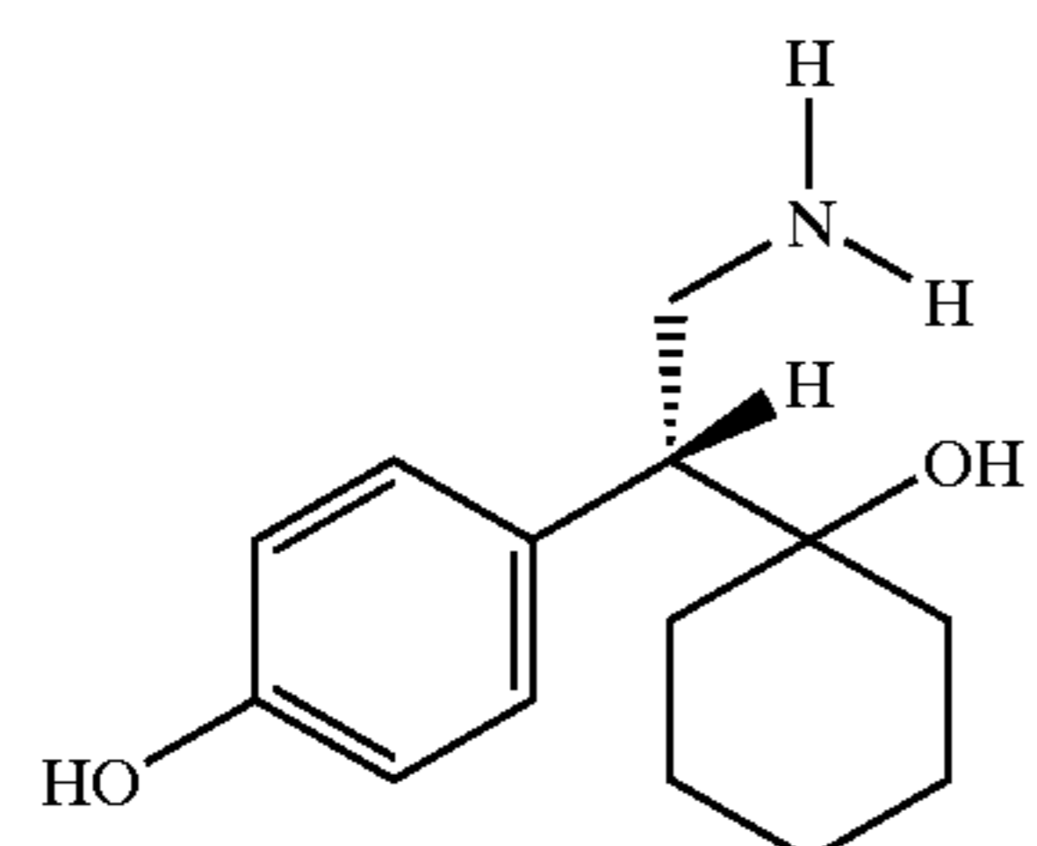
(-)-O-desmethyl-N,N-didesmethylvenlafaxine
