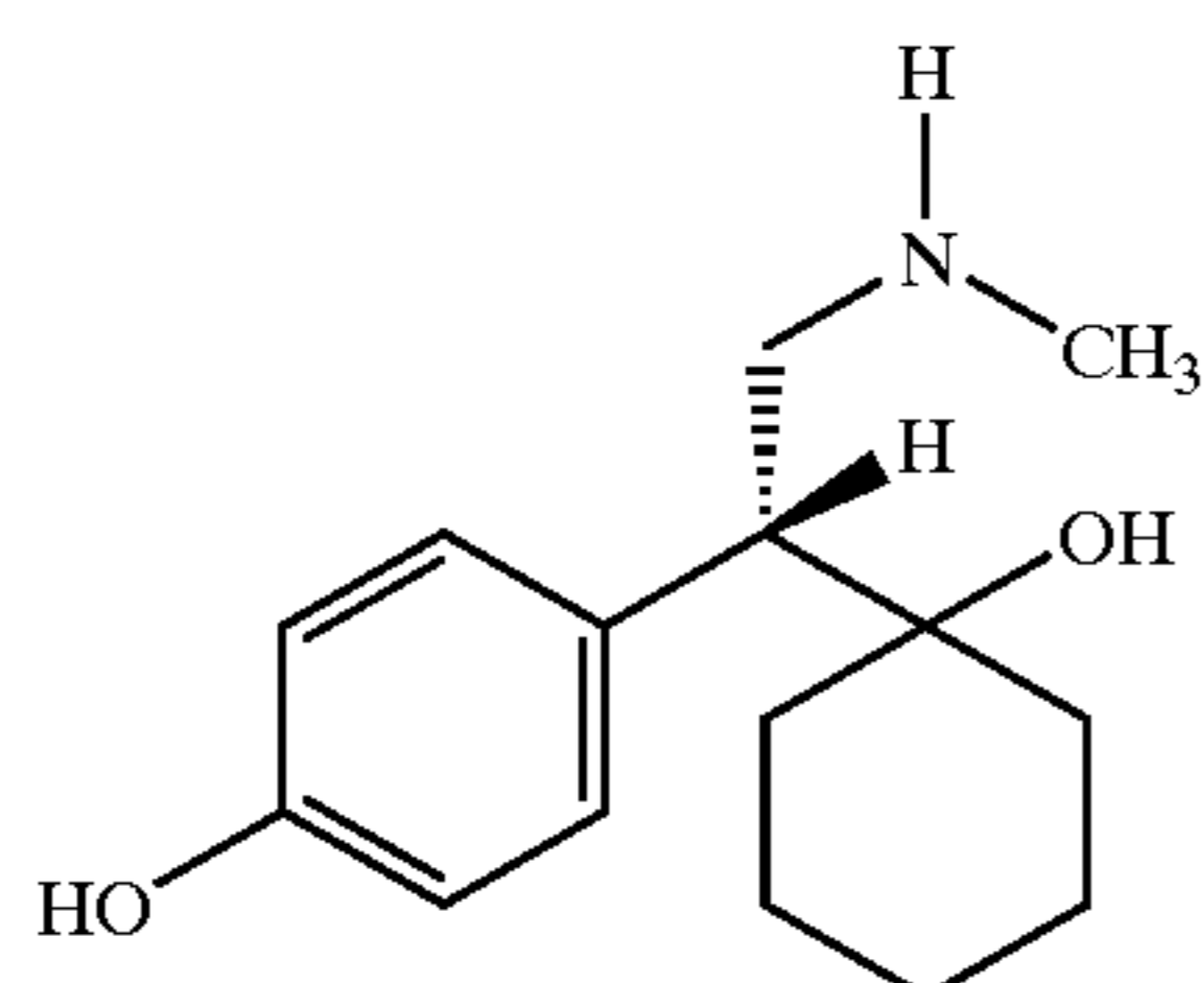
(-)-N,O-didesmethylvenlafaxine
