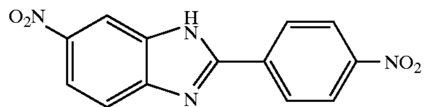
2-(4-nitrophenyl)-5-nitrobenzimidazole
