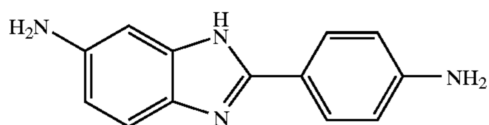
2-(4-aminophenyl)-5-aminobenzimidazole
