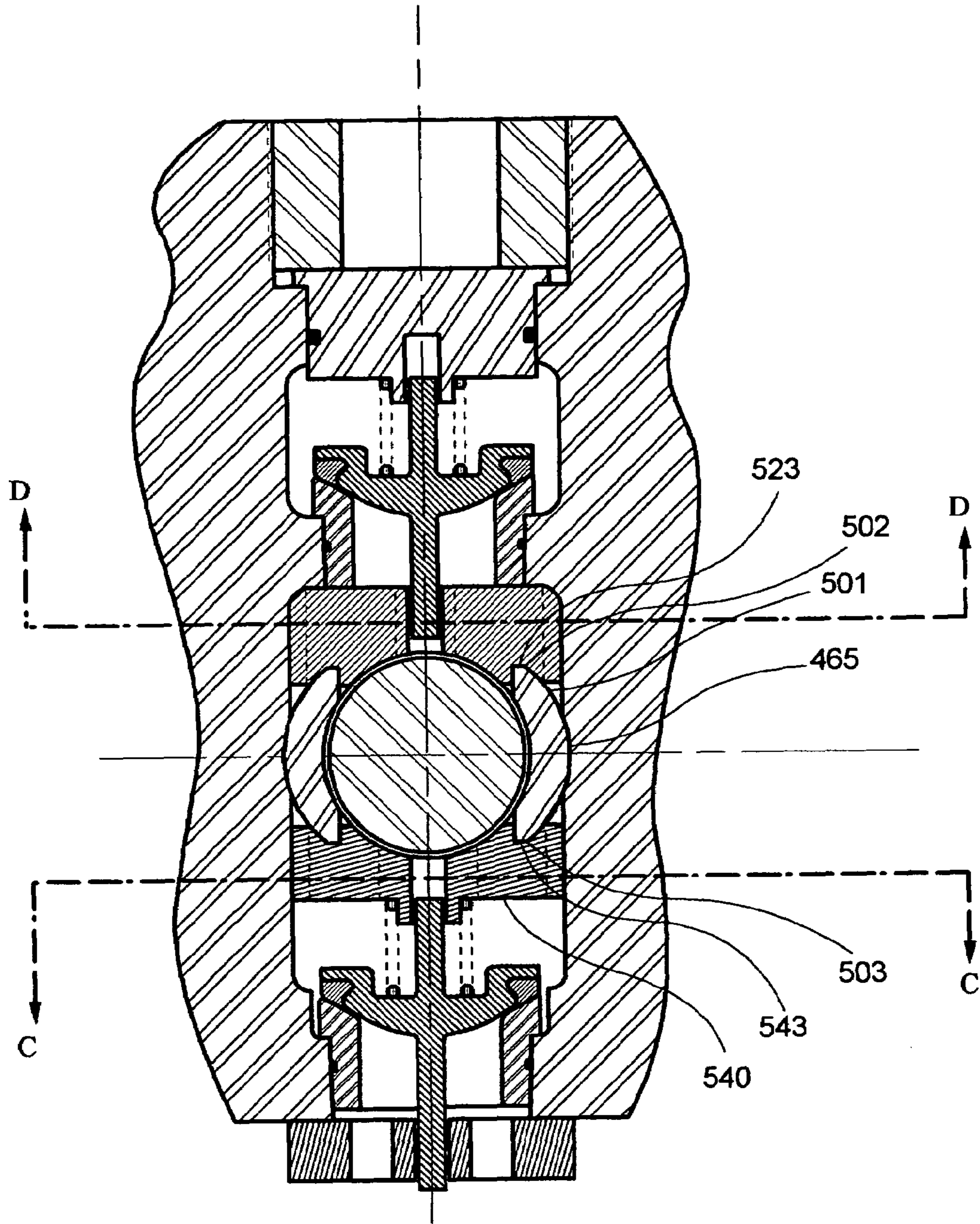
(Section B-B of Figure 10A)
