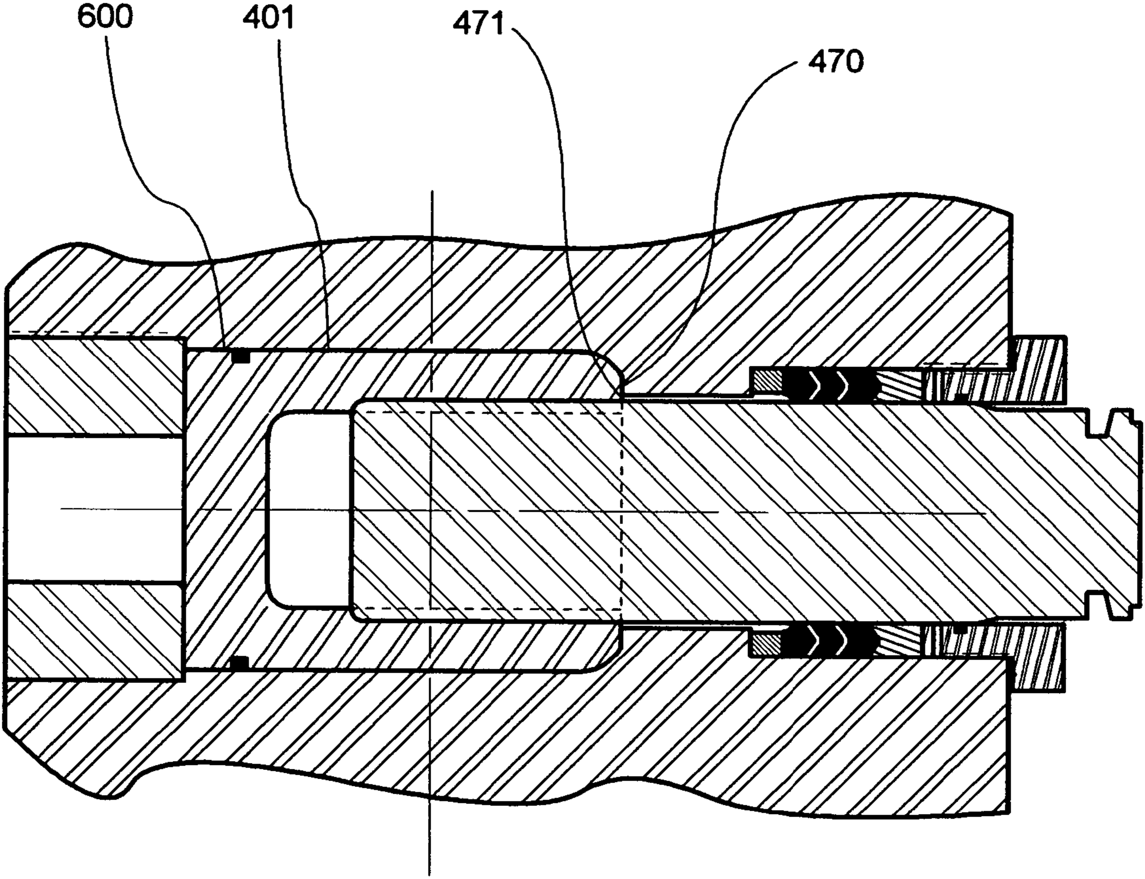
(Section B-B of Figure 9A)
