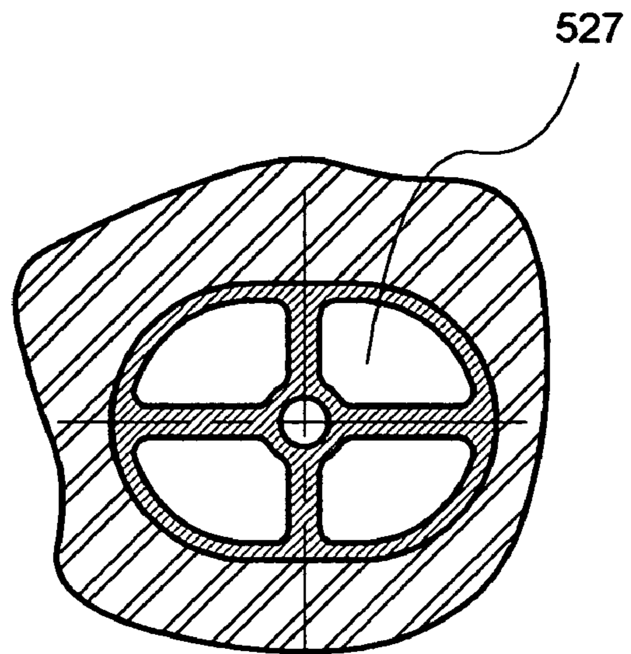
(Section D-D of Figure 10B)
