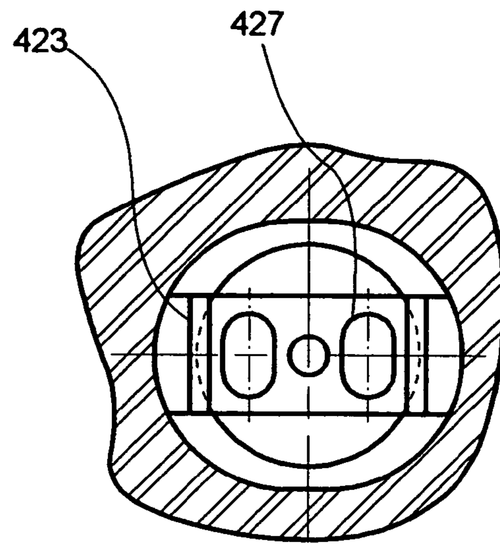
(Section D-D of Figure 8B)
