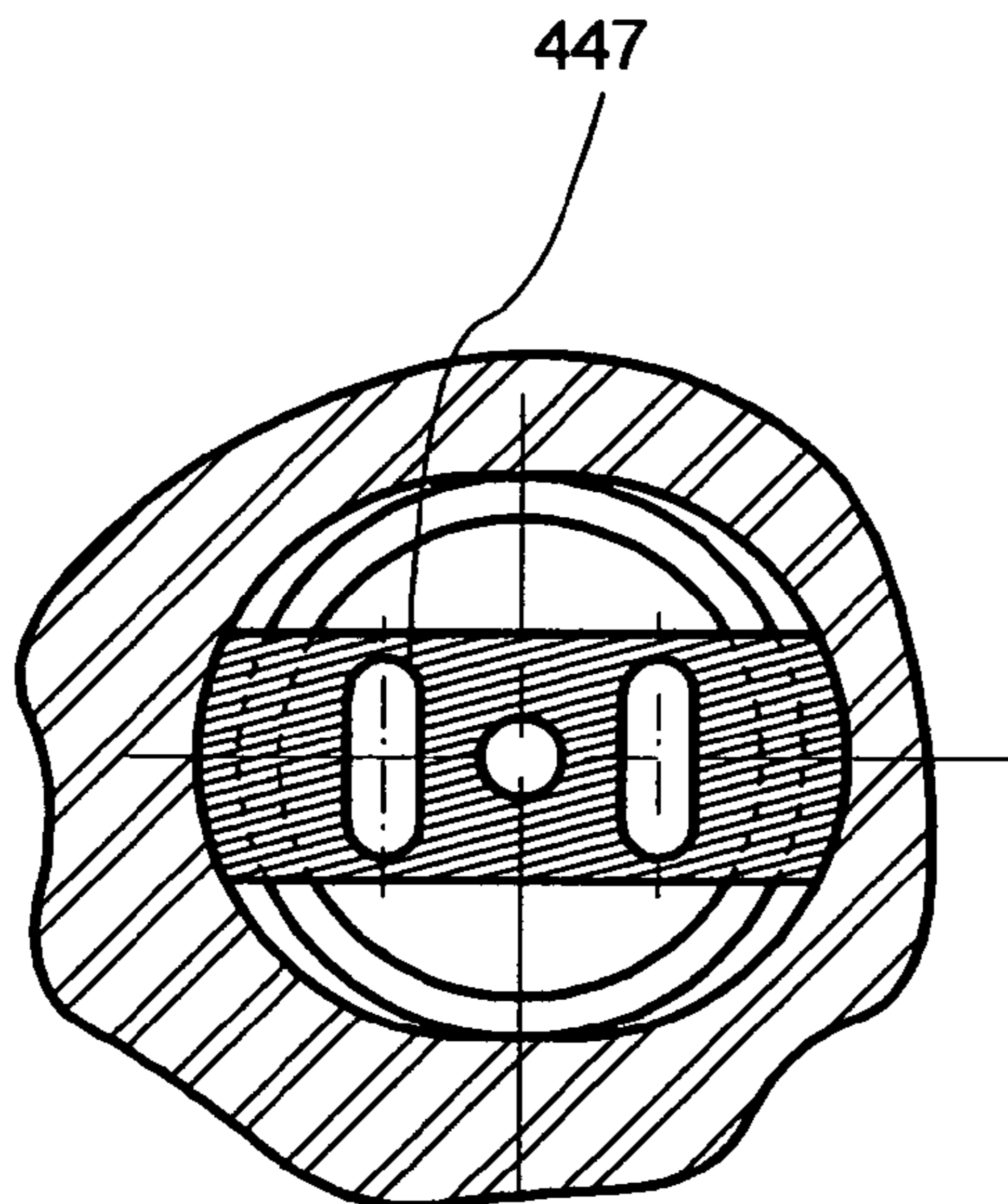
(Section E-E of Figure 8B)
