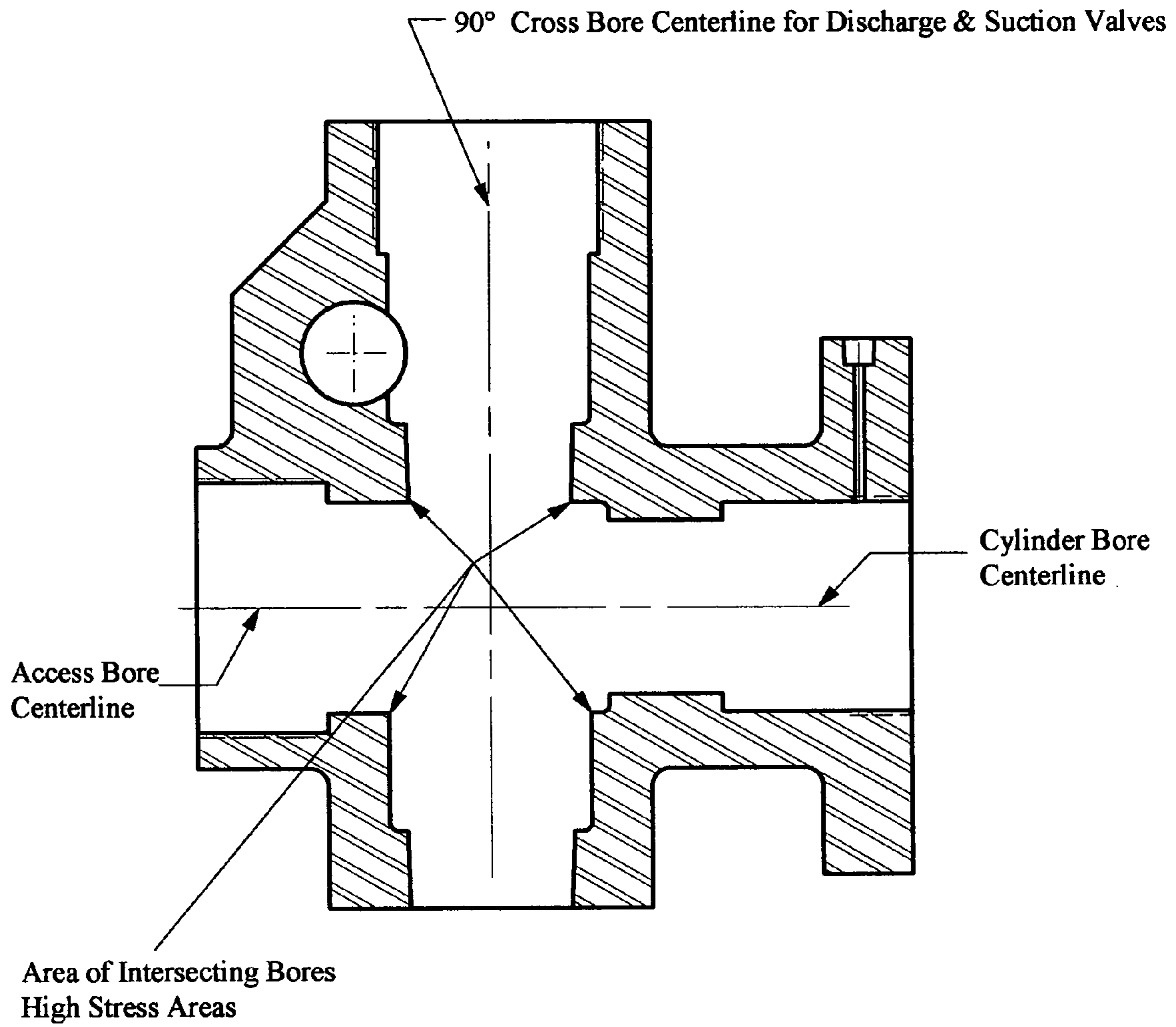
Prior Art Figure 3
