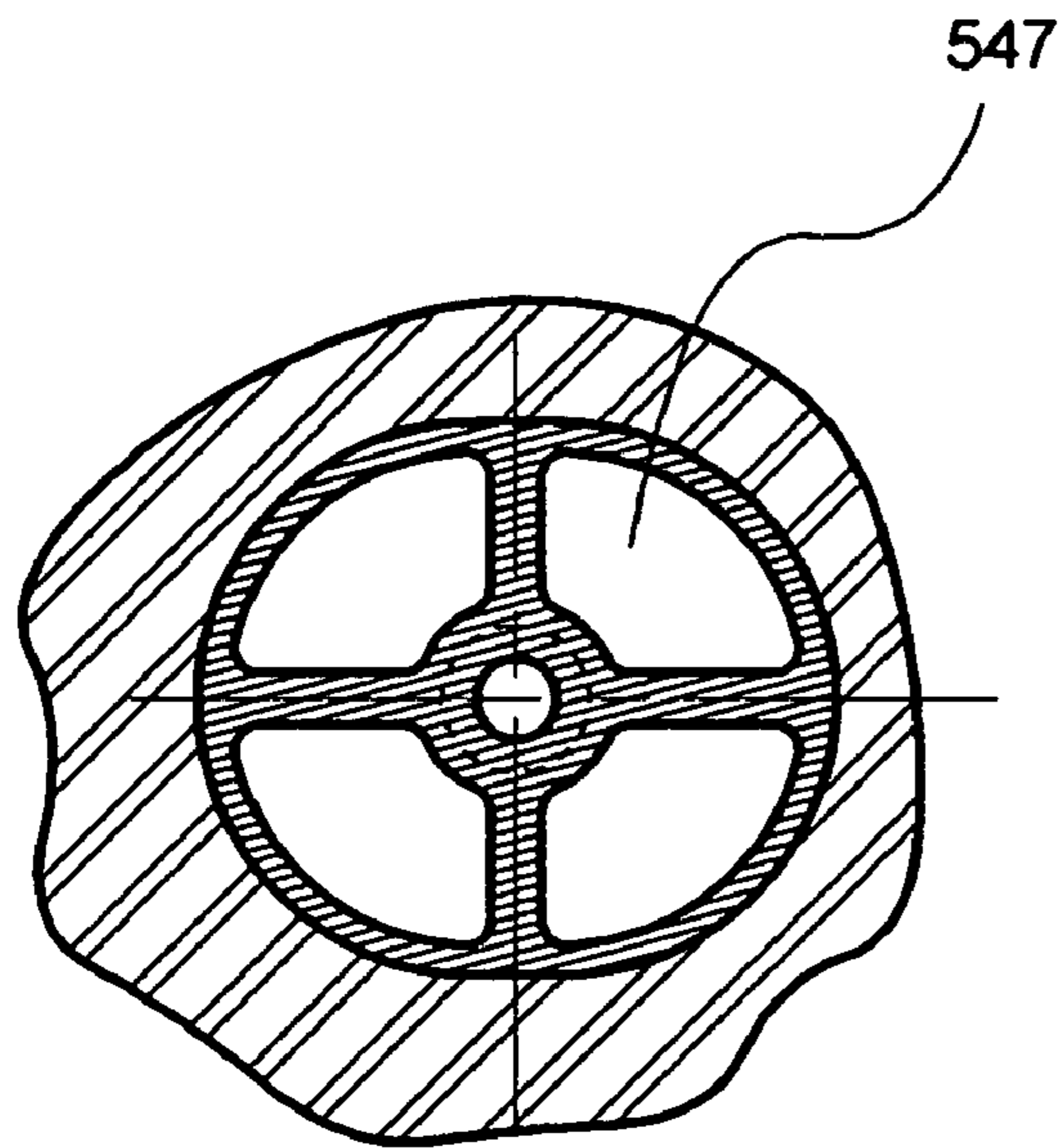
(Section C-C of Figure 10B)
