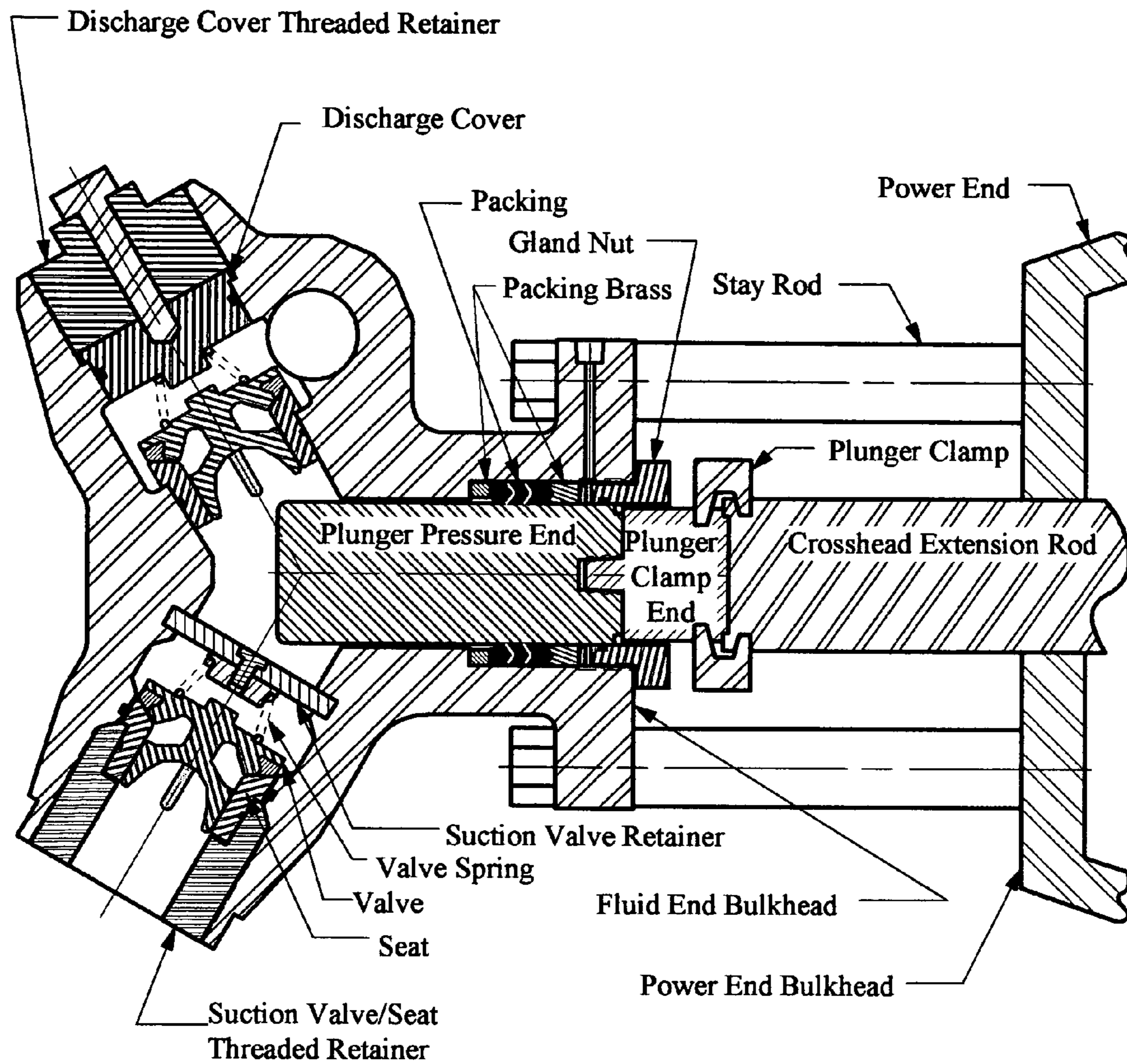
Prior Art Figure 5
