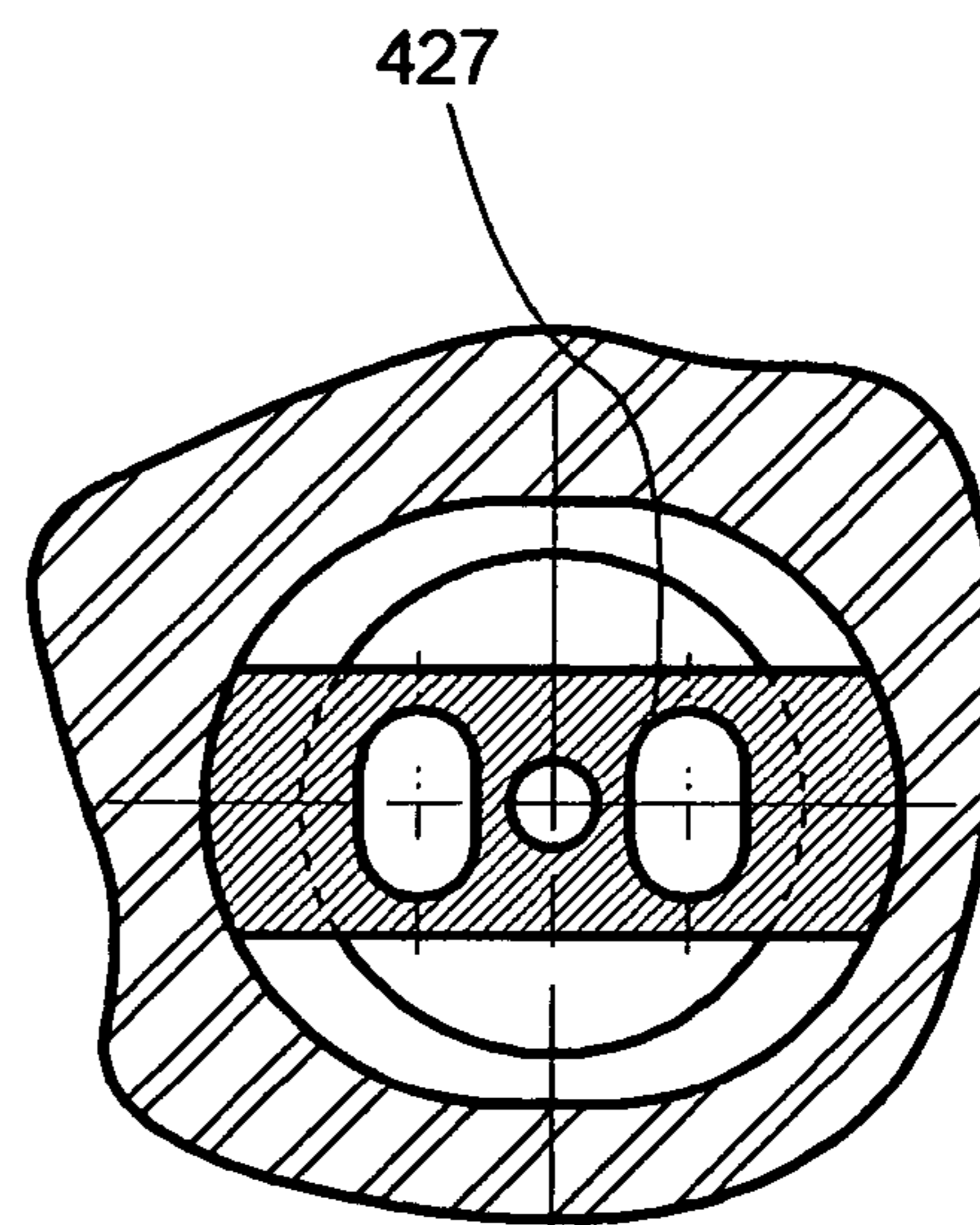
(Section F-F of Figure 8B)
