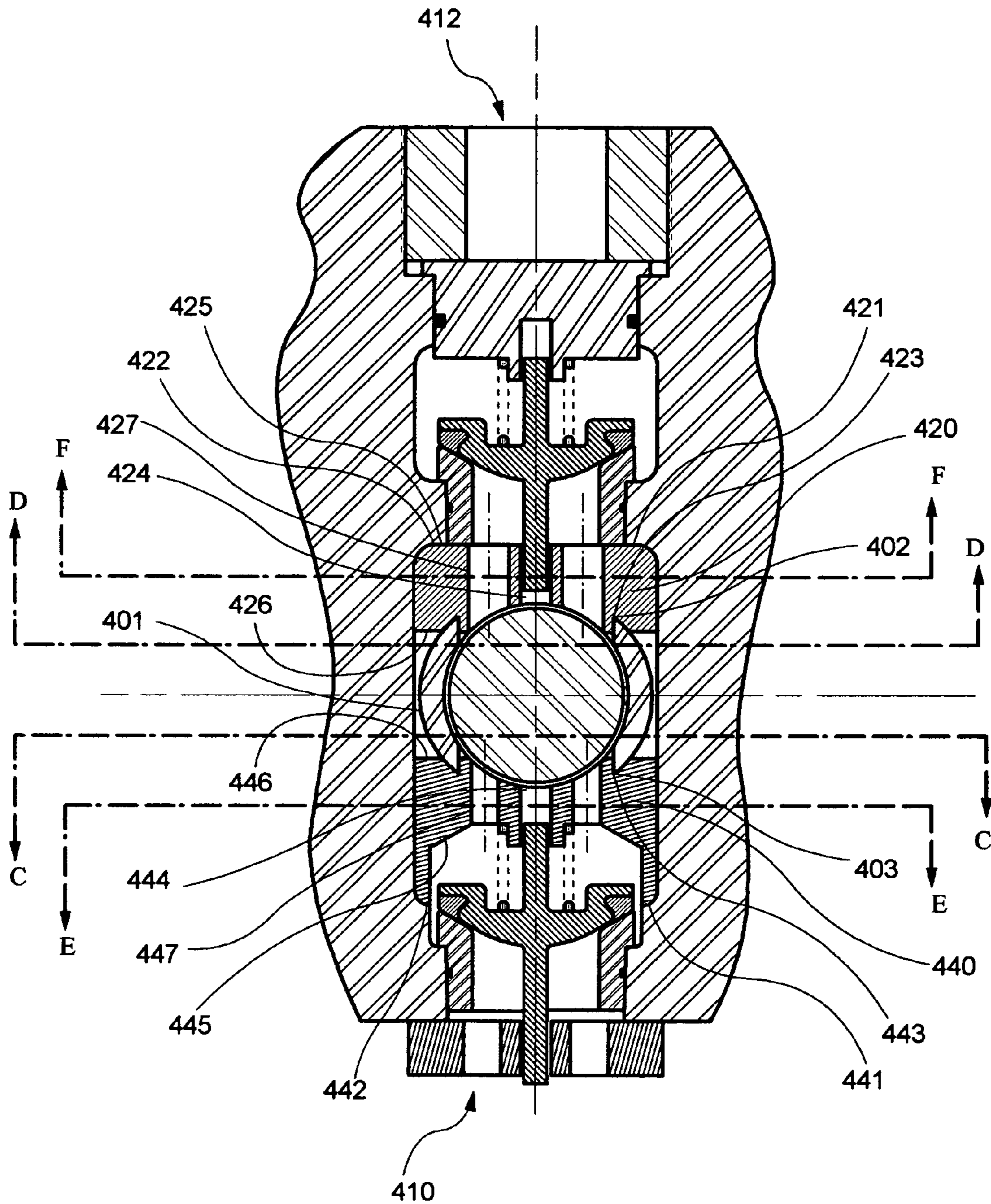
(Section B-B of Figure 8A
