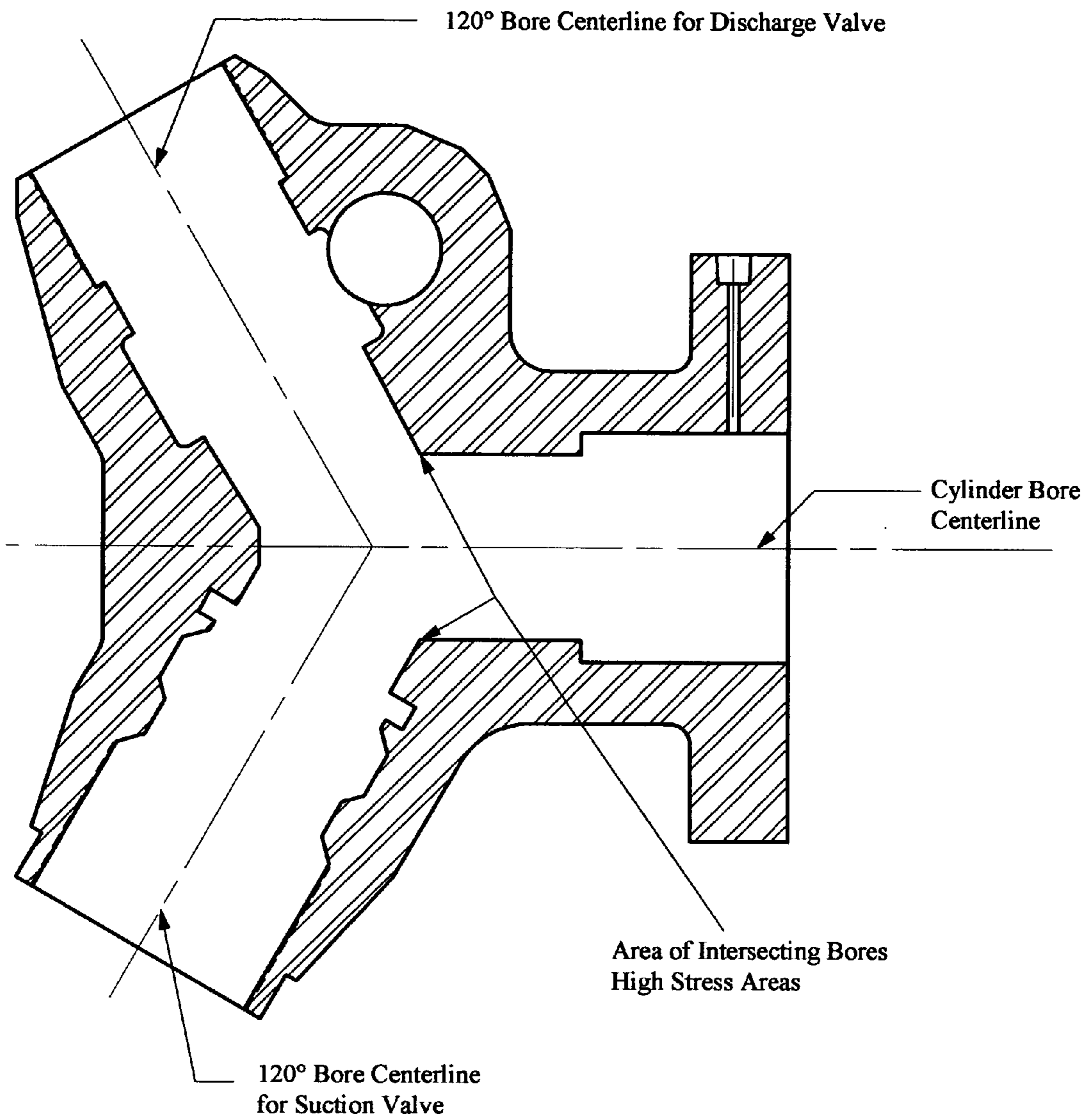
Prior Art Figure 4
