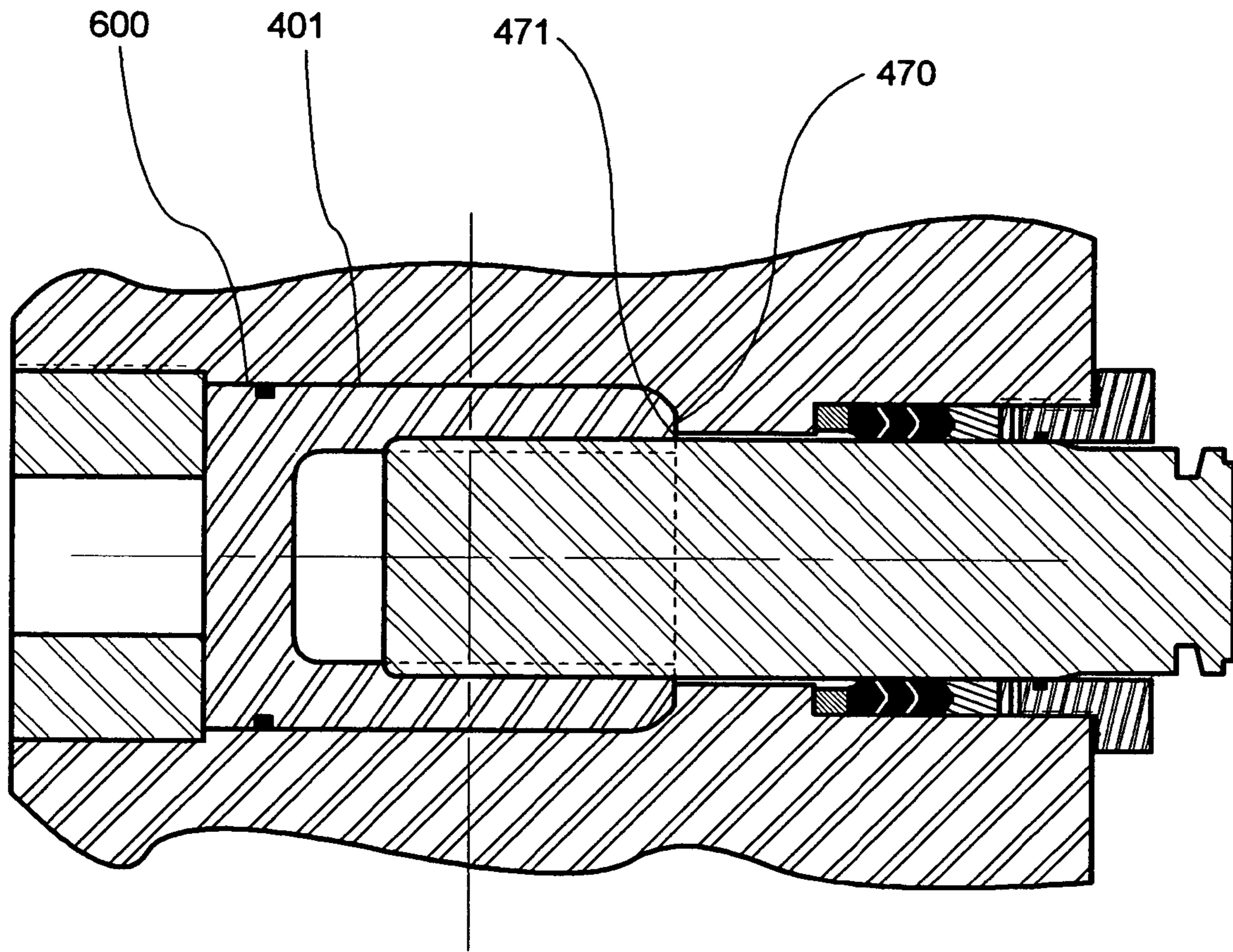
(Section B-B of Figure 9A)
