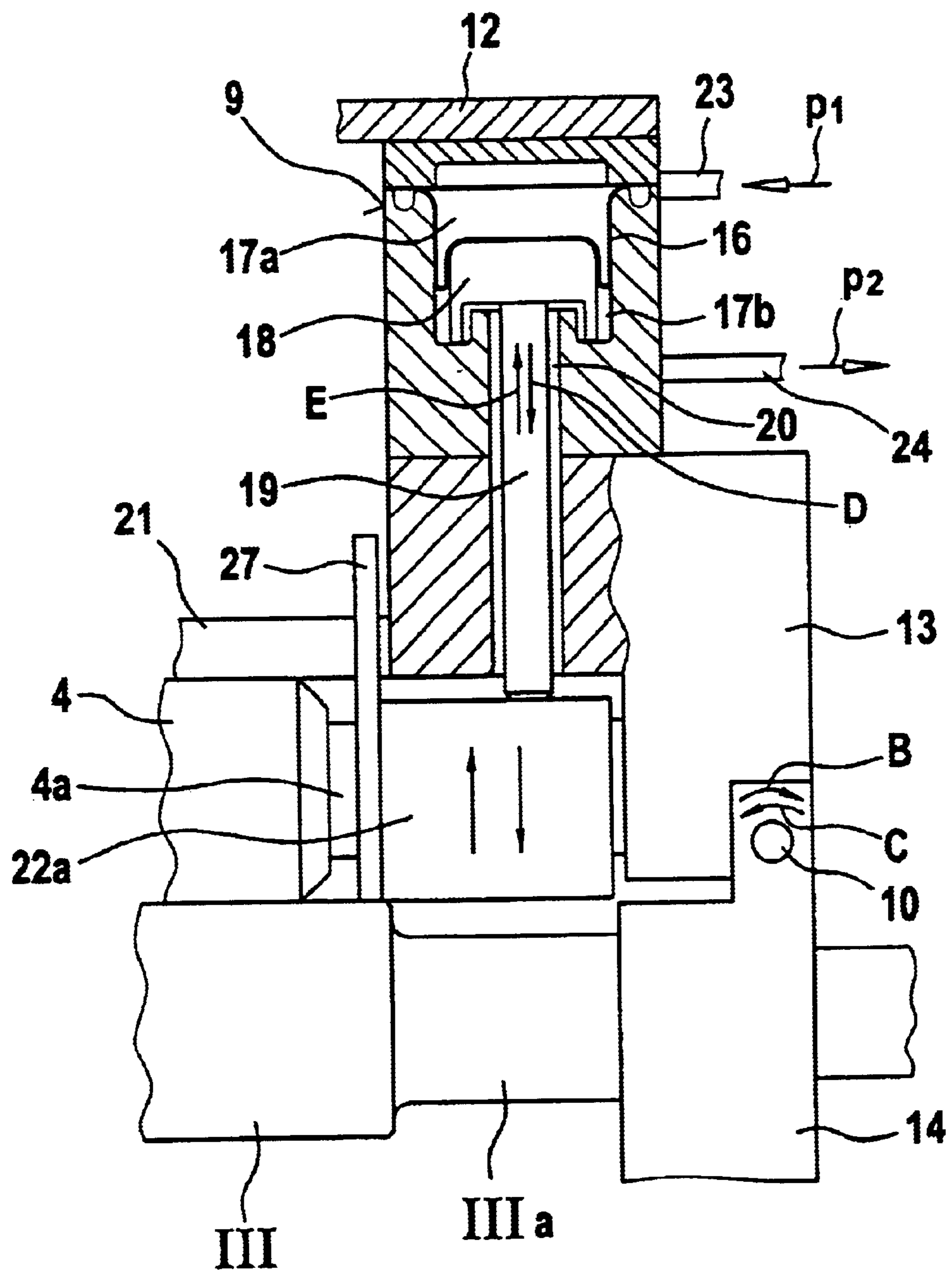
Fig. 2 Section K-K
