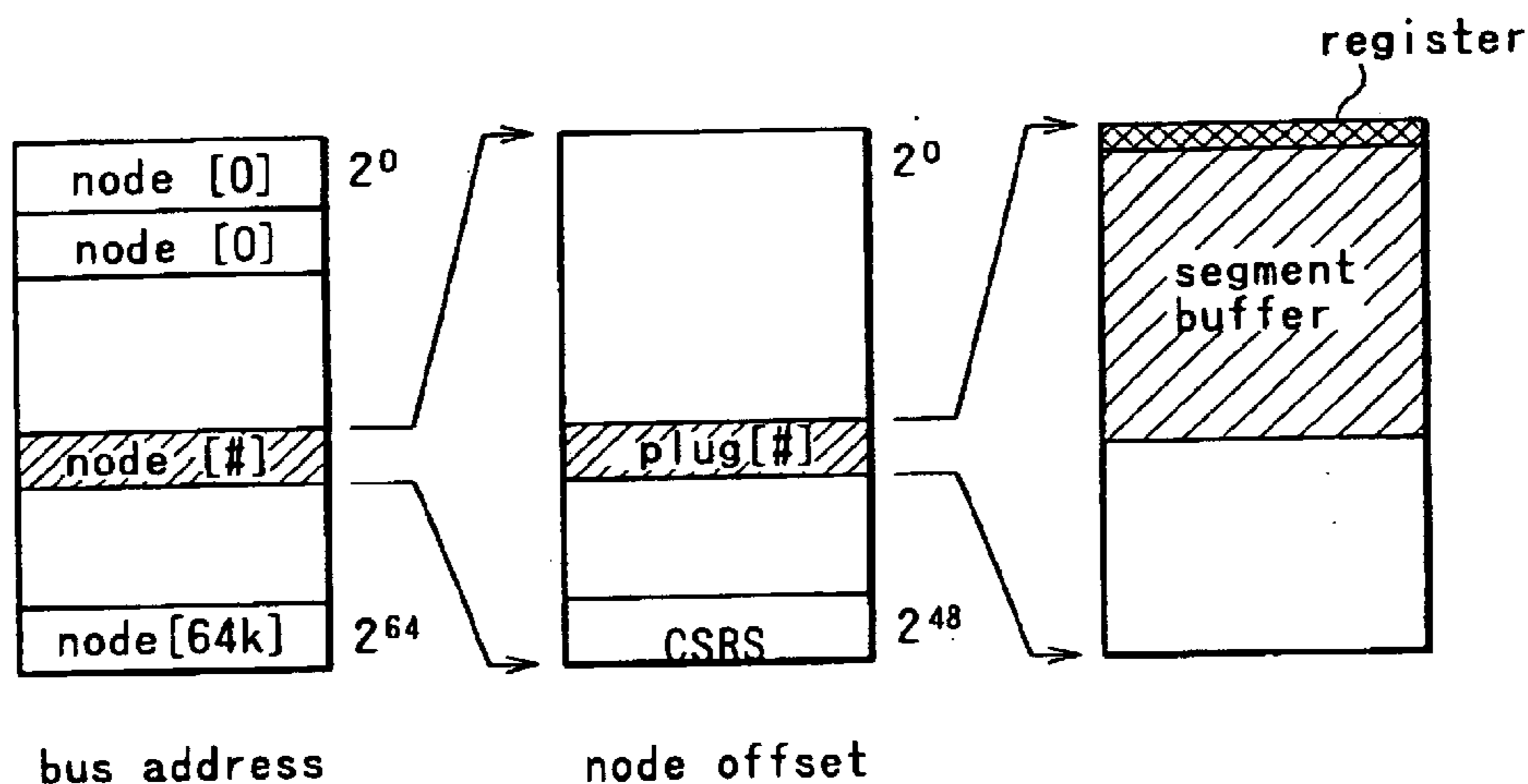
Location of plug address spaces
