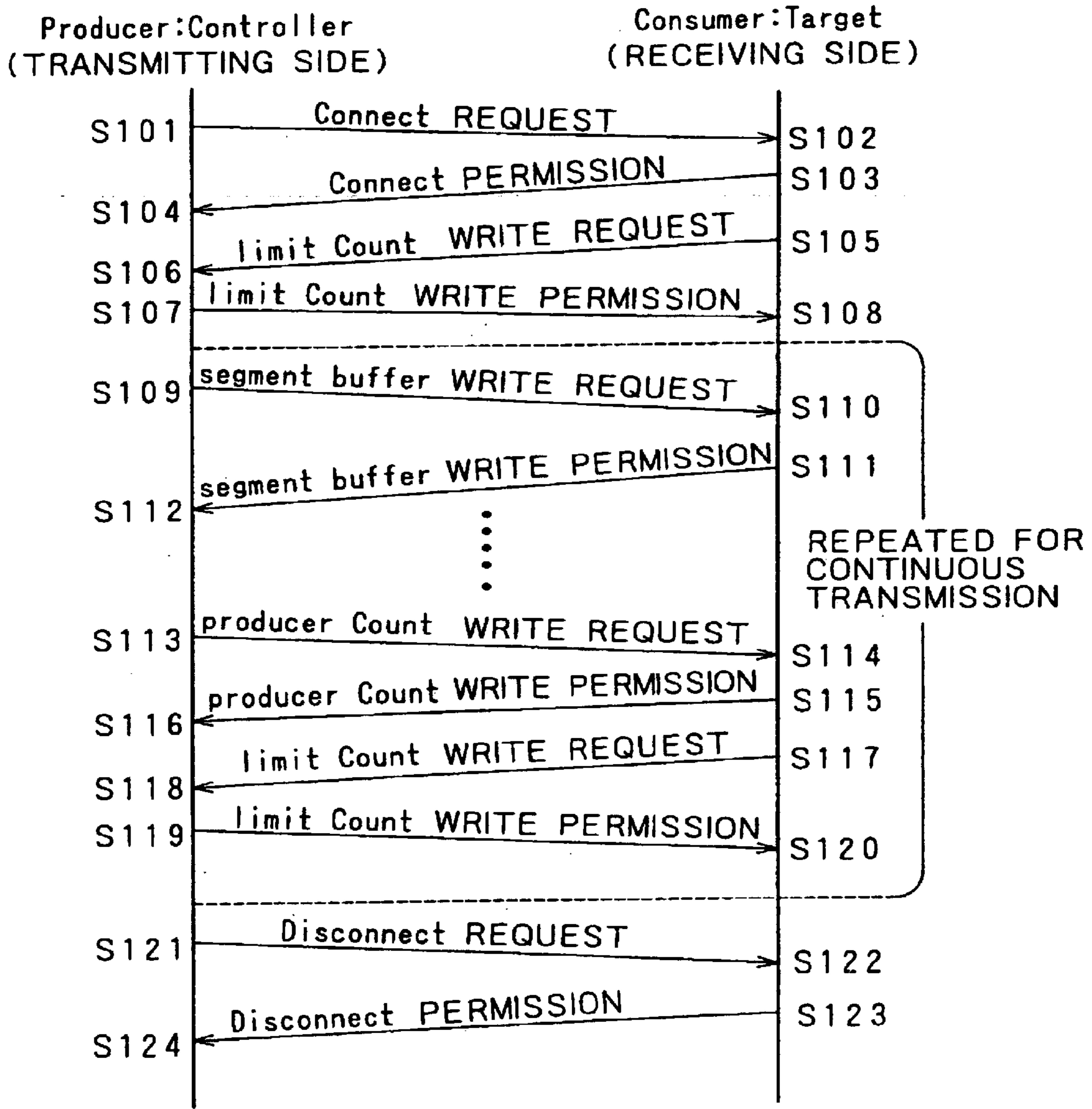
PROCEDURES FOR Asynchronous Connection TRANSMISSION AND RECEPTION
