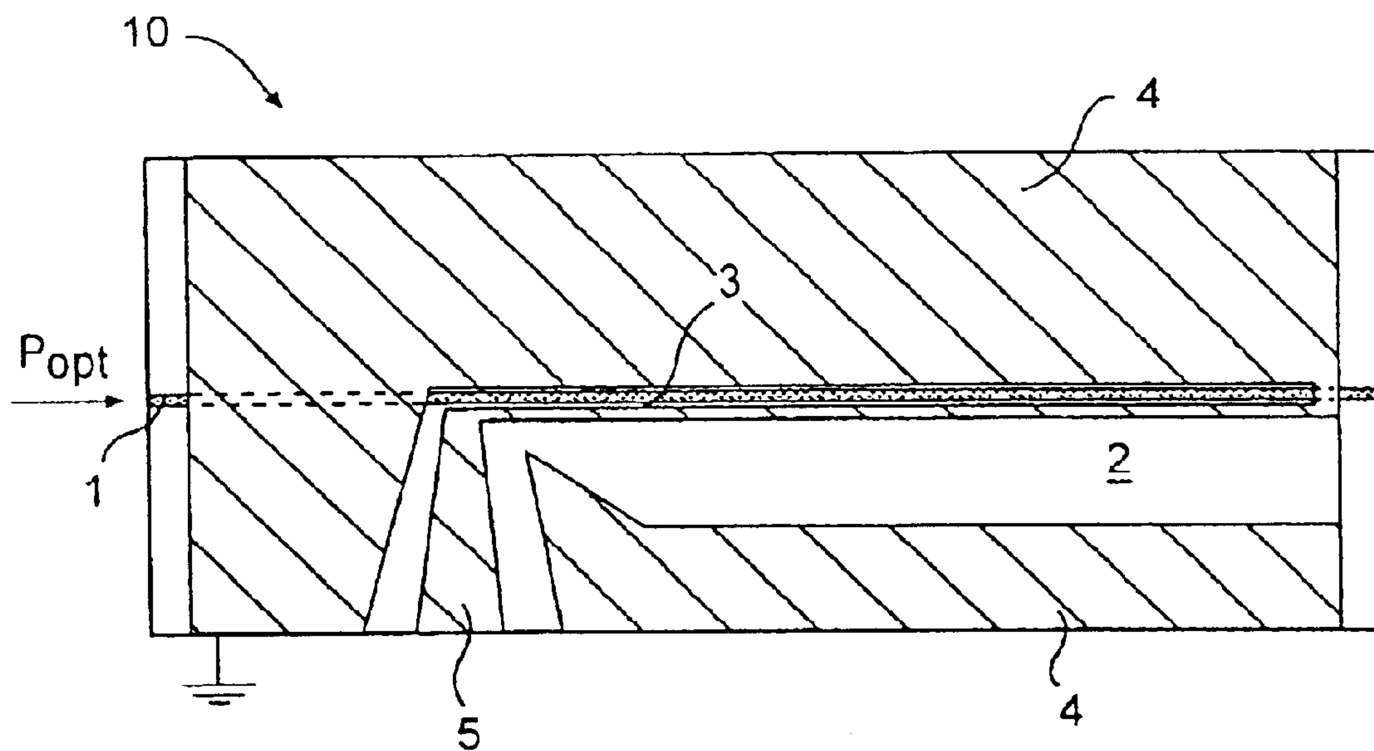
FIG. 3 (PRIOR ART)
