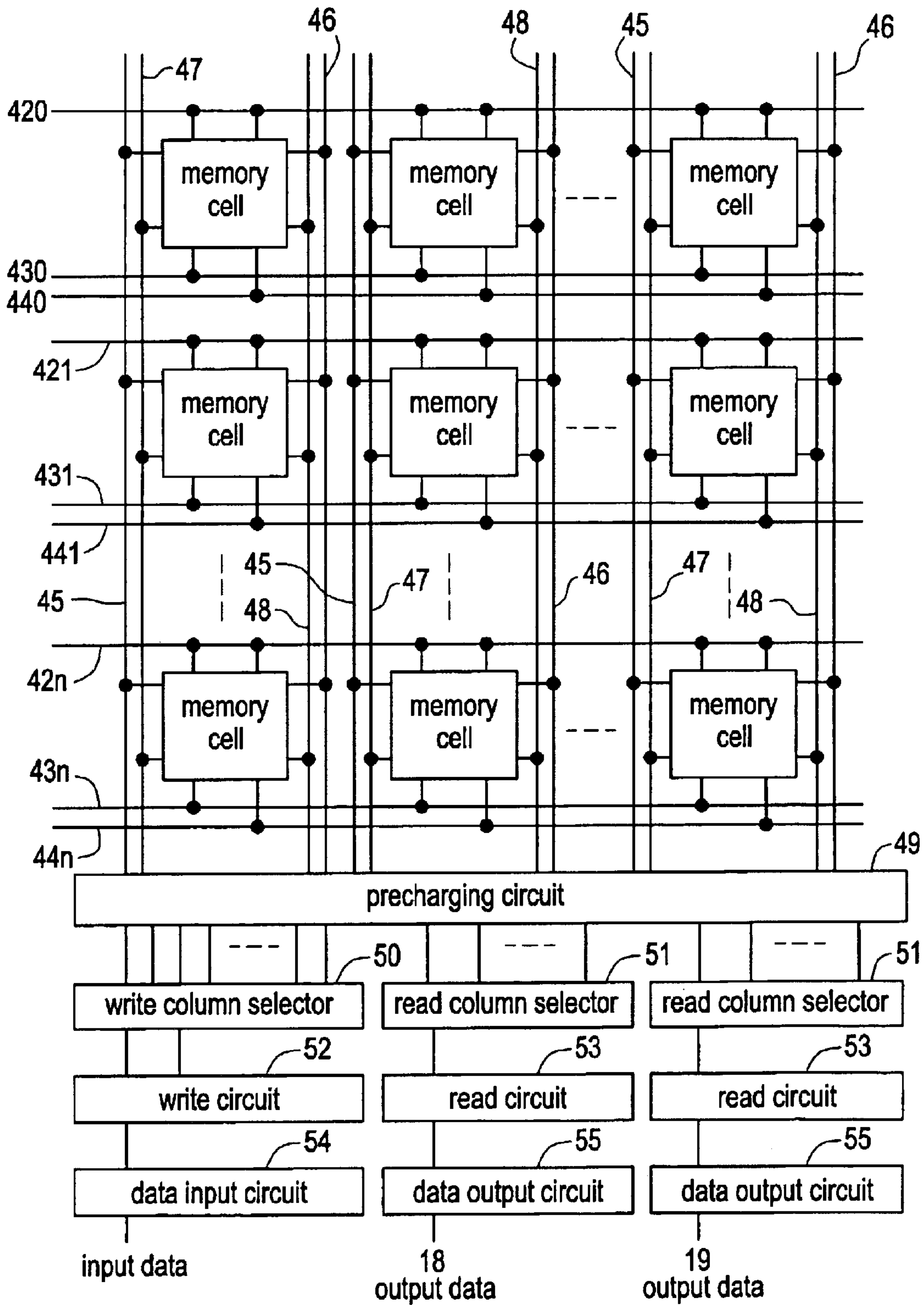
FIG. 2 PRIOR ART
