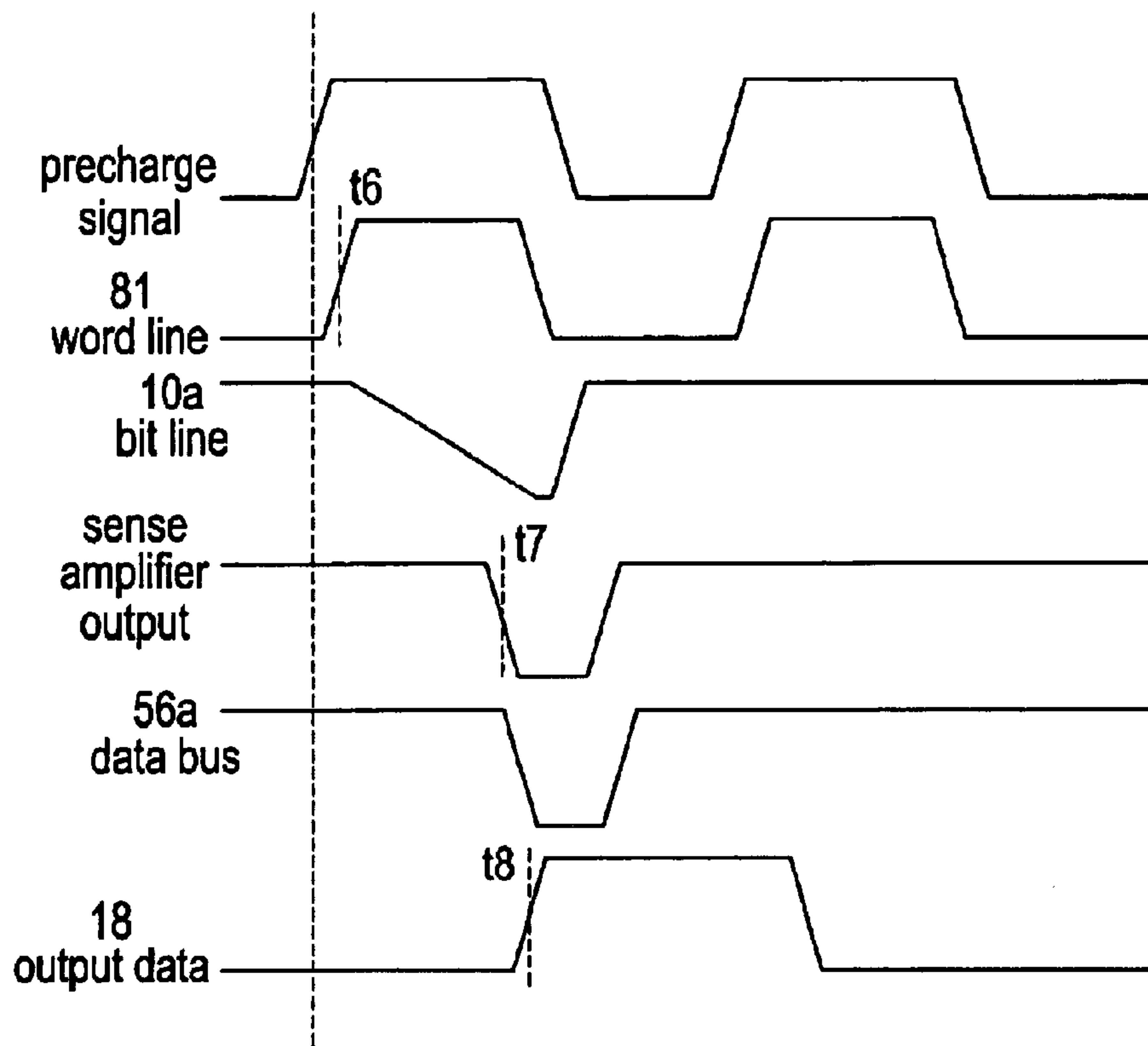
FIG. 7 PRIOR ART
