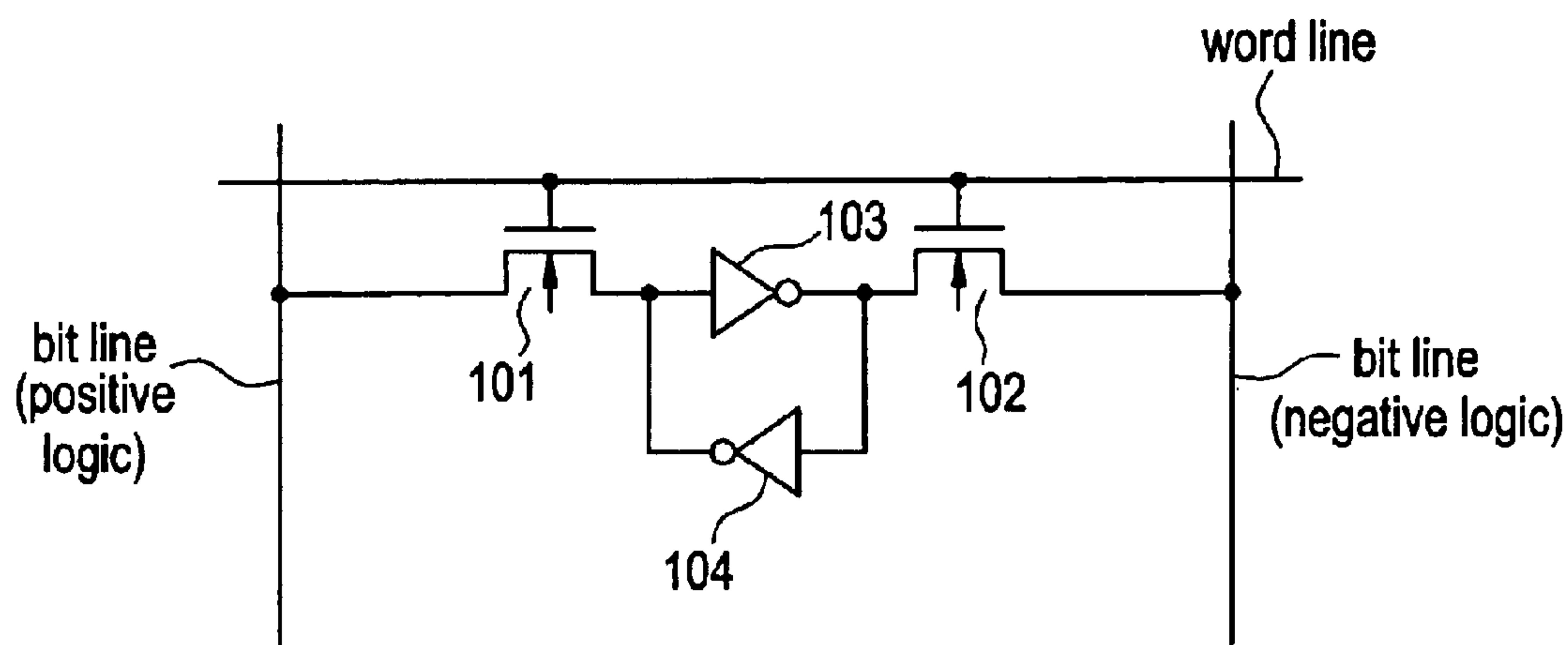
FIG. 7 PRIOR ART
